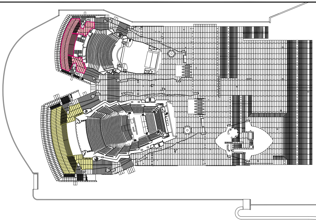
LEVEL 4 - SSDA (SSD 7549) Drawing : 10 BG 20904 S11 RevG
