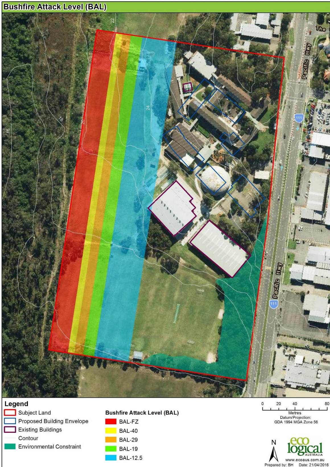
Figure 4: Bushfire Attack Level (BAL) plan
