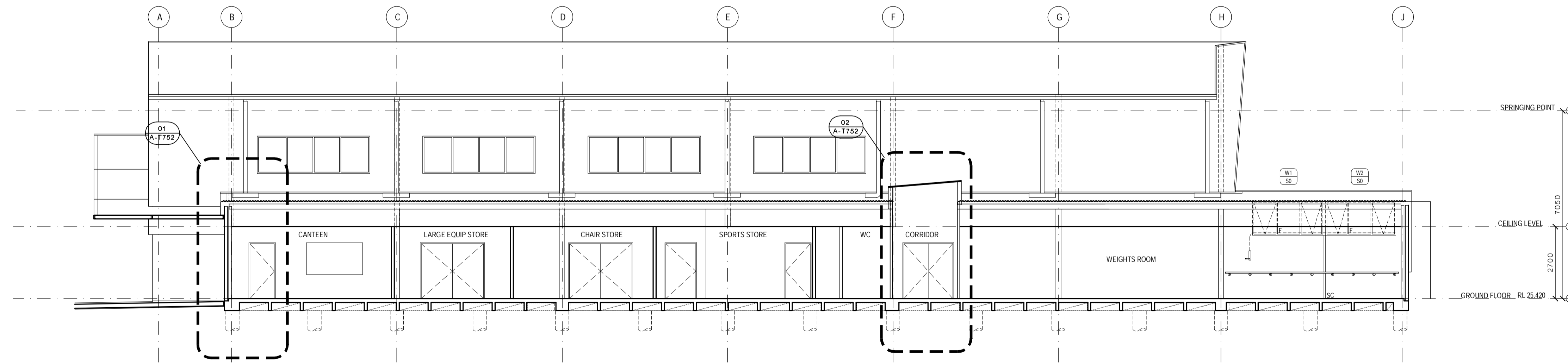
02 SECTION A701 SCALE 1:100
