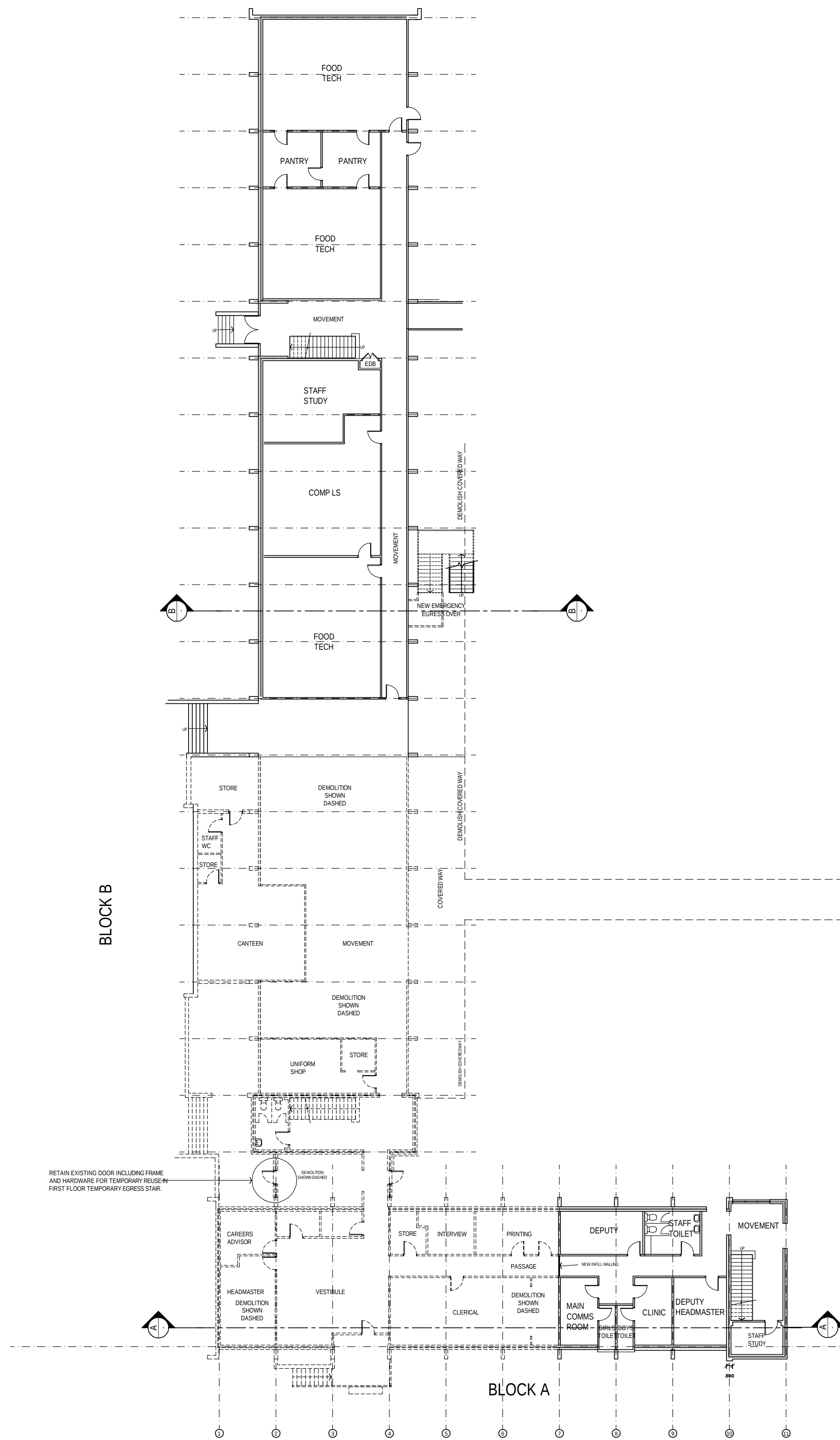
GROUND FLOOR Scale 1:200
