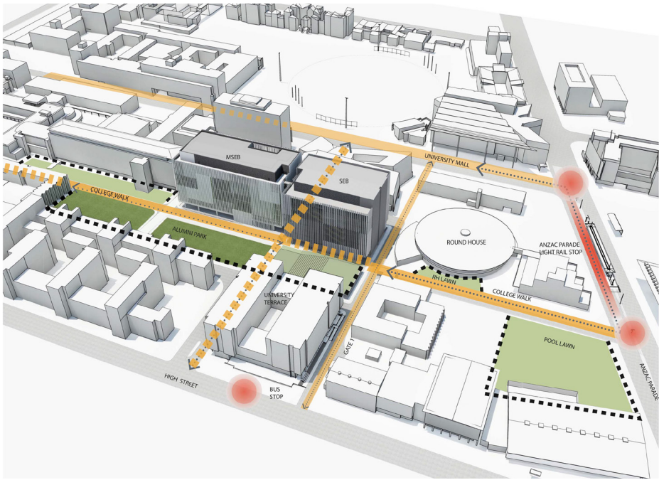
SITE ANALYSIS PROPOSED
