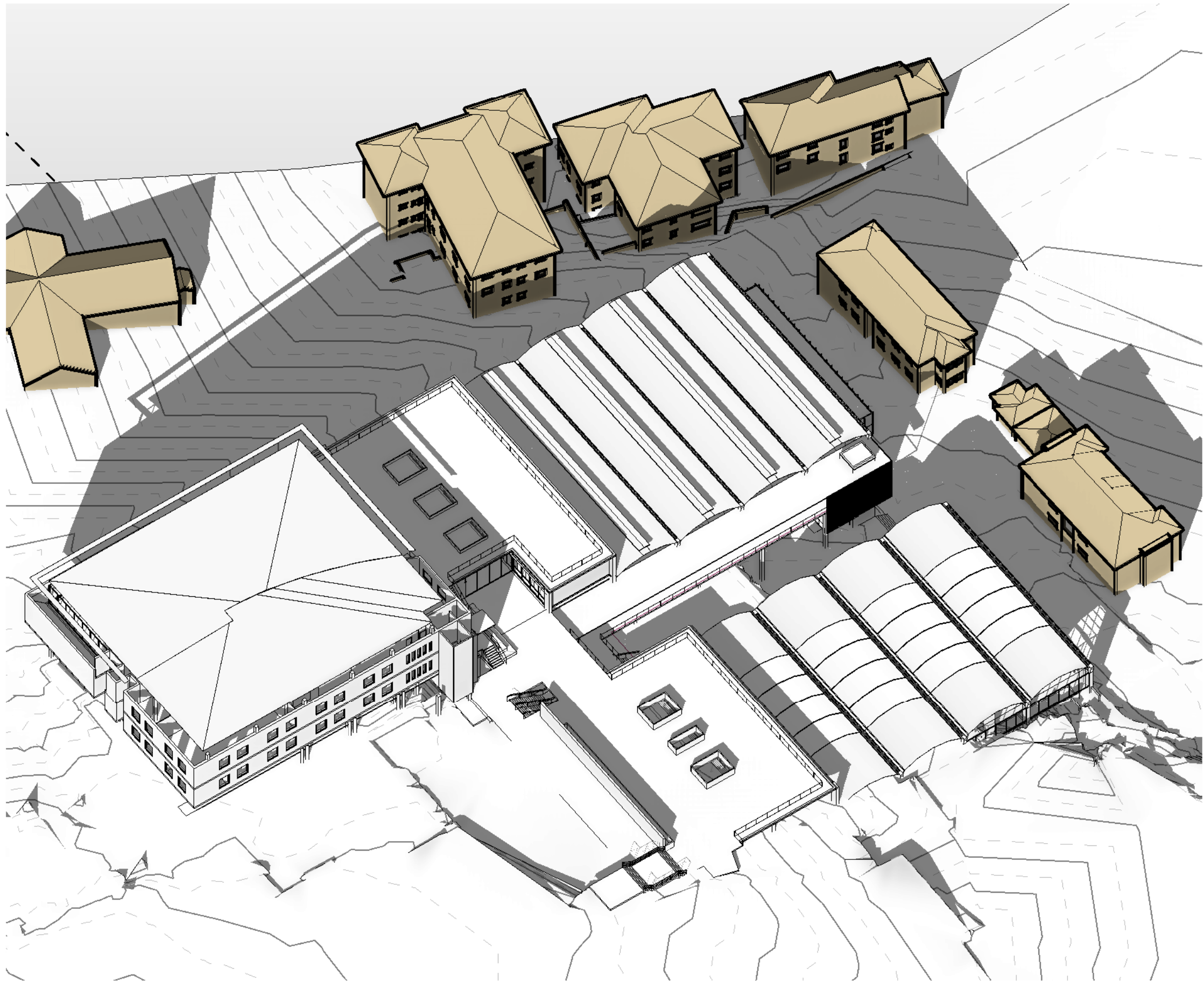
2 3D VIEW - 21 JUNE - 2:00 PM - SHADOW CAST BY PROPOSED BUILDINGS SCALE
