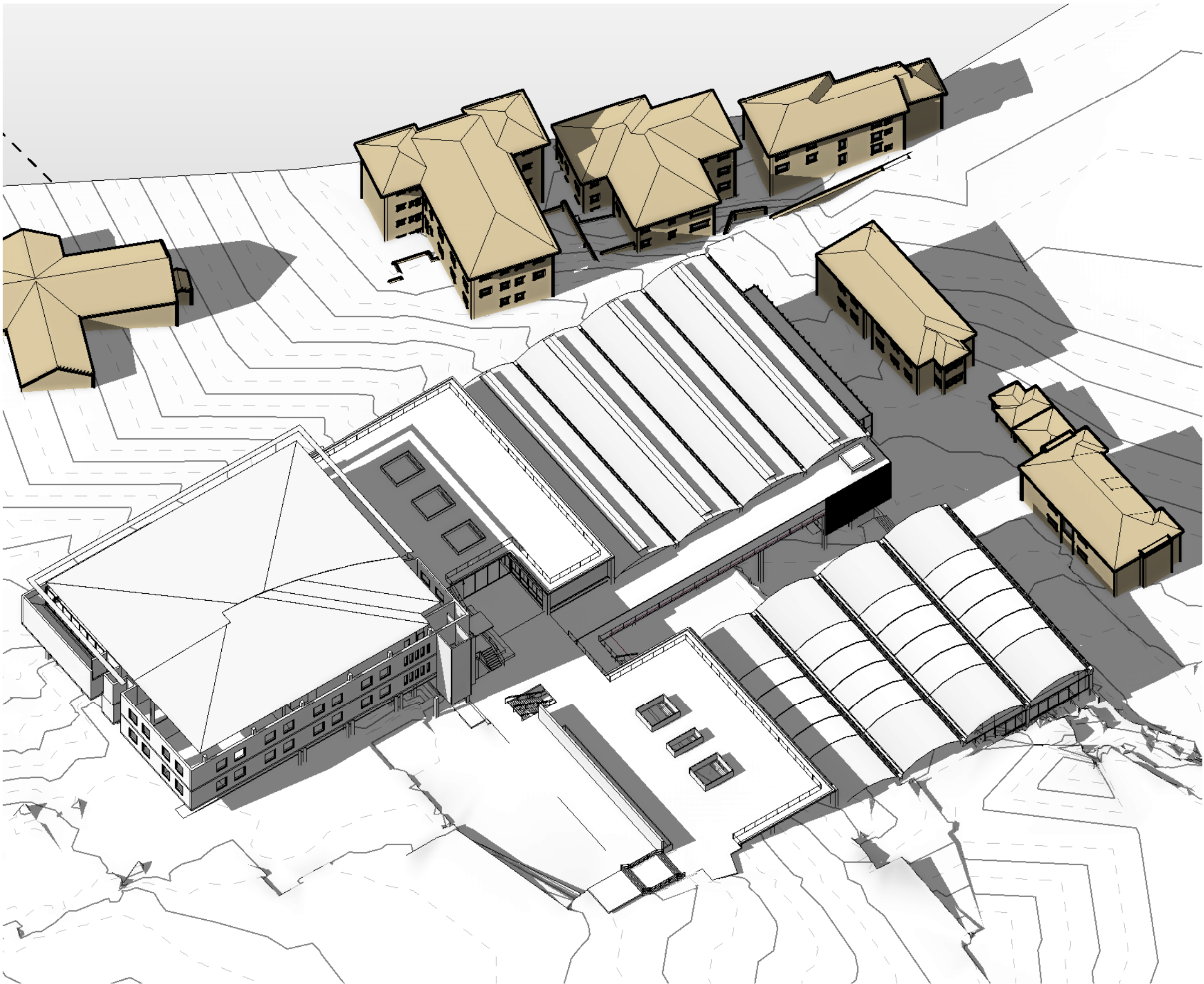
2 3D VIEW - 21 JUNE - 11:00 AM - SHADOW CAST BY PROPOSED BUILDINGS SCALE
