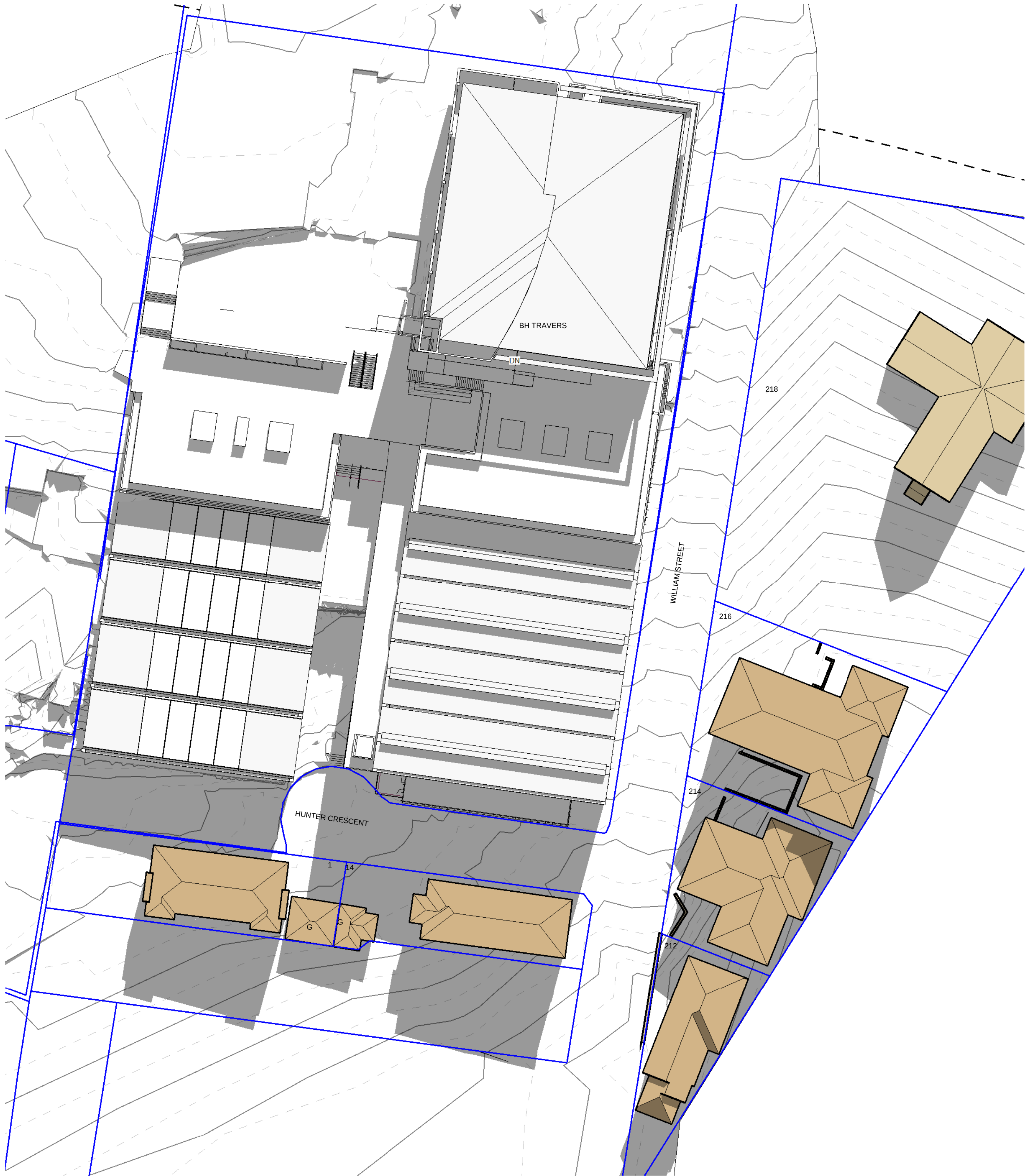
1 PLAN - 21 JUNE - 11:00 AM - SHADOW CAST BY PROPOSED BUILDINGS SCALE 1 : 400
