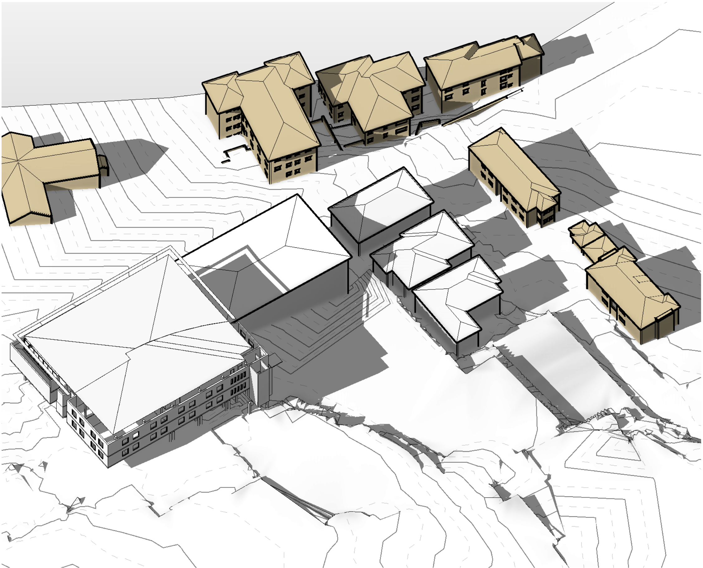
2 3D VIEW - 21 JUNE - 11:00 AM - SHADOW CAST BY EXISTING BUILDINGS SCALE
