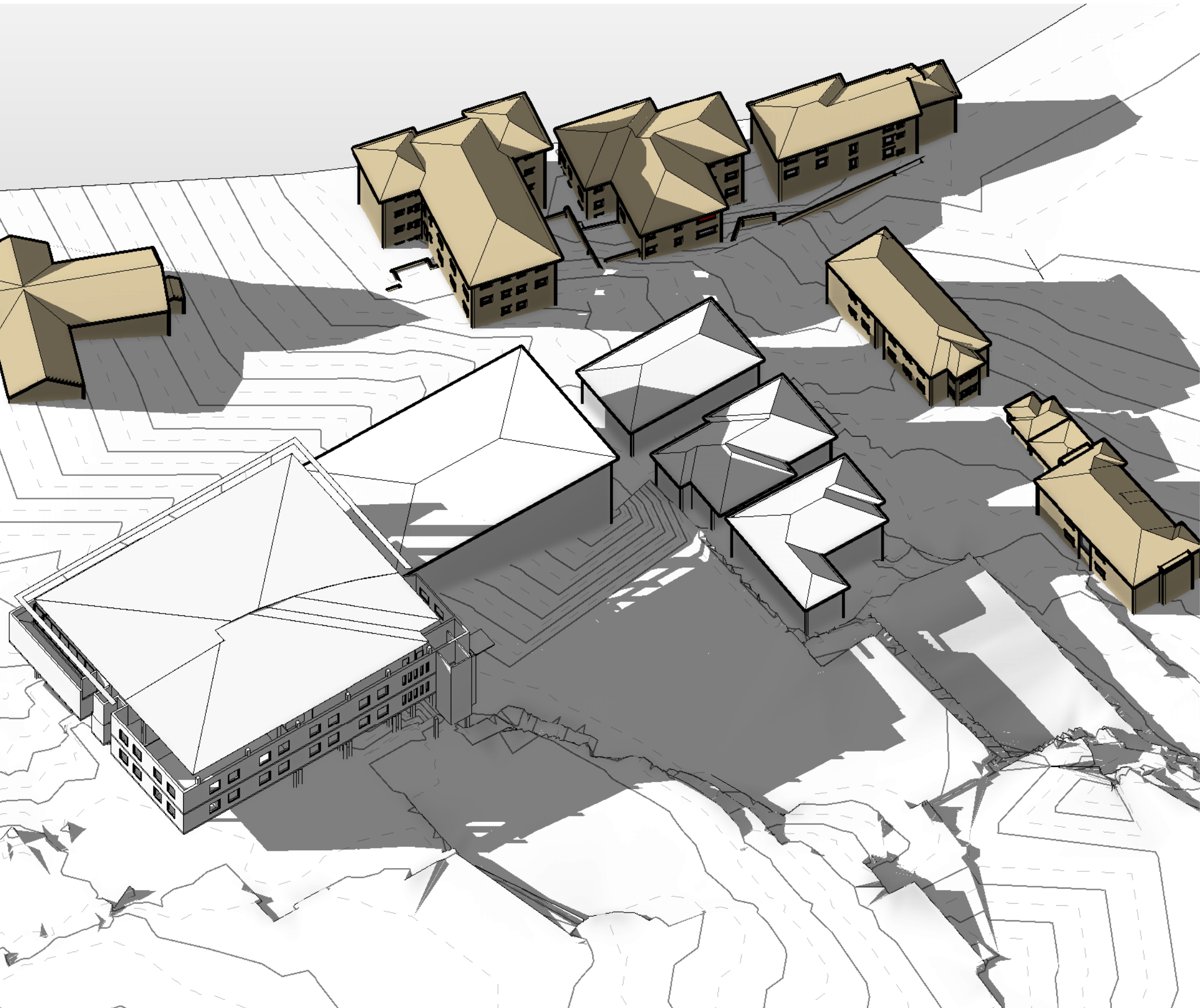
2 3D VIEW- 21 JUNE - 9:00 AM - SHADOW CAST BY EXISTING BUILDINGS SCALE
