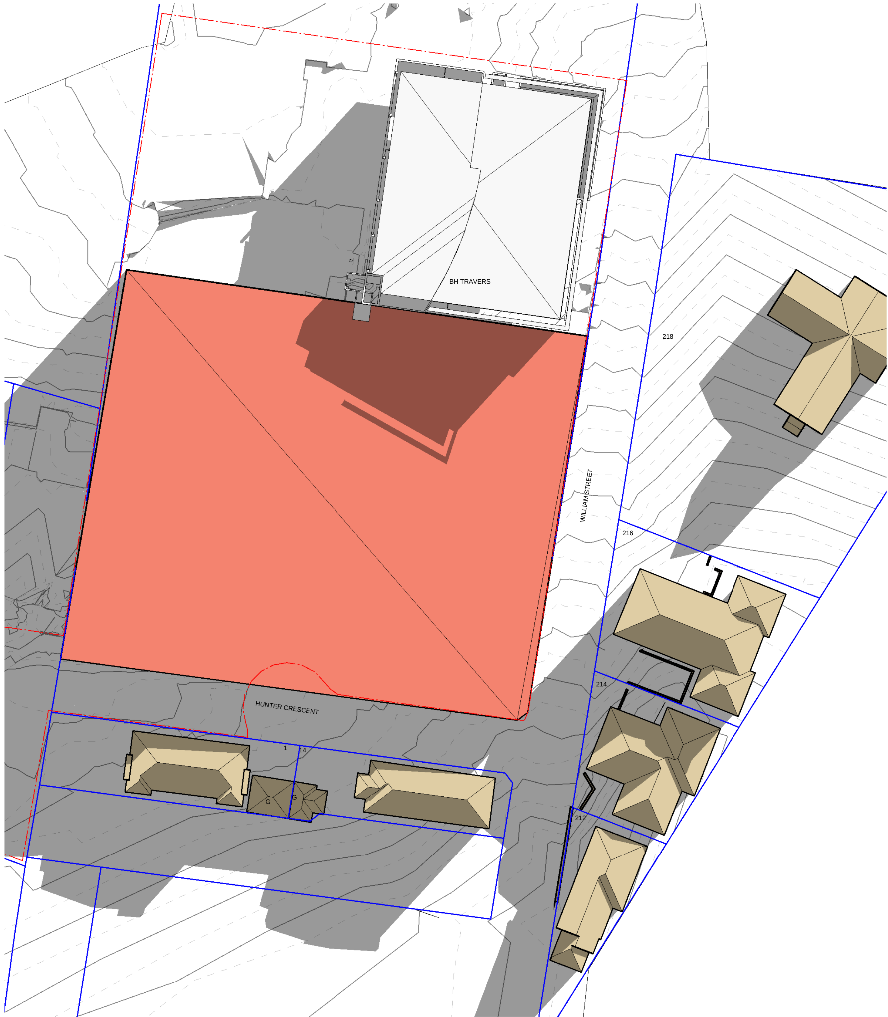
1 PLAN - 21 JUNE - 9:00 AM - SHADOW CAST BY 12M HIGH COMPLIANT SCALE 1 : 400
