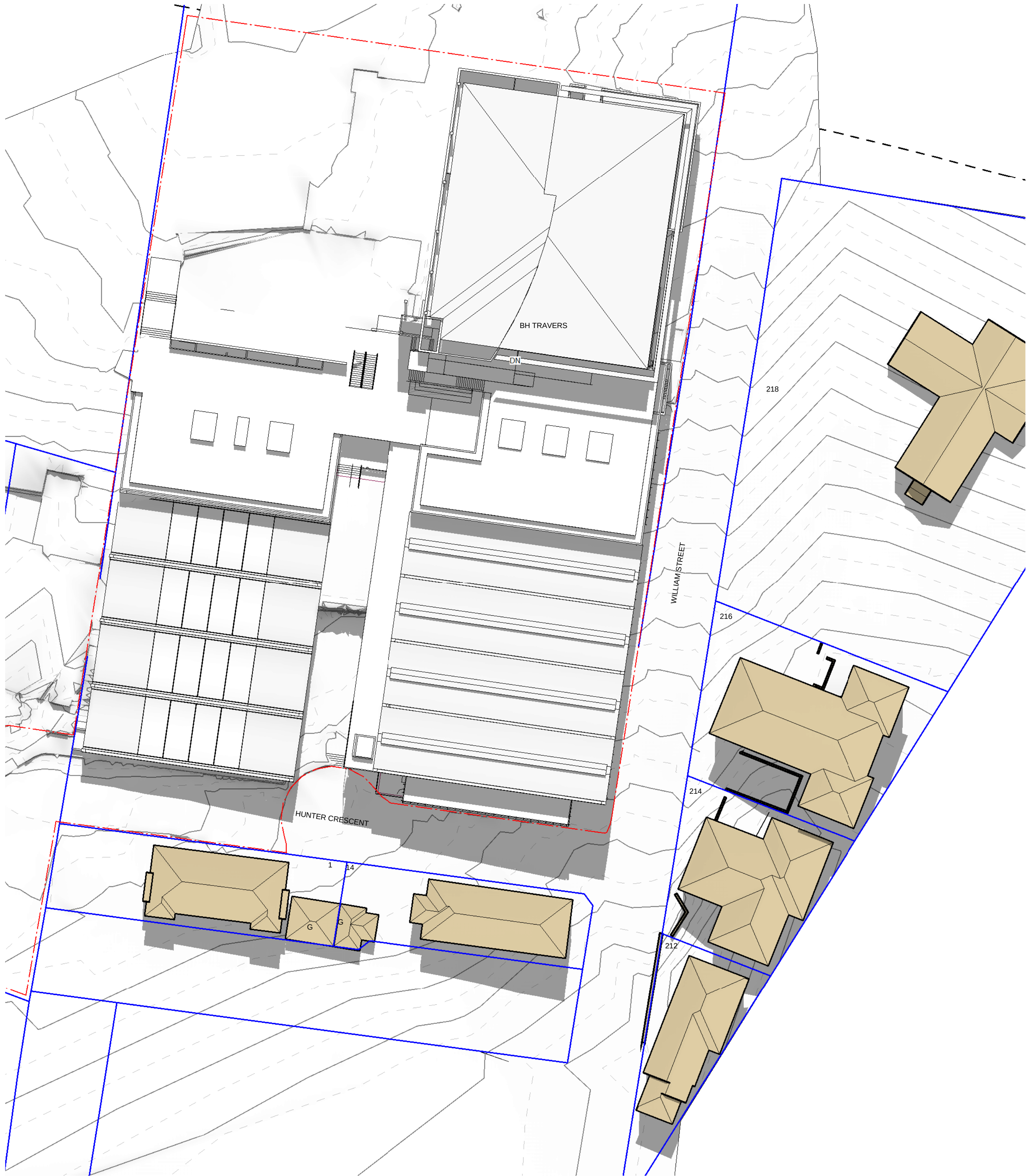
1 PLAN - 21 MARCH - 12:00 NOON - SHADOW CAST BY PROPOSED BUILDINGS SCALE 1 : 400
