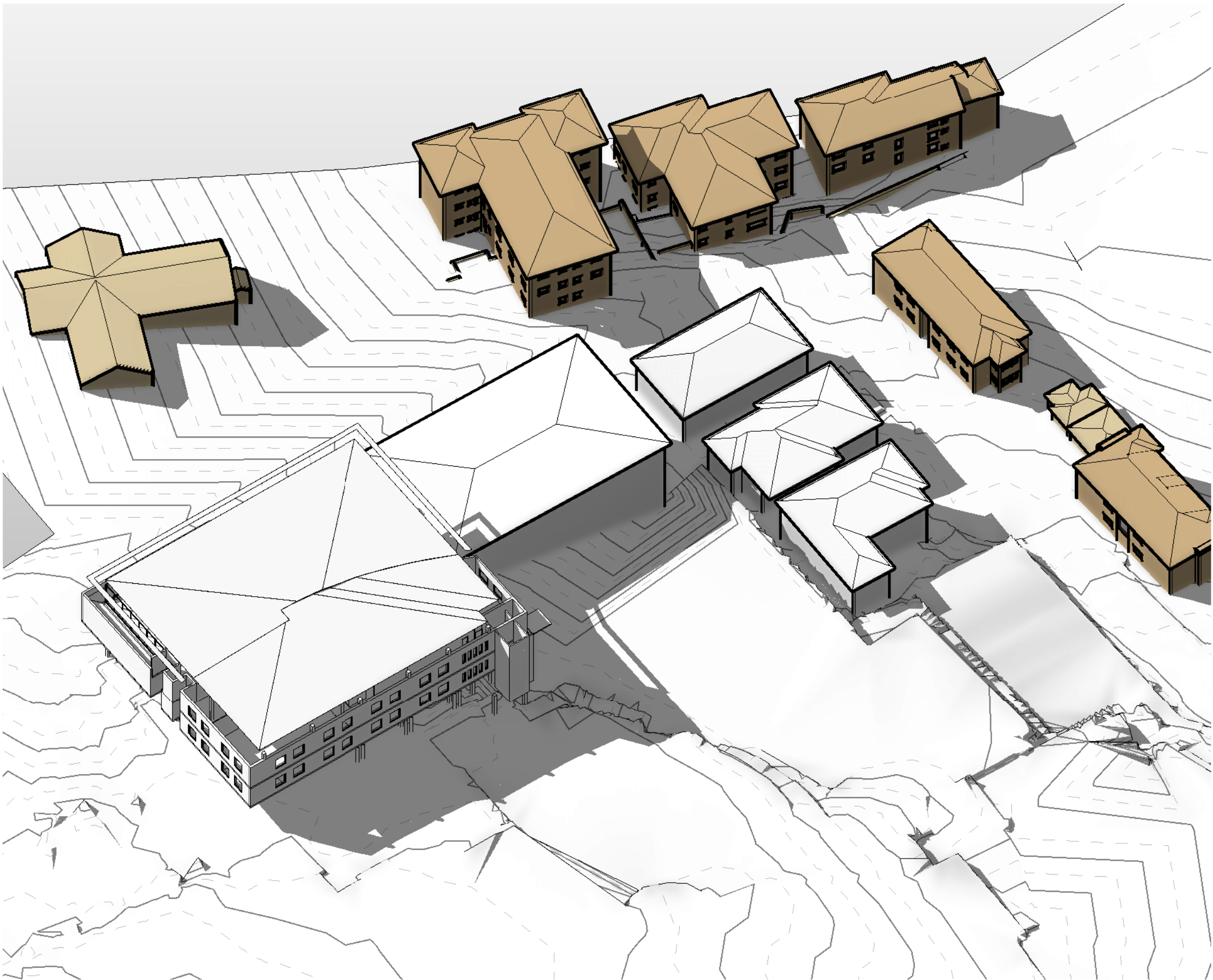
2 3D VIEW - 21 MARCH - 900 AM - SHADOW CAST BY EXISTING BUILDINGS SCALE
