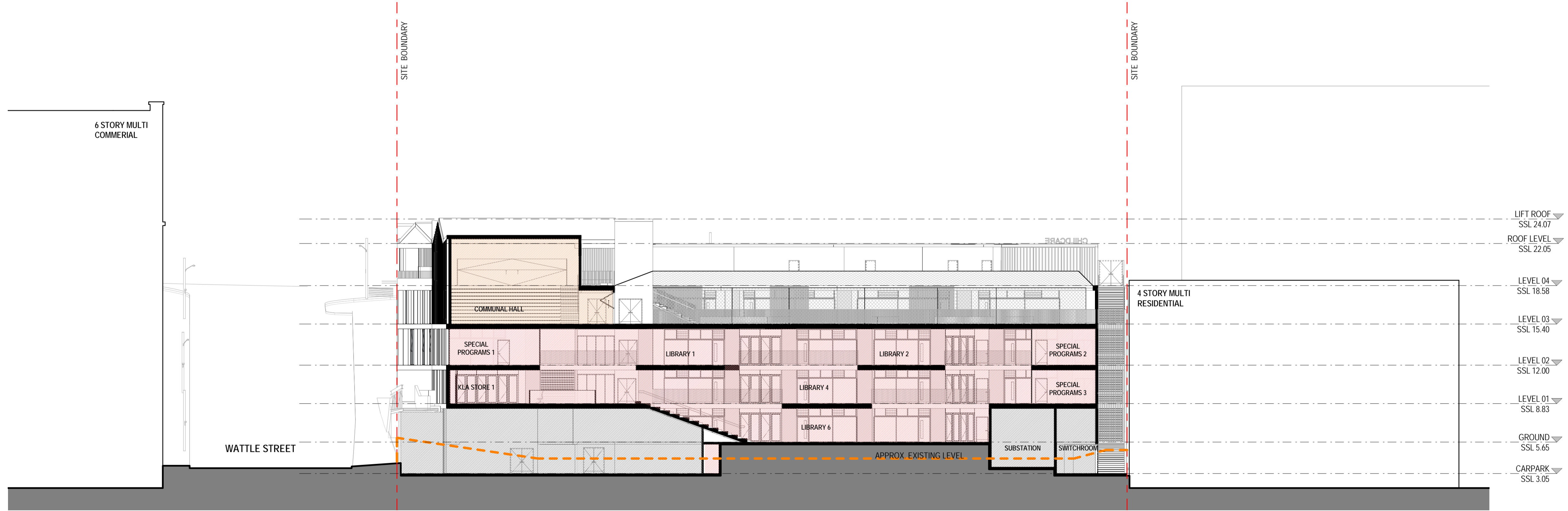
2 DA - SECTION THROUGH LIBRARY DA-4001 SCALE 1:200
