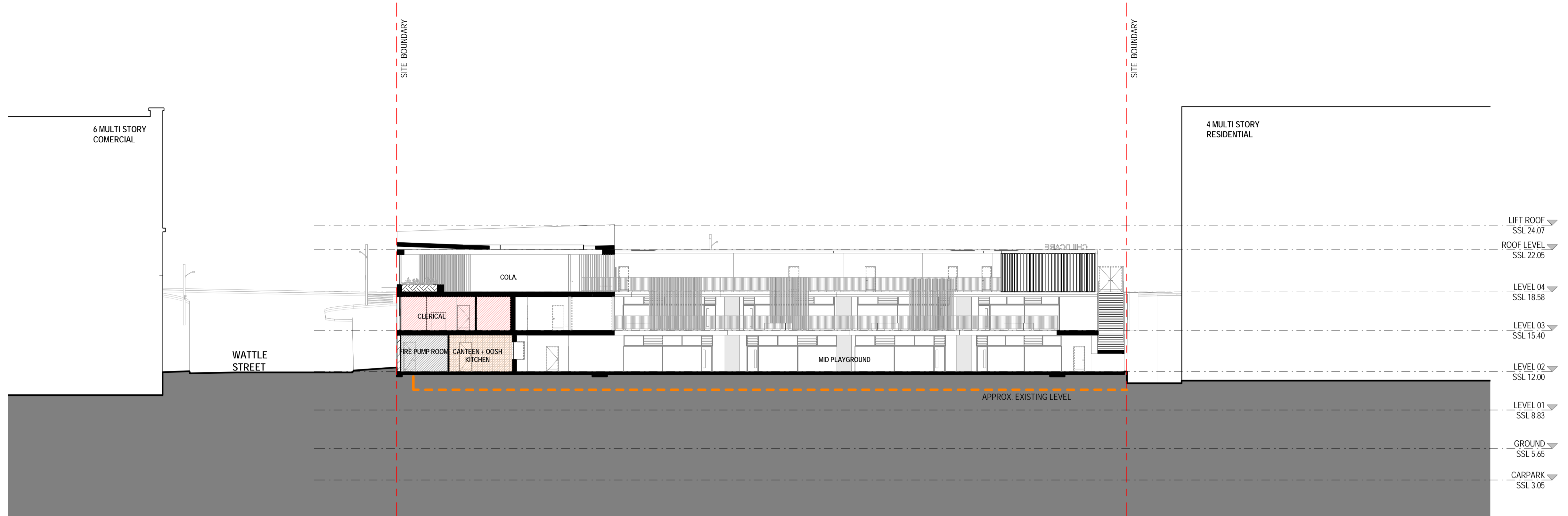
1 DA - SECTION THROUGH MIDDLE PLAYGROUND DA-4001 SCALE 1:200
