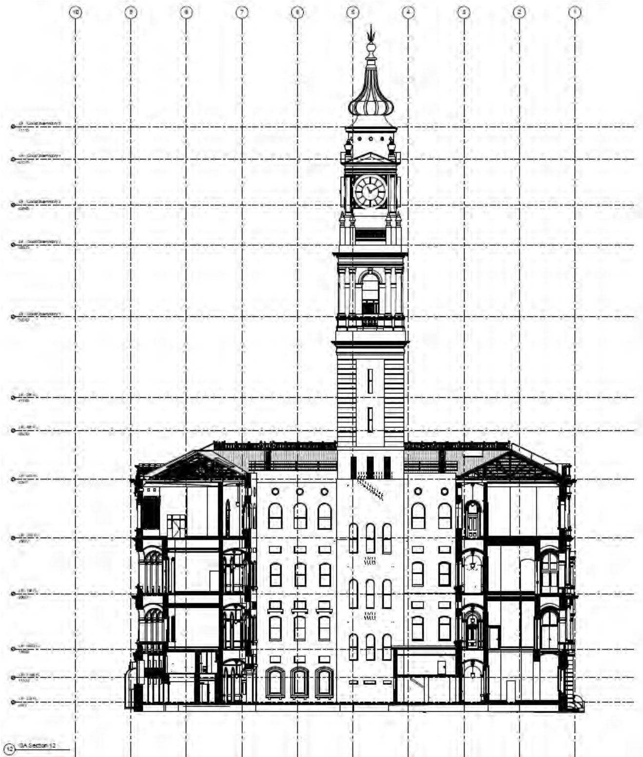
Figure A.36 Lands Building - Existing Section 12 Source: Make Architects
