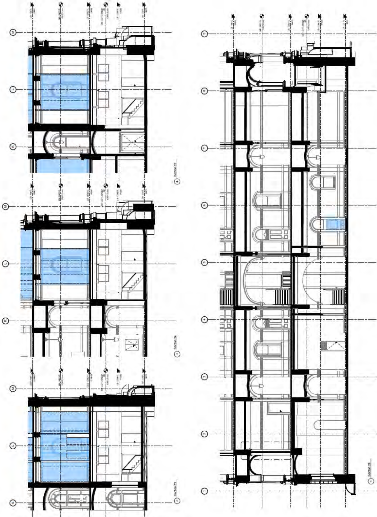
Figure A.41 Lands Building - Existing Sections 23-26 Source: Make Architects
