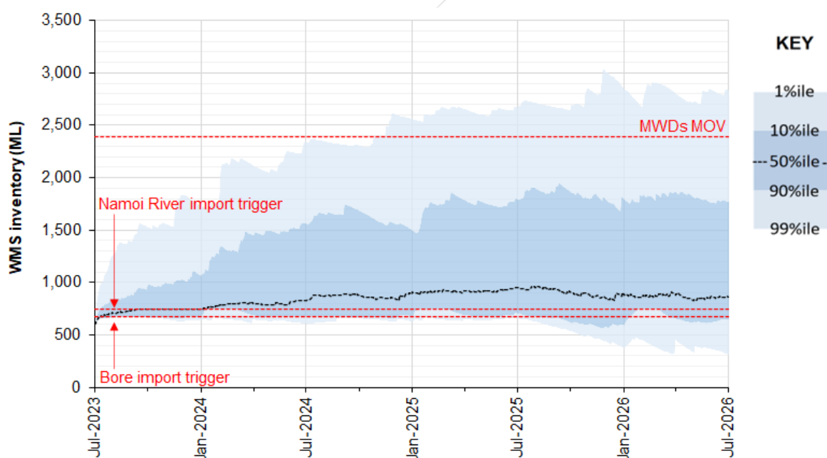
Figure 13 Forecast MWD and Pit Water Storage Combined Inventory
