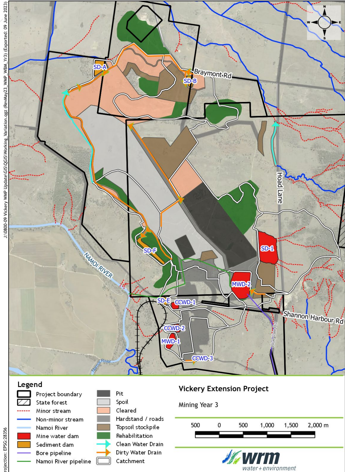
Figure 2c Layout Year 3
