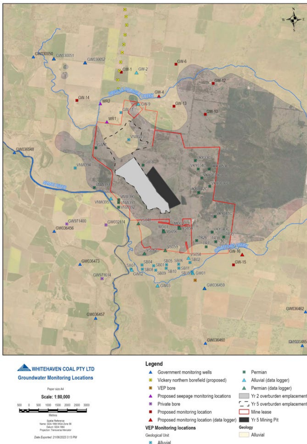
Figure 4-1 VCM Groundwater Monitoring Network
