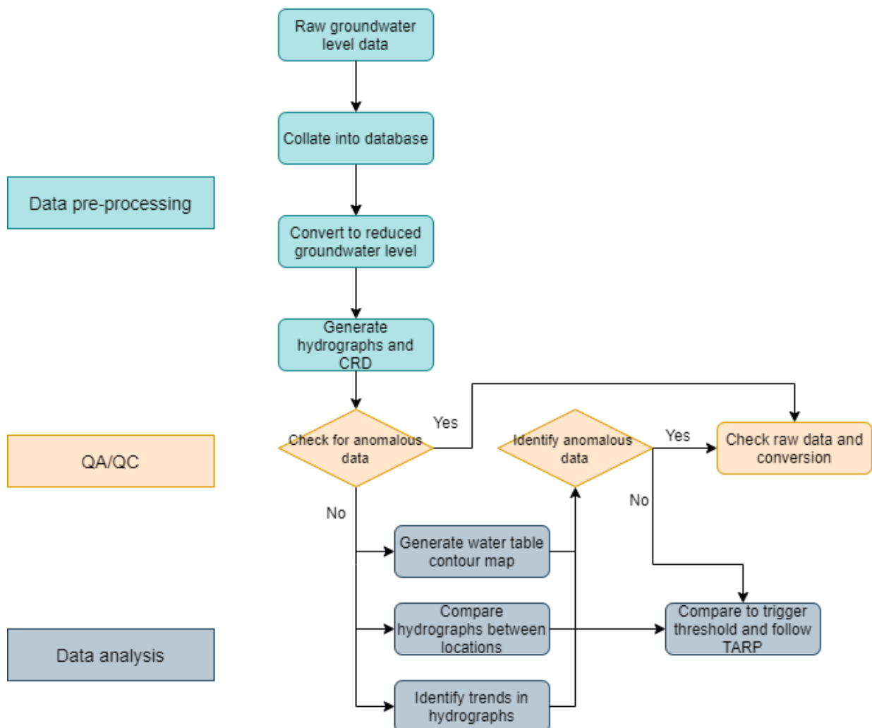
Figure 6-1 Groundwater level data pre-processing and analysis flowchart
