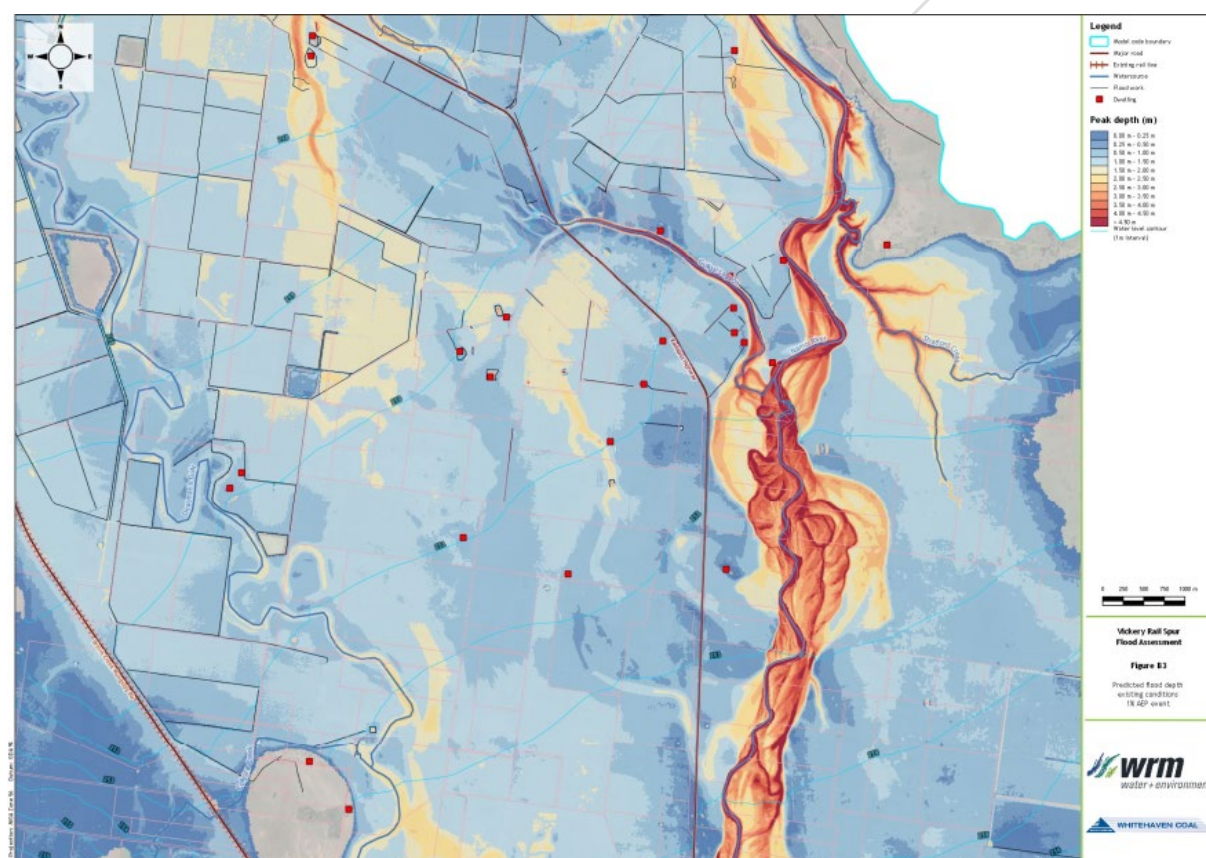
Figure 9 Namoi River Floodplain Depths and Extents for the 1% AEP Event
