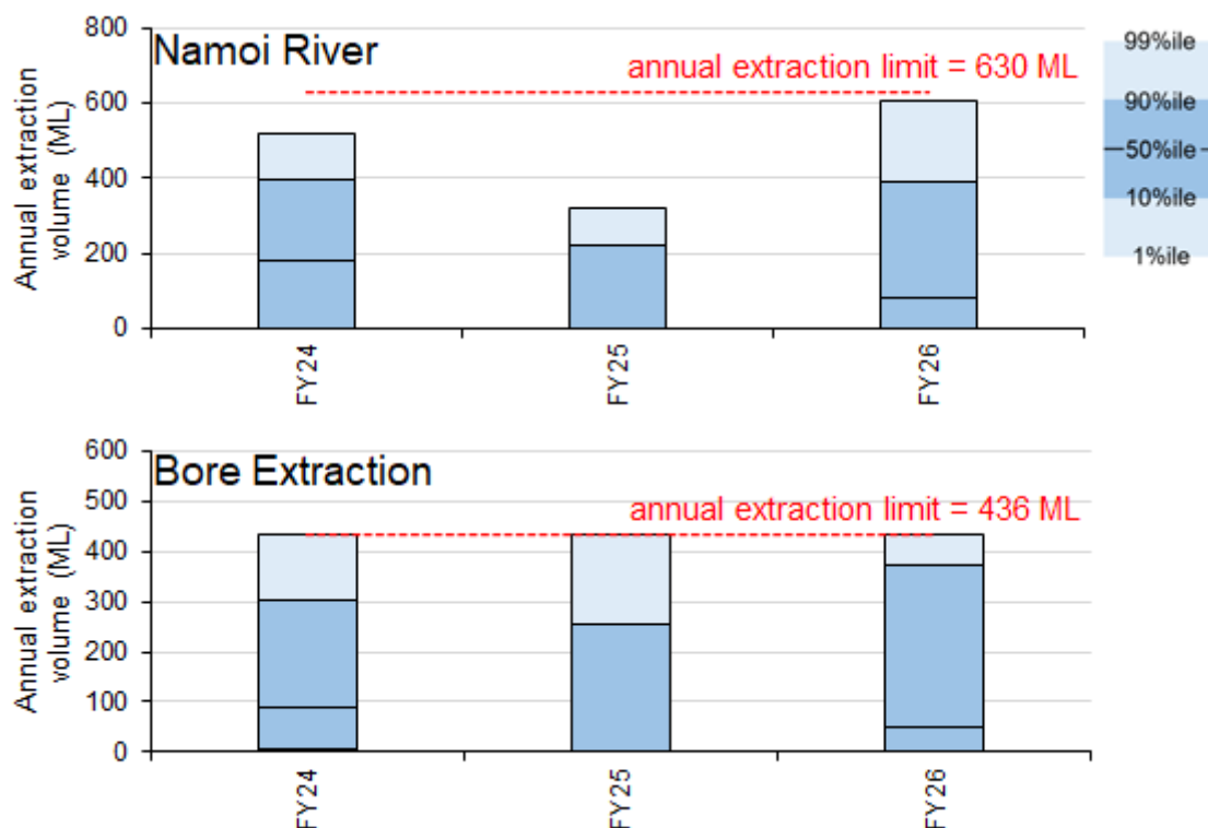
Figure 15 Forecast Total Annual External Water Supply, Namoi River and Groundwater Supply Bore
