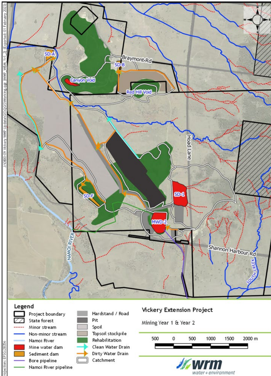
Figure 2a Layout Year 1
