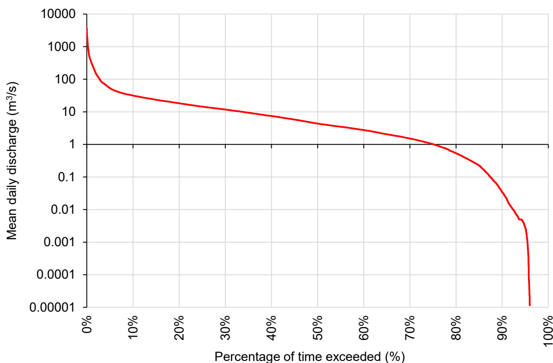
Figure 8 Ranked Flow Plot, Namoi River at Boggabri (Gauge No. 419012)
