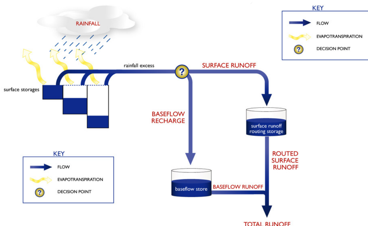
Figure 12 AWBM Model Configuration
