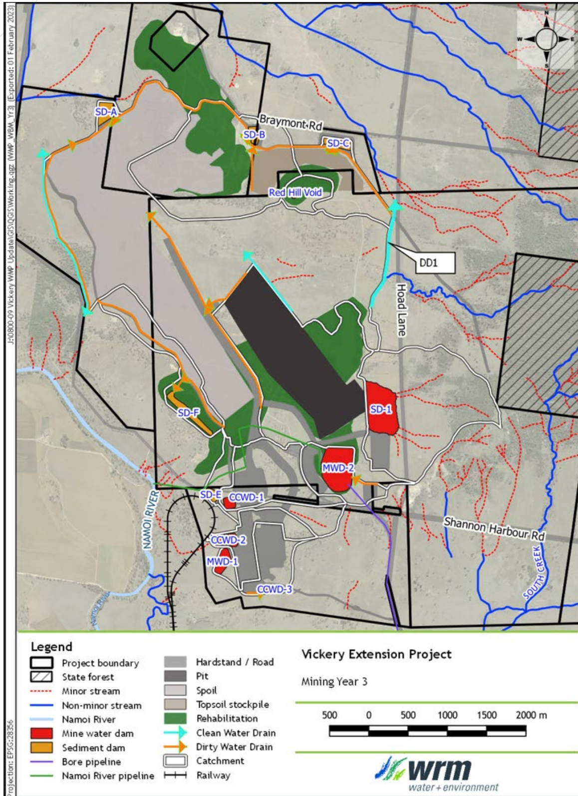
Figure 2b Layout Year 2
