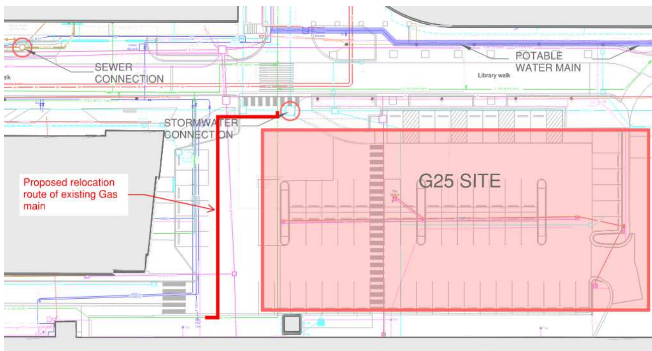
Figure 6 UNSW Kensington Campus Proposed Gas Main Relocation
