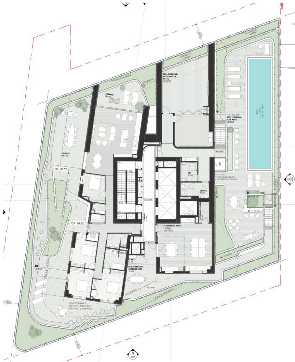
Figure 5: L02 podium terrace – Plan view.
