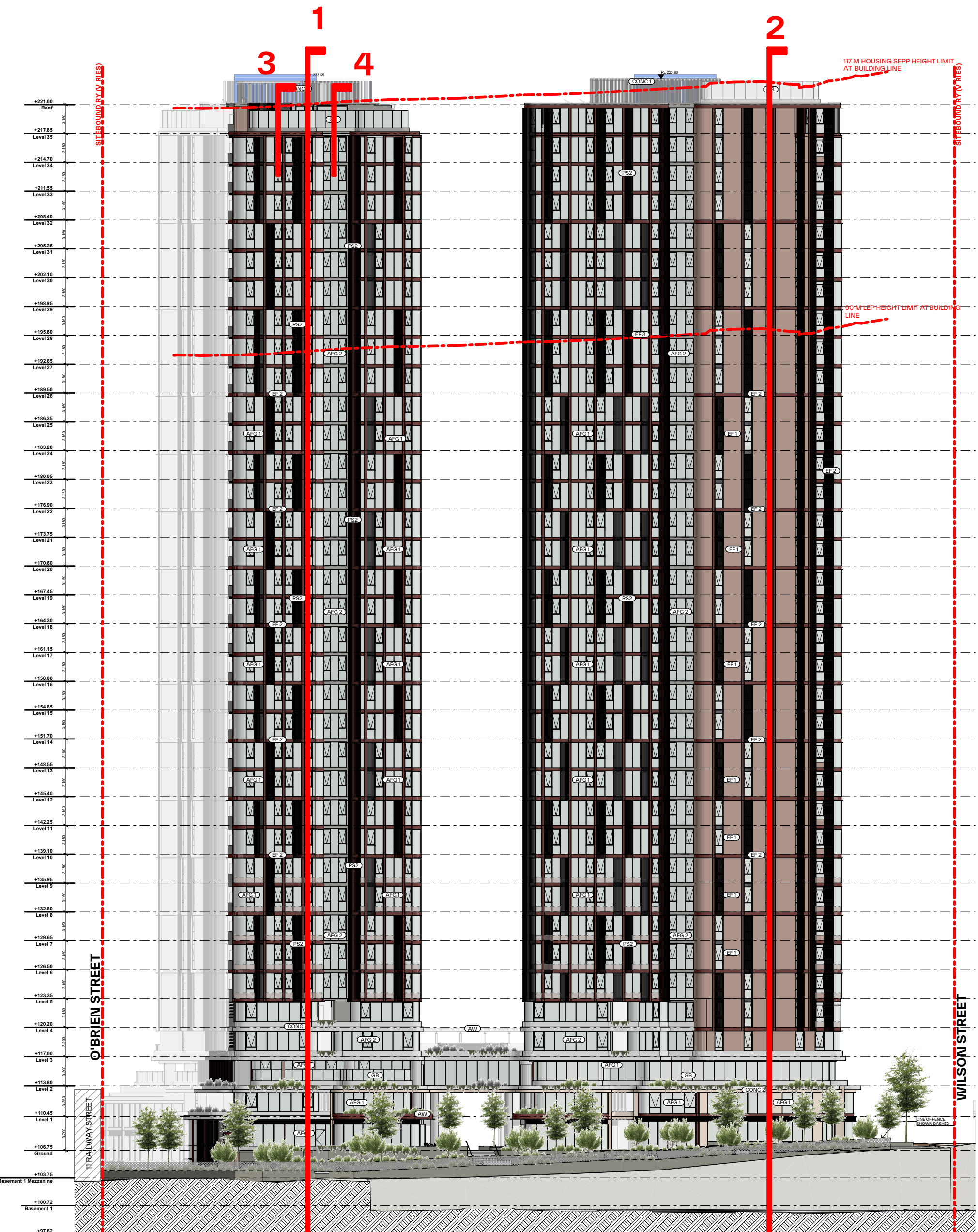
6 KEY ELEVATION Scale 1:400
