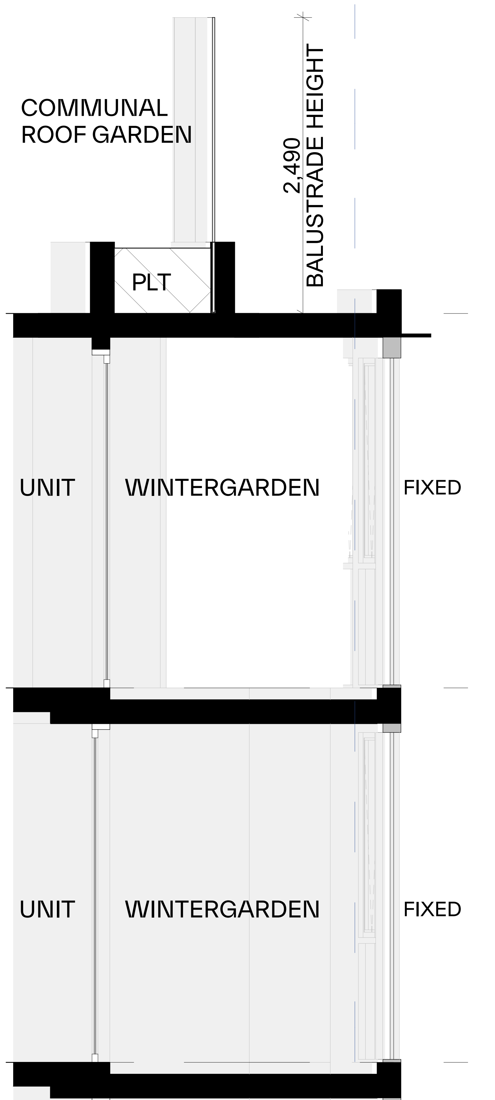
4 Facade Section Detail 02 Scale 1:20
