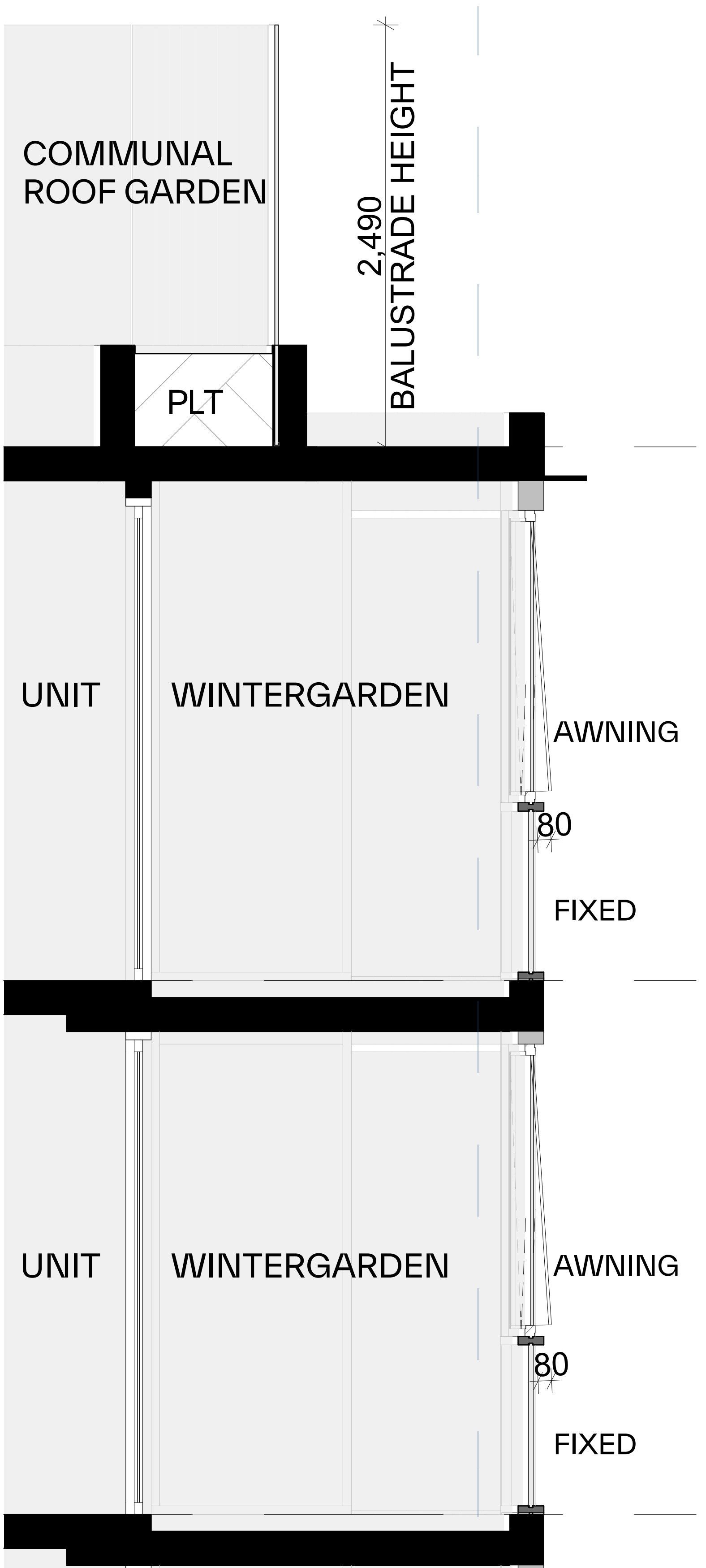
3 Facade Section Detail 01 Scale 1:20
