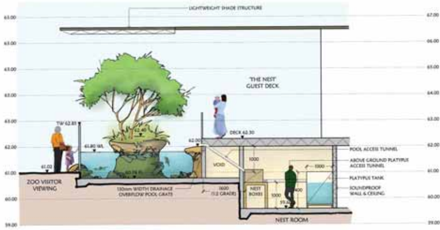
01 PLATYPUS EXHIBIT SECTION A-A 1:50
