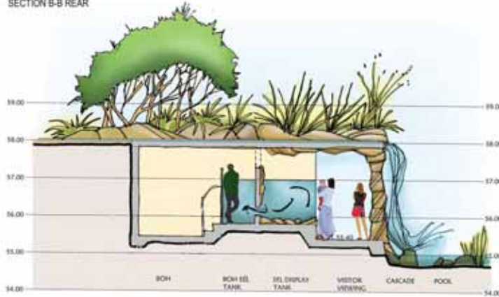
04 EEL EXHIBIT SECTION C-C
