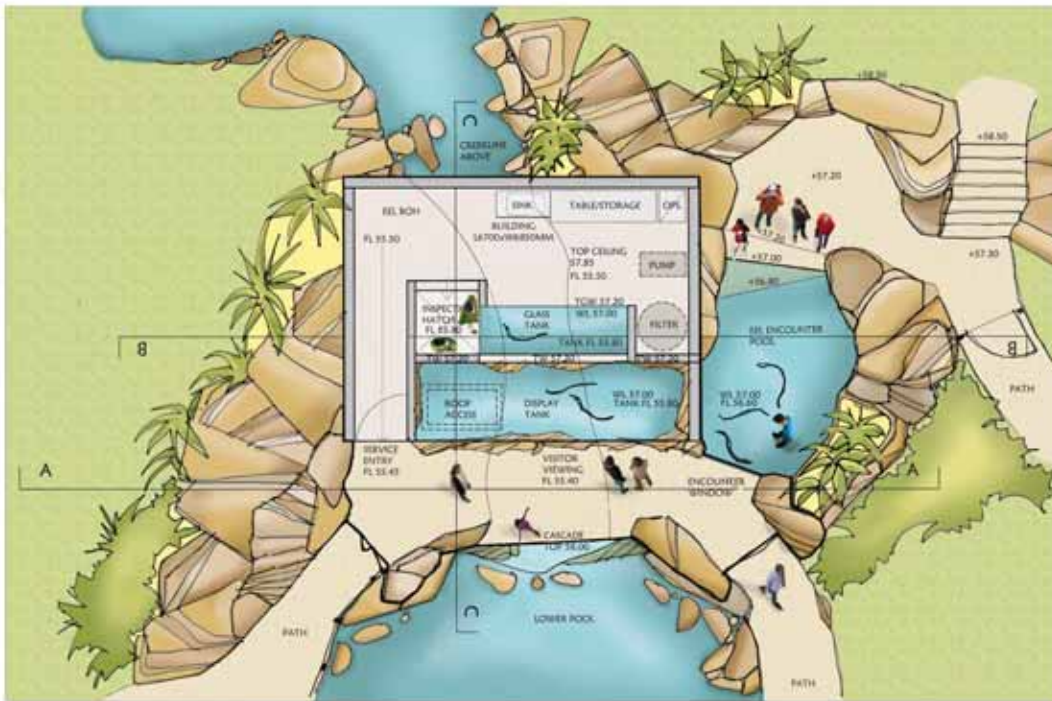
01 EEL EXHIBIT DISPLAY AREA PLAN
