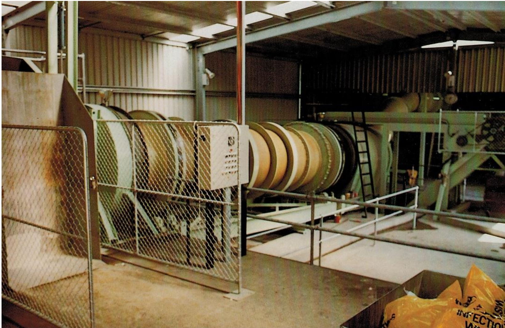
Plate 2 Example Primary Combustion Chamber
