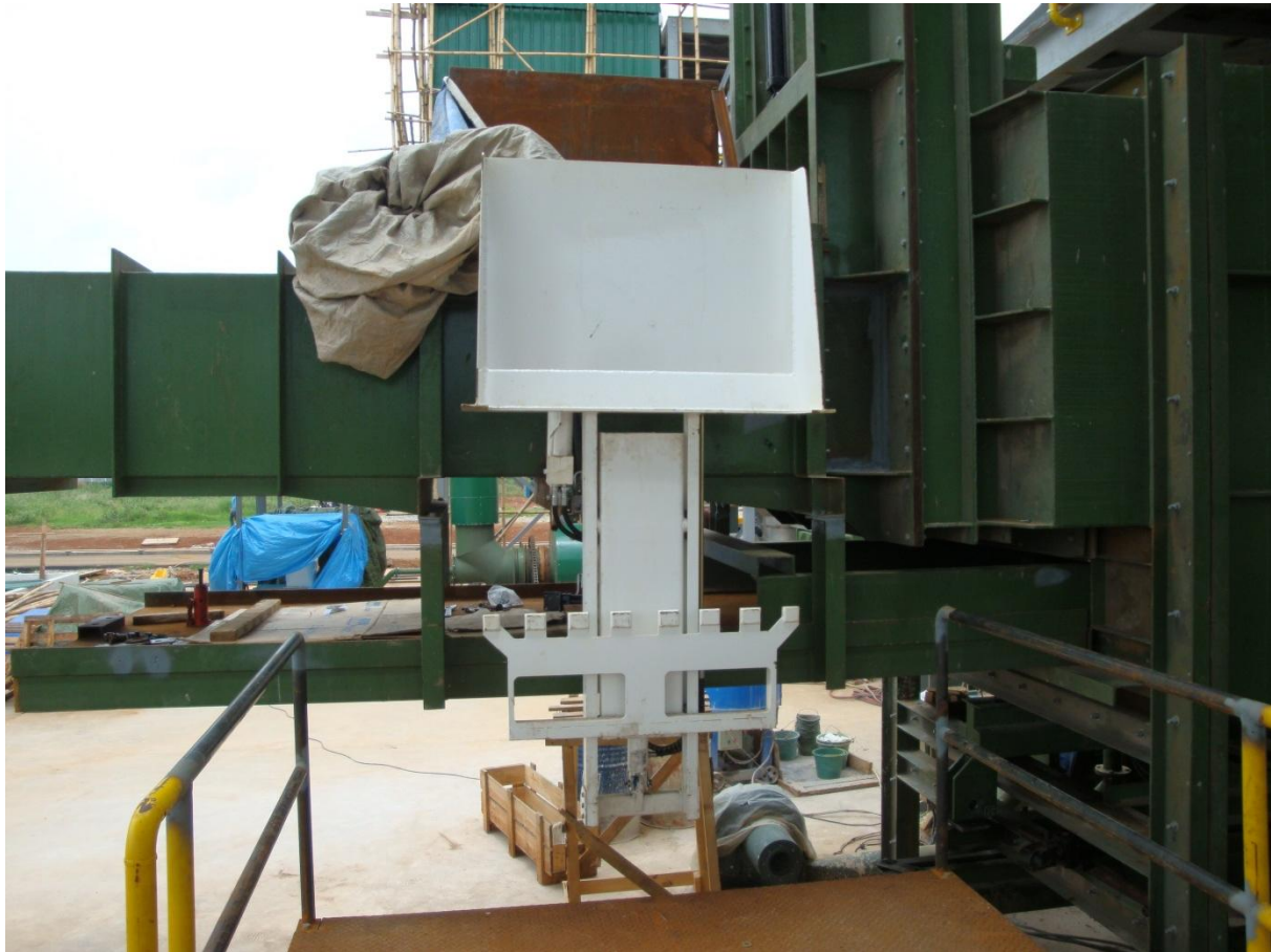
Plate 1 Bin Tippler
