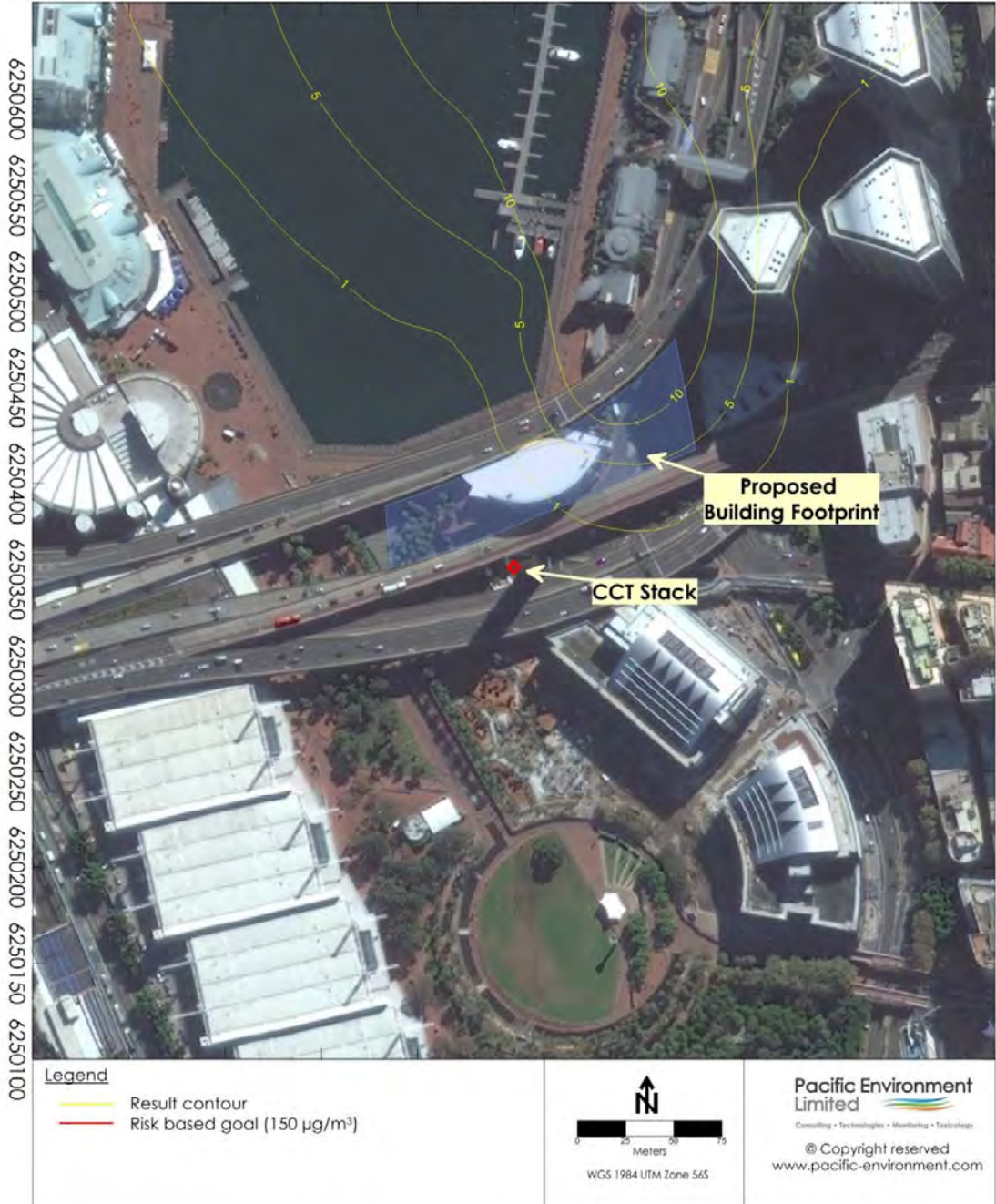
Ground Level – Peak Emissions Scenario – 1-Hour NO 2 Concentration (Goal – 150 µg/m 3 )
