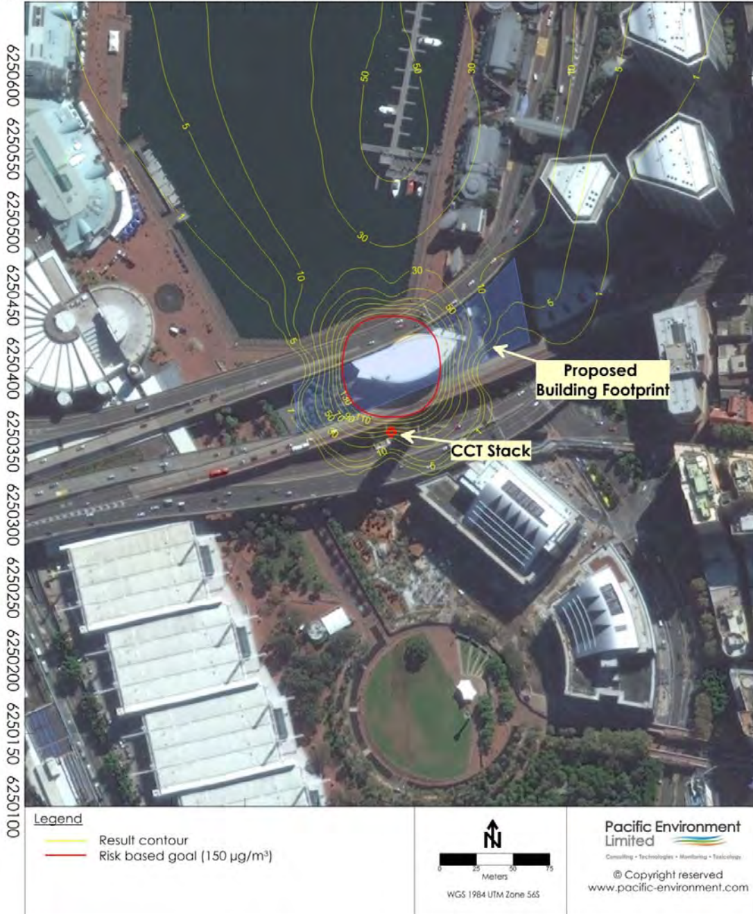
80 m – Peak Emissions Scenario – 1-Hour NO 2 Concentration (Goal – 150 µg/m 3 )
