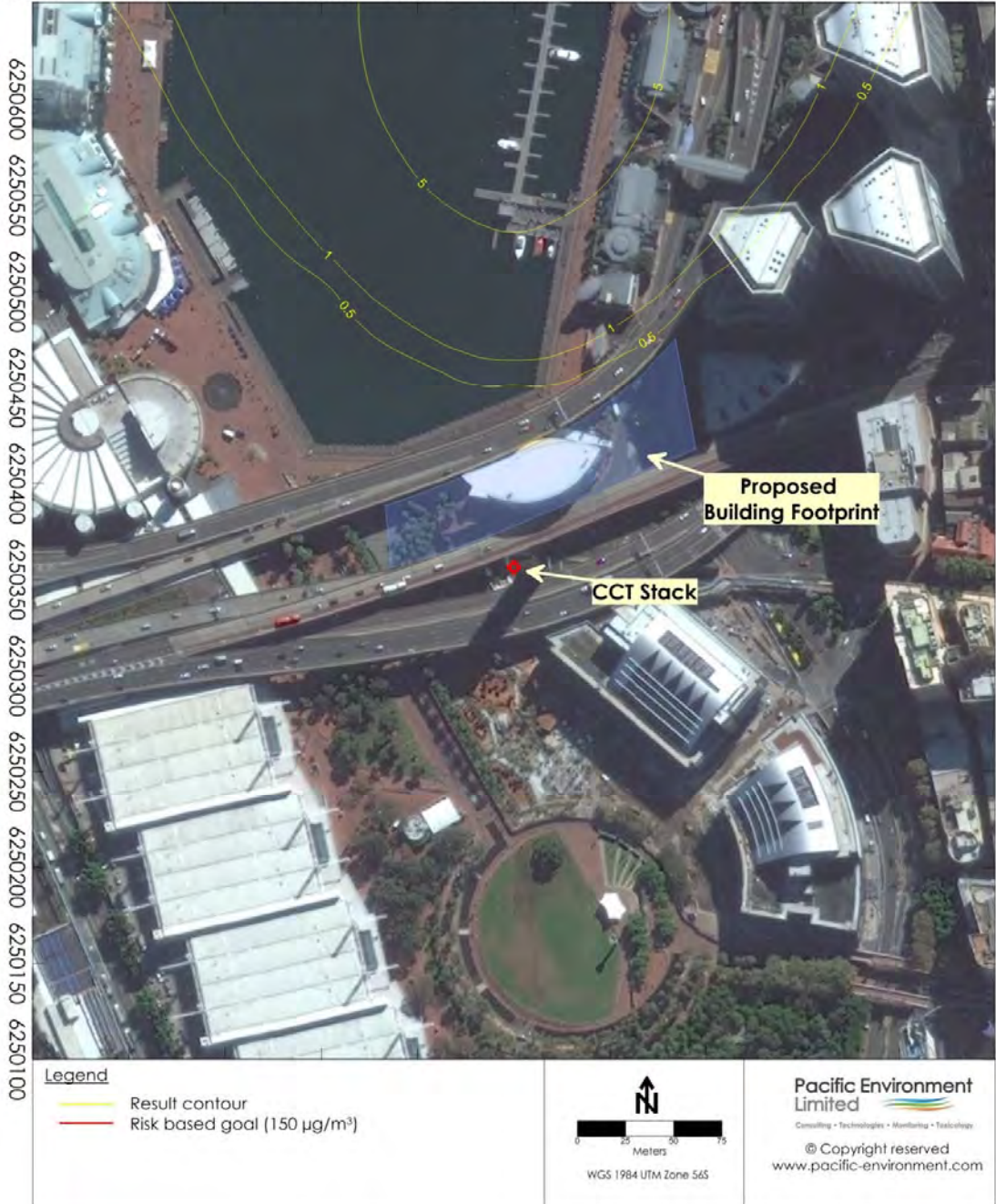
Ground Level – No Building Medium Emissions Scenario – 1-Hour \text{NO}_2 Concentration
