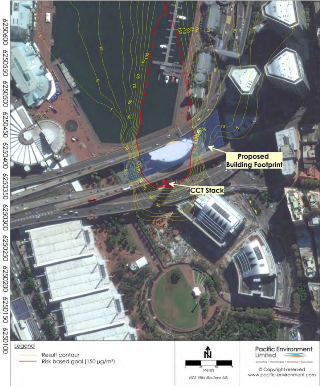
90 m - Medium Emissions Scenario – 1-Hour \text{NO}_2 Concentration (Goal – 150 \mu\text{g}/\text{m}^3 )
