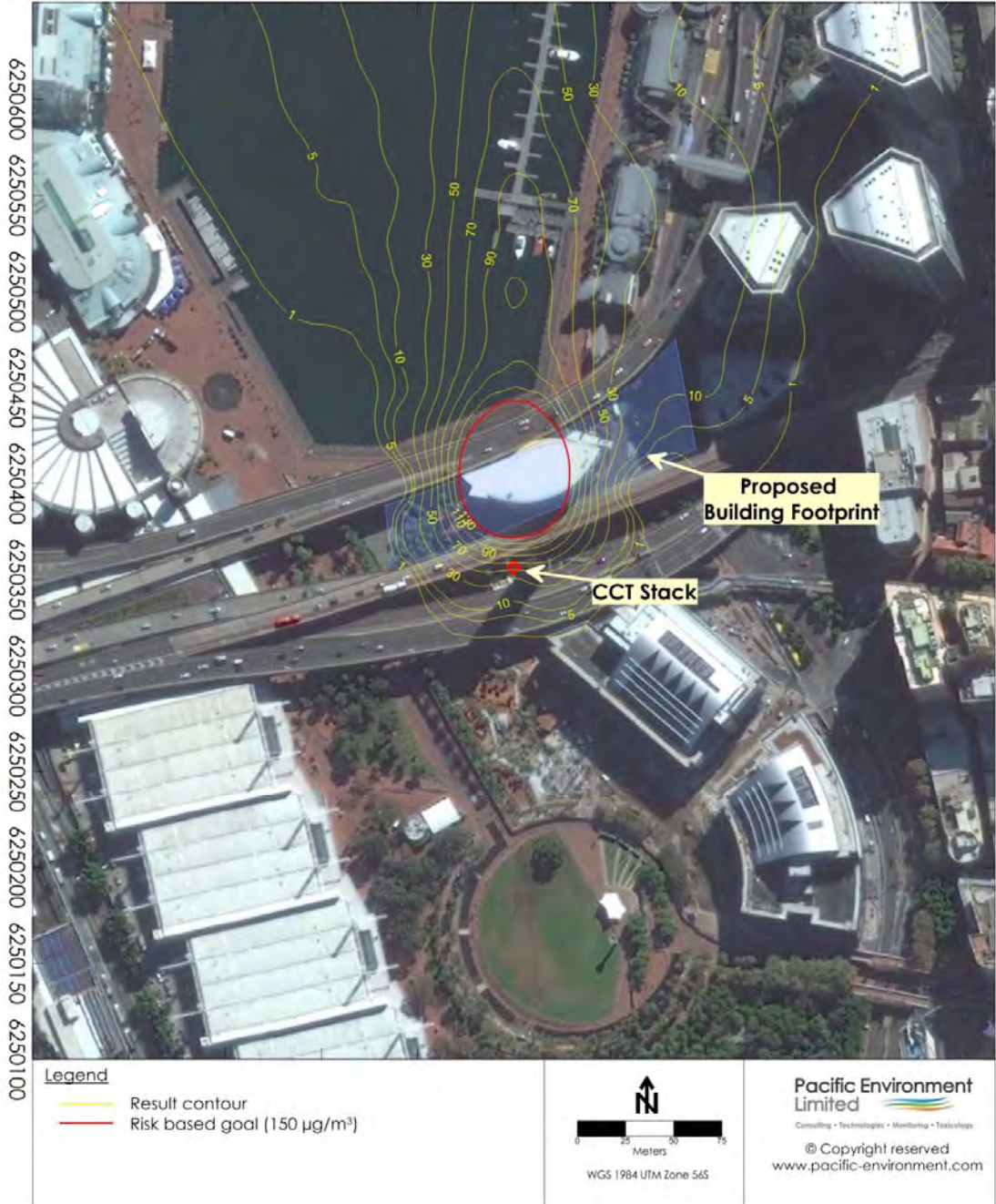
70 m - Low Emissions Scenario - 1-Hour \text{NO}_2 Concentration (Goal - 150 \mu\text{g}/\text{m}^3 - Red Line)
