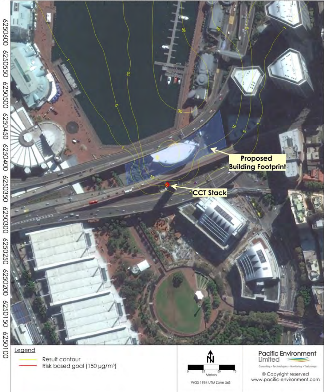
60 m – Low Emissions Scenario – 1-Hour \text{NO}_2 Concentration (Goal – 150 \mu\text{g}/\text{m}^3 )
