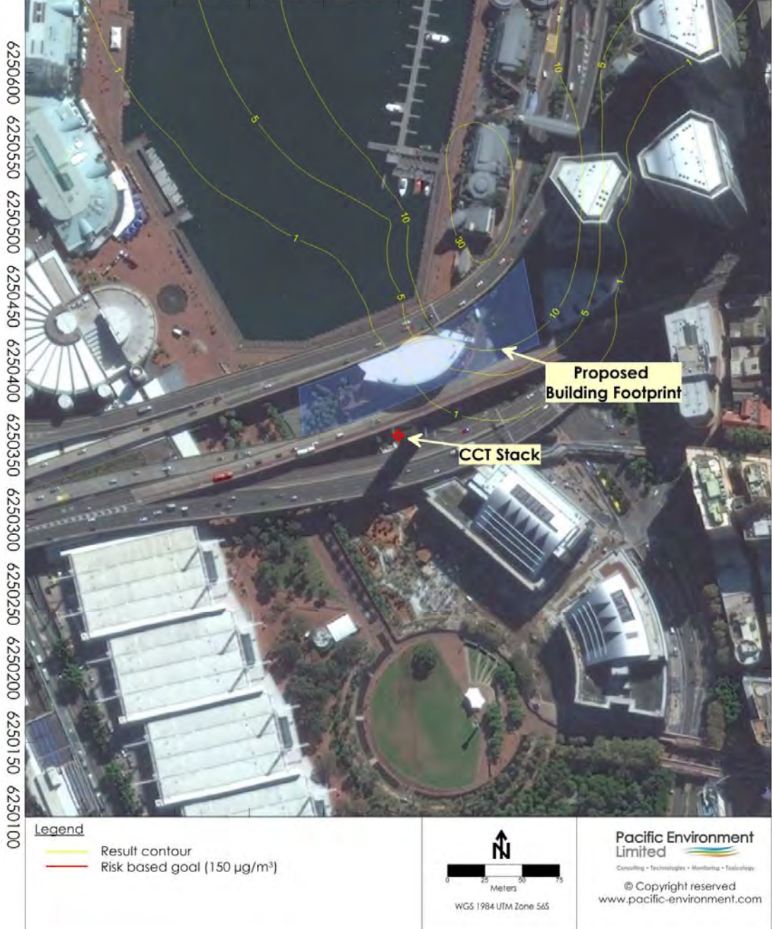
Ground Level – Medium Emissions Scenario – 1-Hour NO 2 Concentration (Goal – 150 µg/m 3 )
