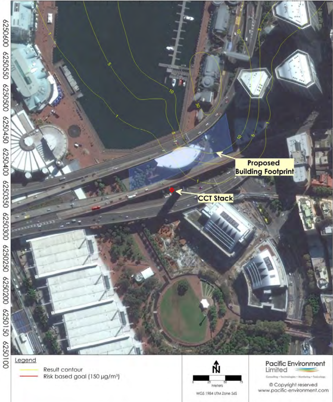
30 m – Medium Emissions Scenario – 1-Hour NO 2 Concentration (Goal – 150 µg/m 3 )
