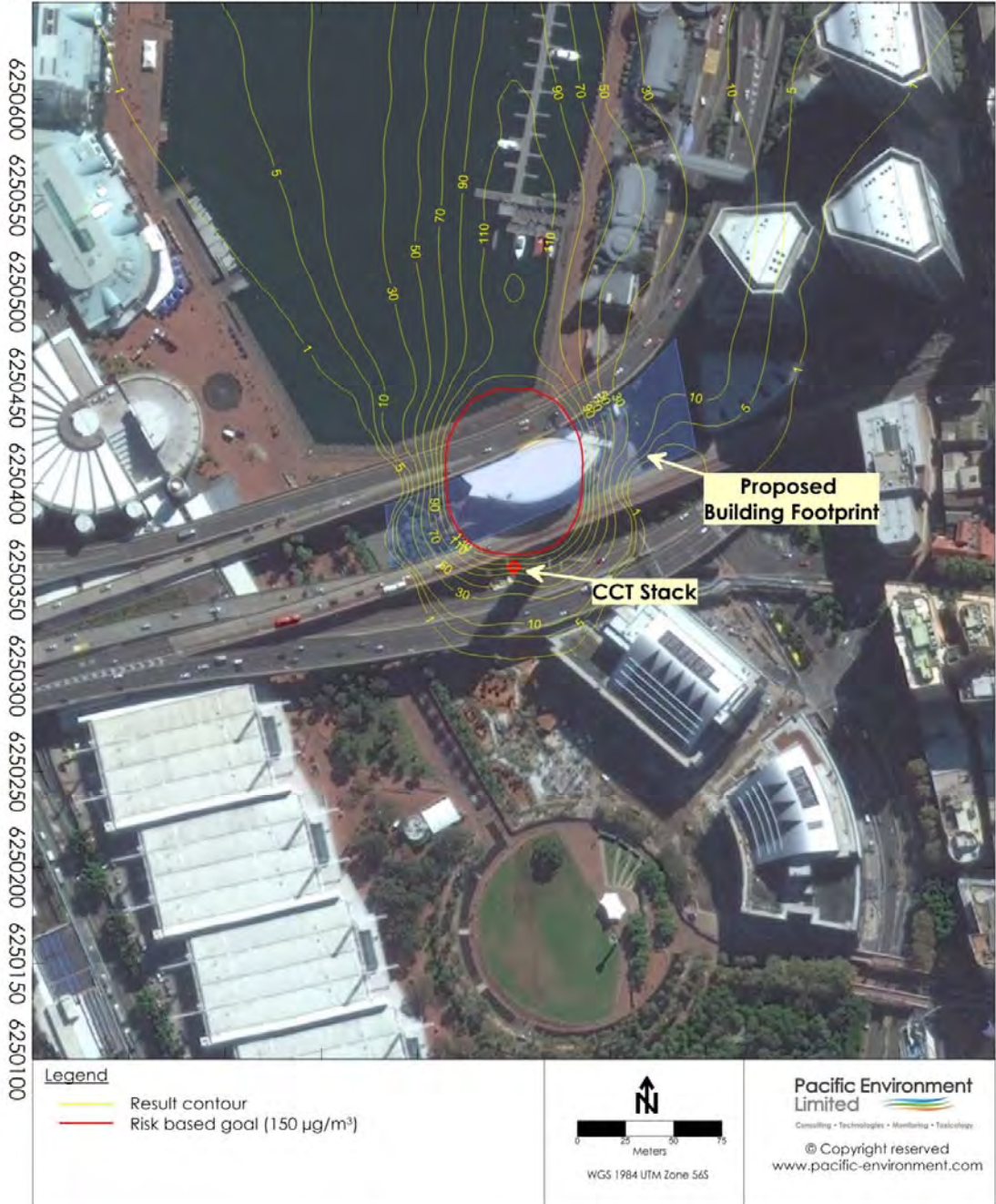
80 m - Medium Emissions Scenario – 1-Hour NO 2 Concentration (Goal – 150 µg/m 3 )
