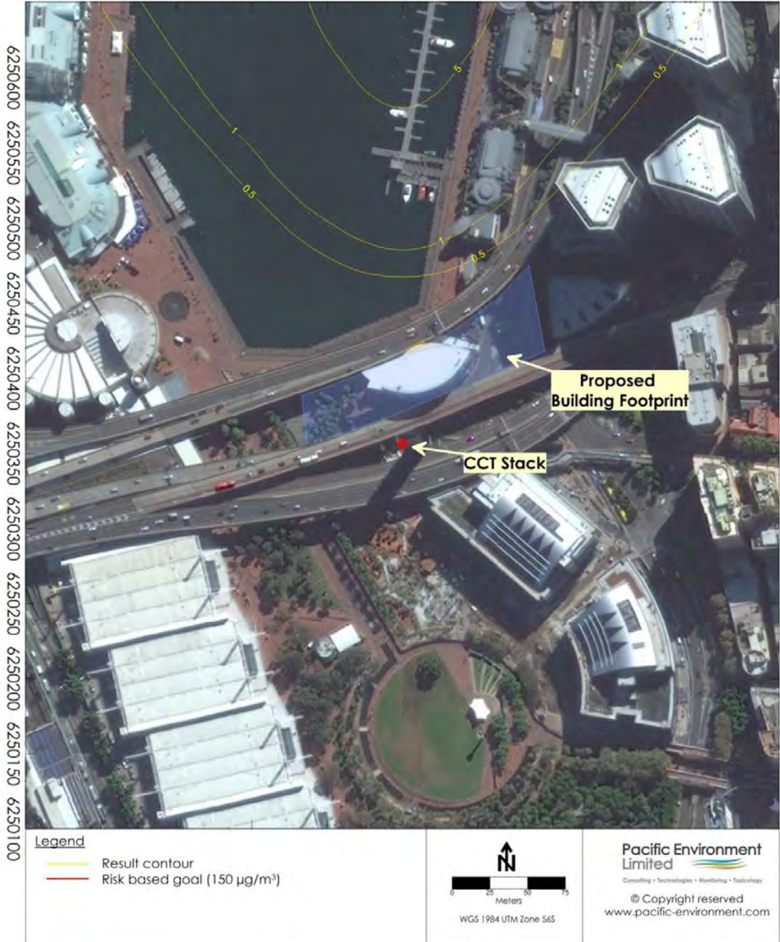
Ground Level – No Building Peak Emissions Scenario – 1-Hour NO 2 Concentration (Goal – 150 µg/m 3 )
