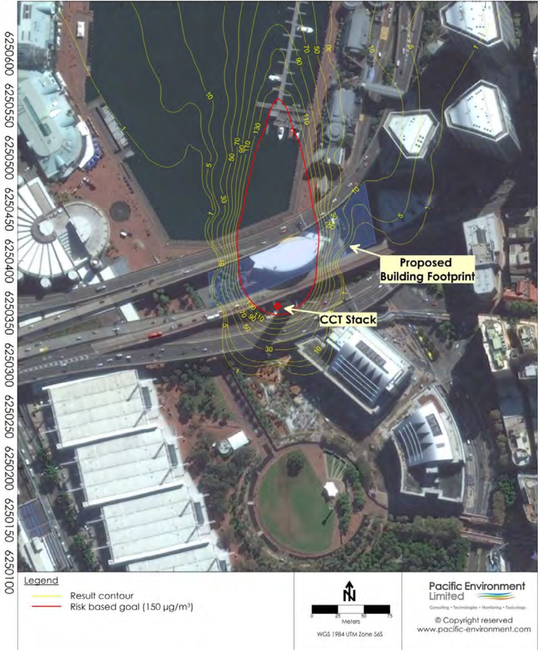
80 m - Low Emissions Scenario – 1-Hour \text{NO}_2 Concentration (Goal – 150 \mu\text{g}/\text{m}^3 - Red Line)
