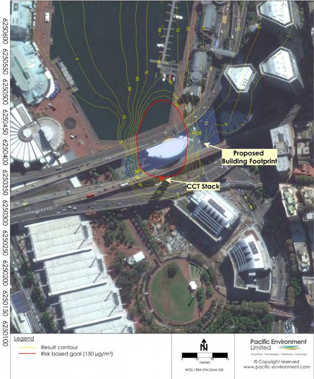
90 m – Peak Emissions Scenario – 1-Hour NO 2 Concentration (Goal – 150 µg/m 3 )
