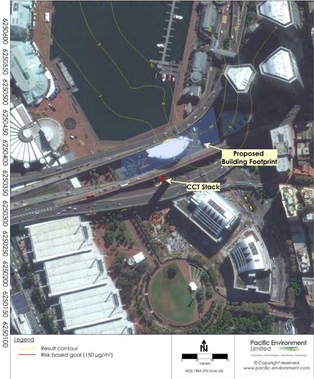
30 m - Peak Emissions Scenario - 1-Hour NO 2 Concentration (Goal - 150 µg/m 3 )
