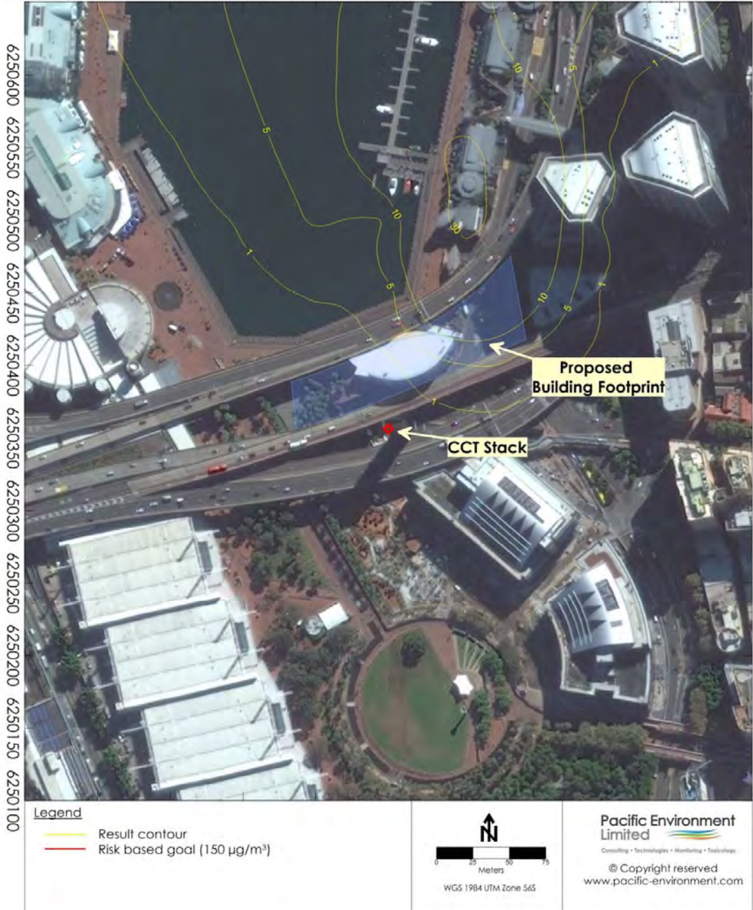
30 m – Low Emissions Scenario – 1-Hour NO 2 Concentration (Goal – 150 µg/m 3 )
