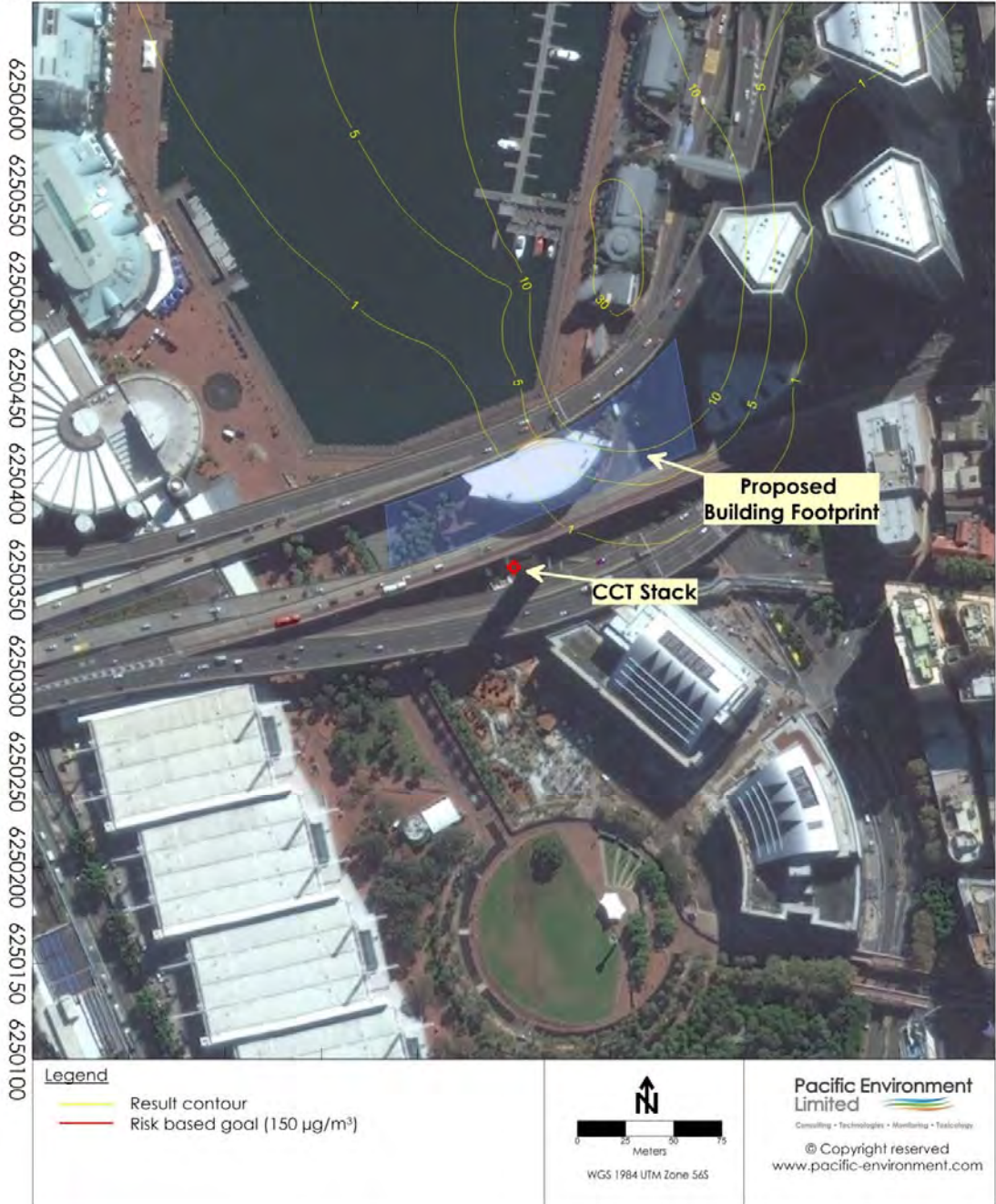
Ground Level – Low Emissions Scenario – 1-Hour \text{NO}_2 Concentration (Goal – 150 \mu\text{g}/\text{m}^3 )
