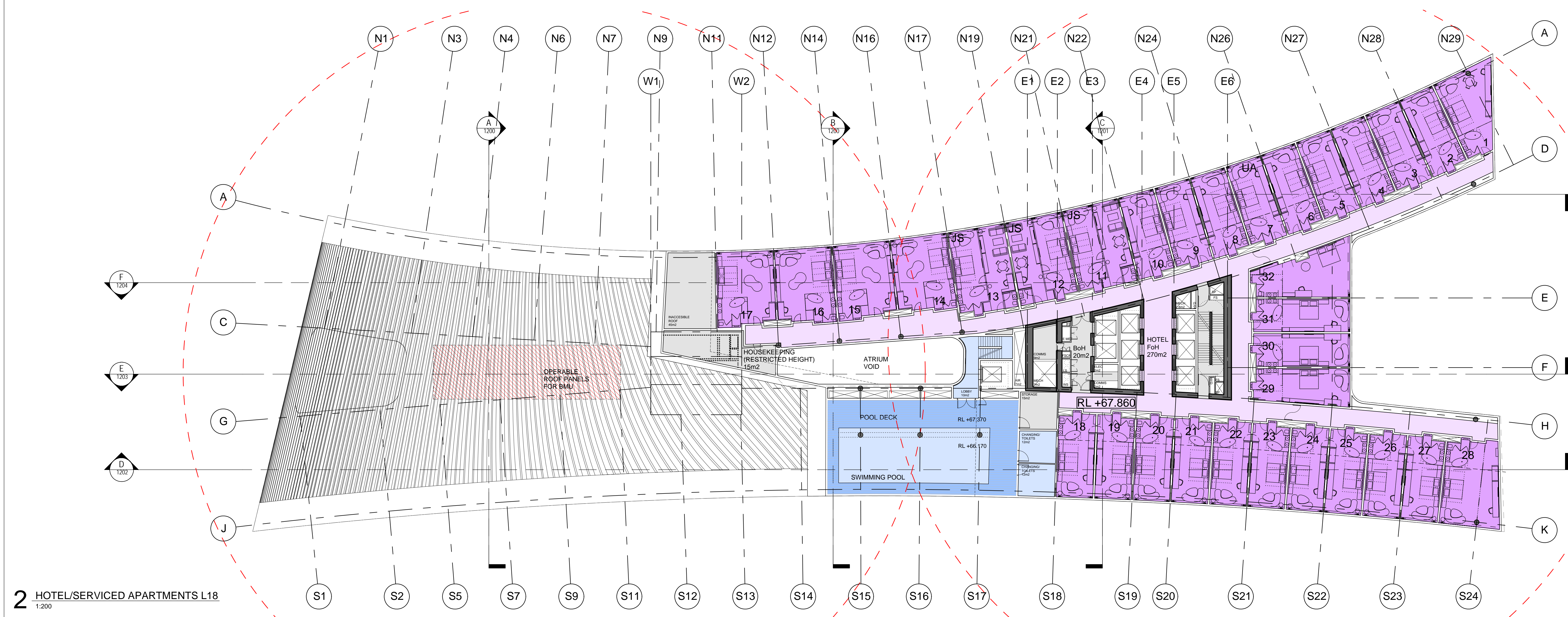
1 HOTEL/SERVICED APARTMENTS L17 1:200
