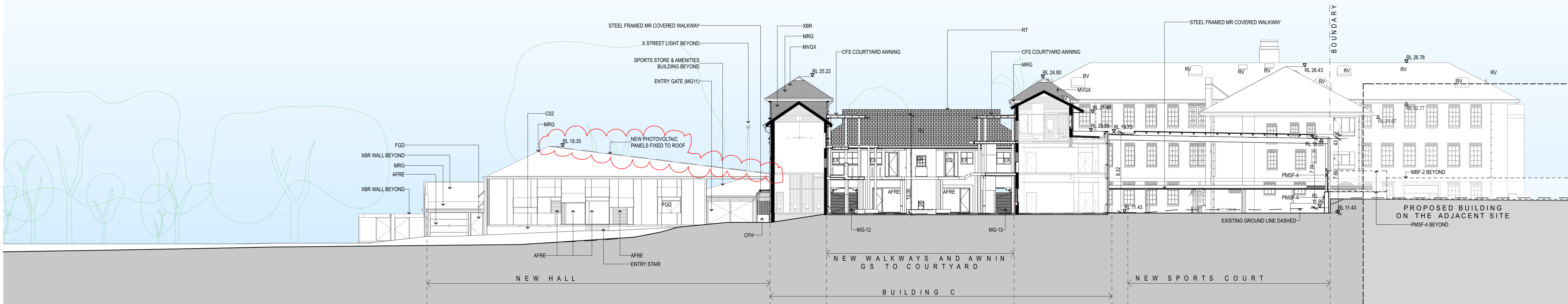
SITE SECTION LOOKING WEST
