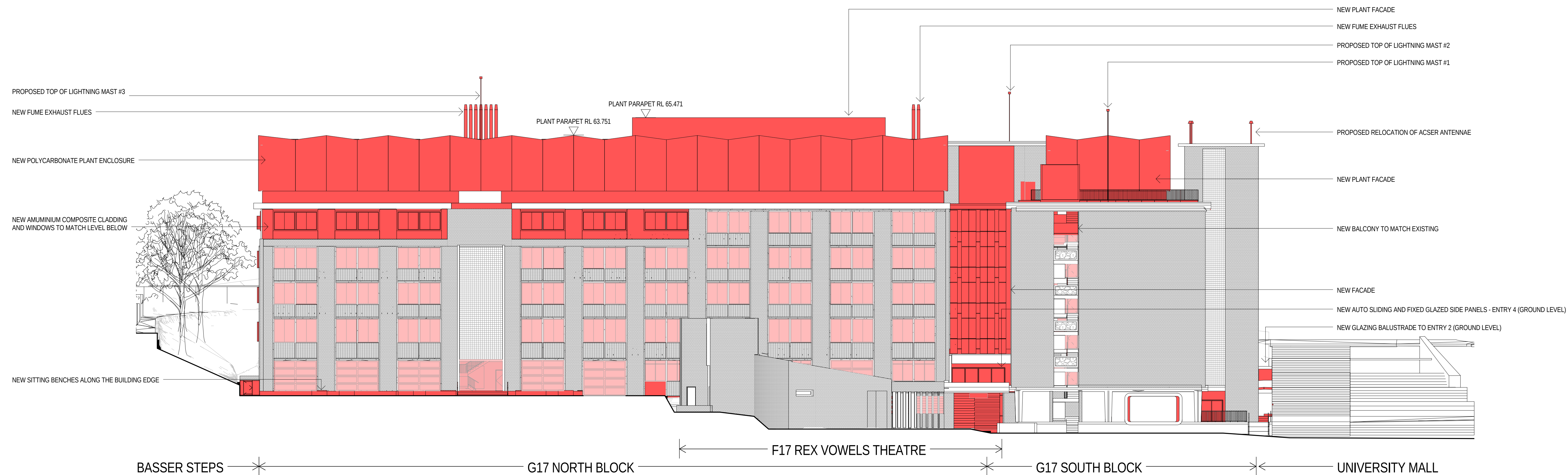
2 ELEVATION - WEST A.1101 1:200
