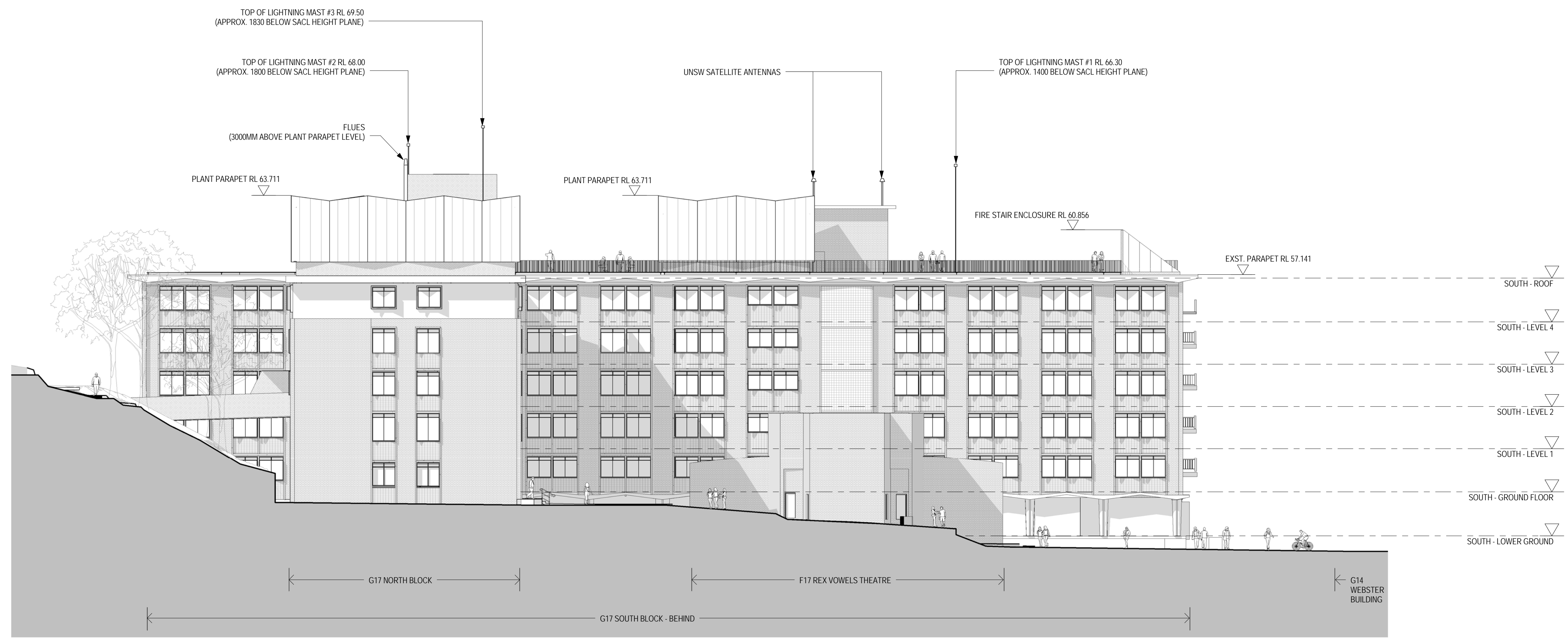
1 ELEVATION - NORTH A.1101 1:200
