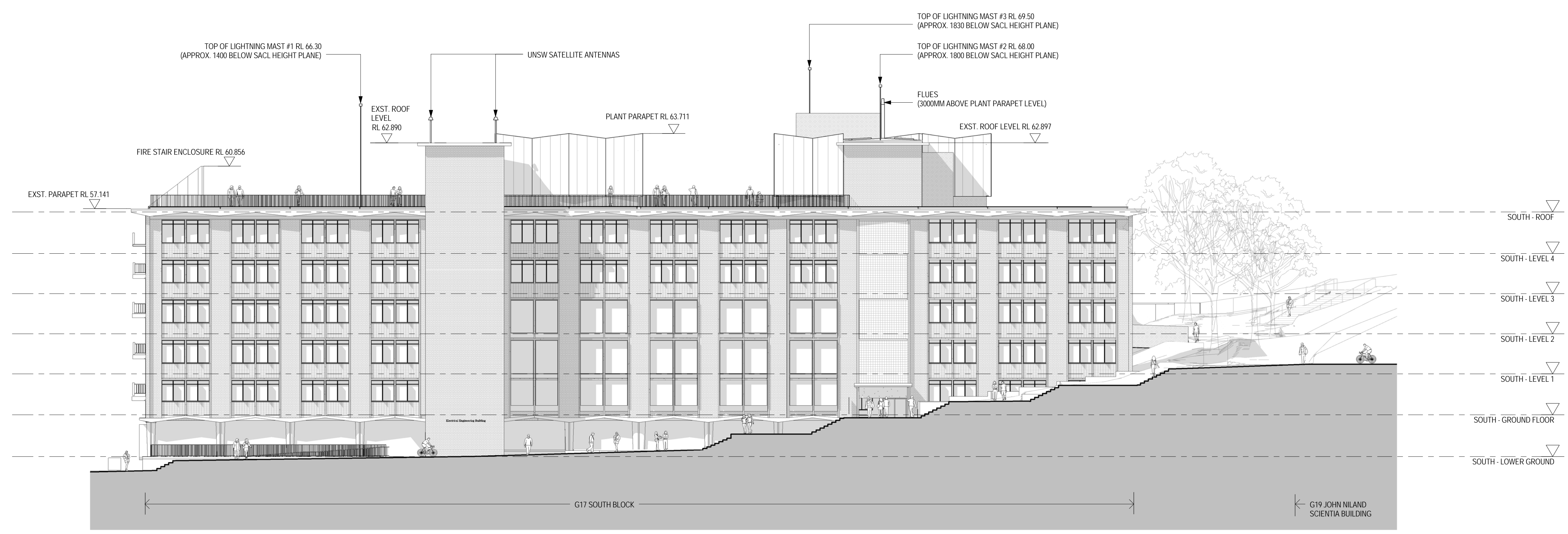
2 ELEVATION - SOUTH A.1101 1:200
