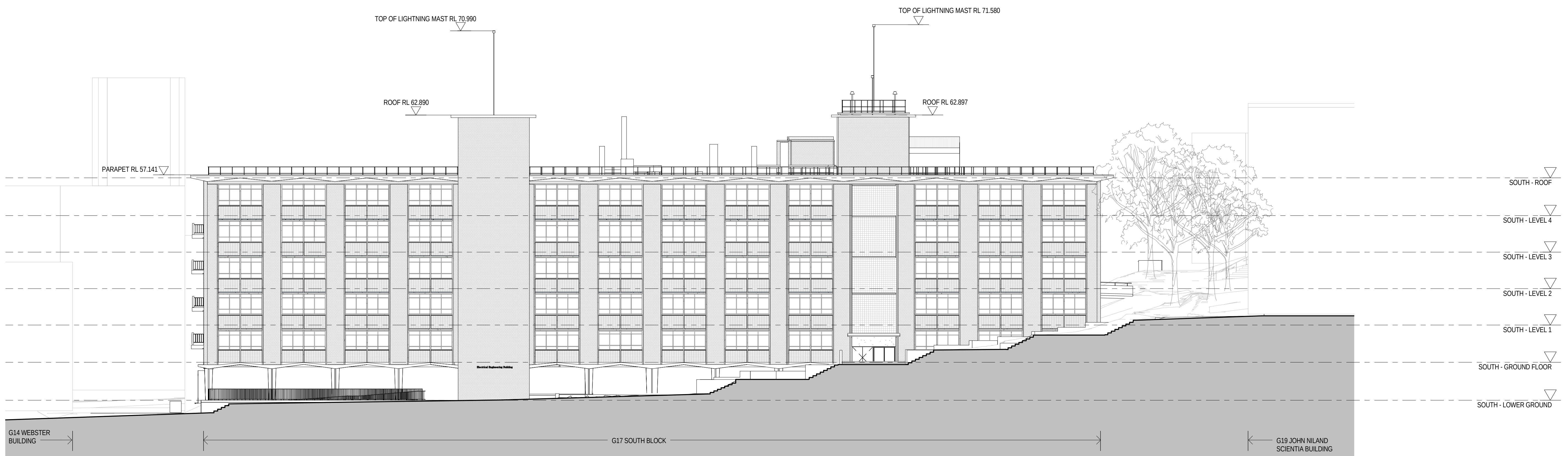
2 EXISTING - ELEVATION - SOUTH A_0201 1:200
