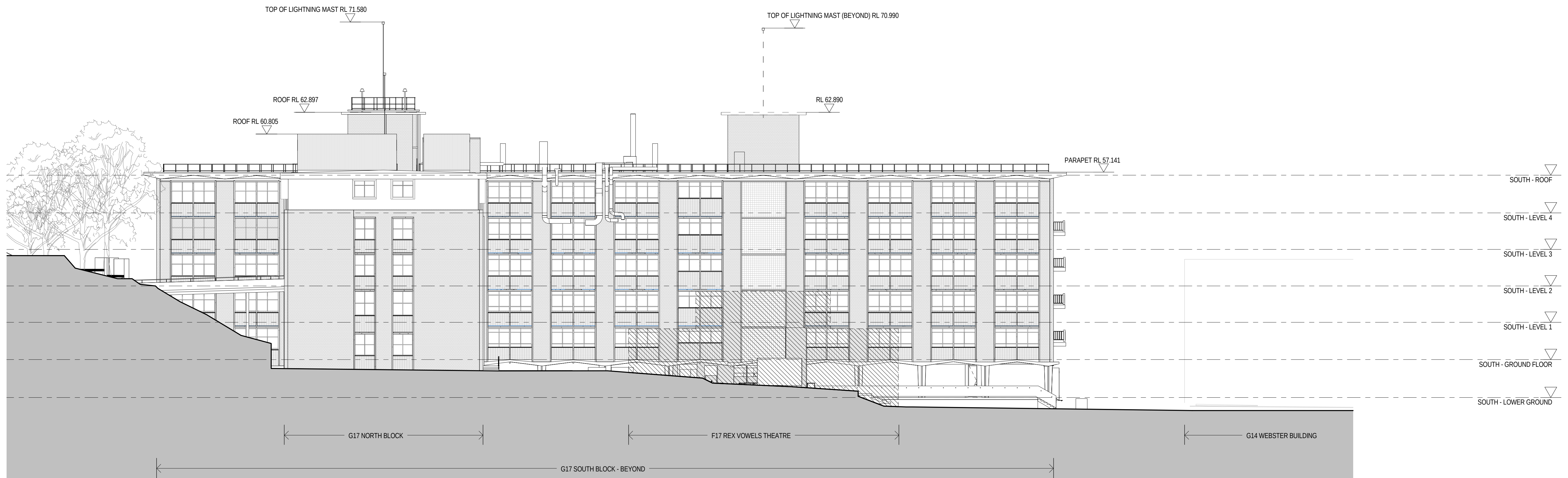
1 EXISTING - ELEVATION - NORTH A_0201 1:200
