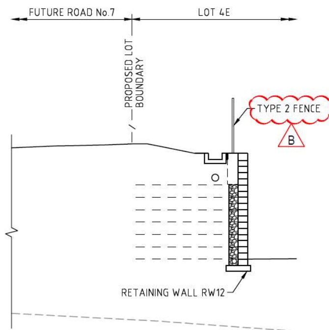
Figure 5 – Typical Section through Retaining Wall – Aside Road
