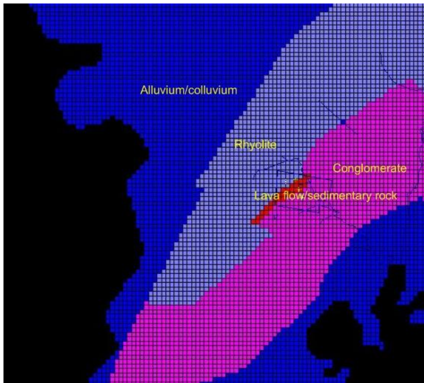
Figure 5 Map of hydraulic conductivity distribution in numerical model (Layer1)
