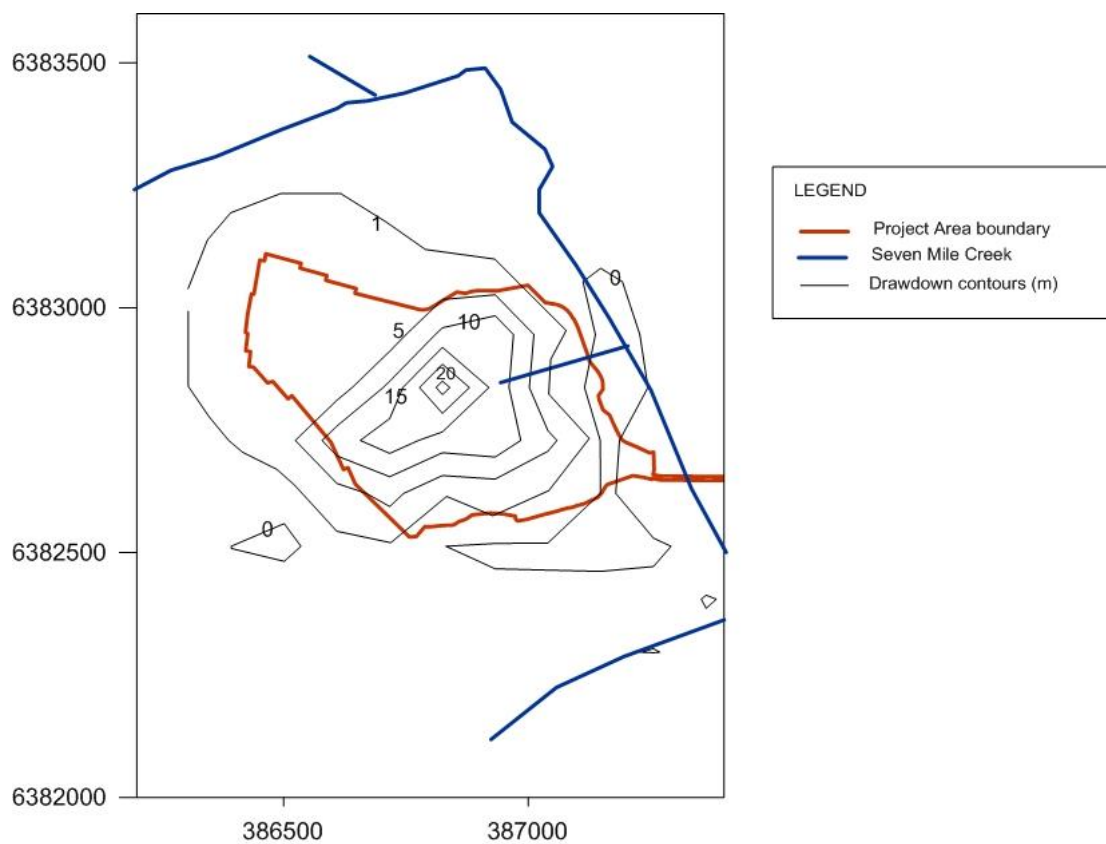
Figure 18 Drawdown in Layer 1 at the end of extraction period
