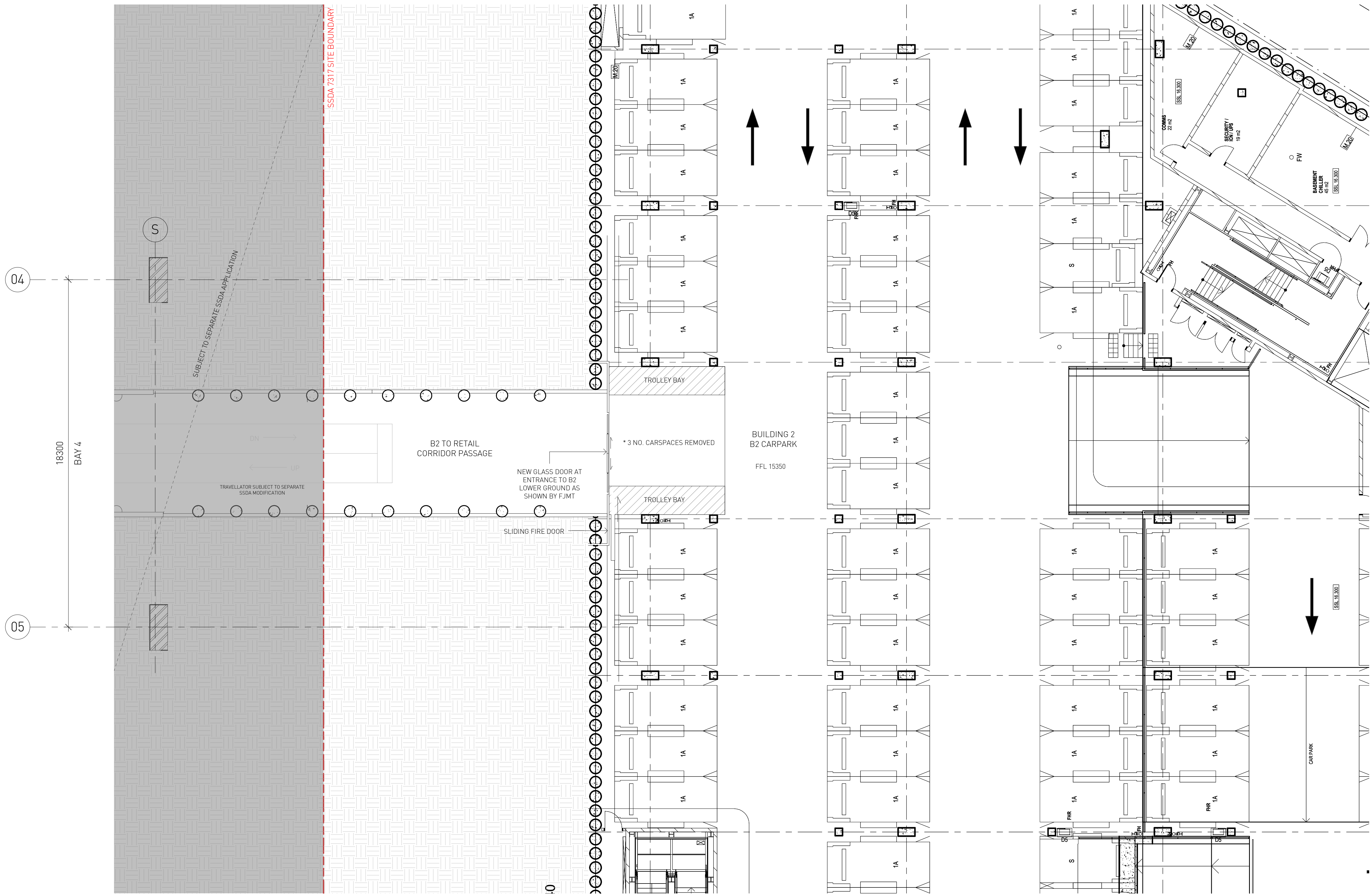
1 TRAVELATOR LINK TO B2 - PLAN 1 : 100
