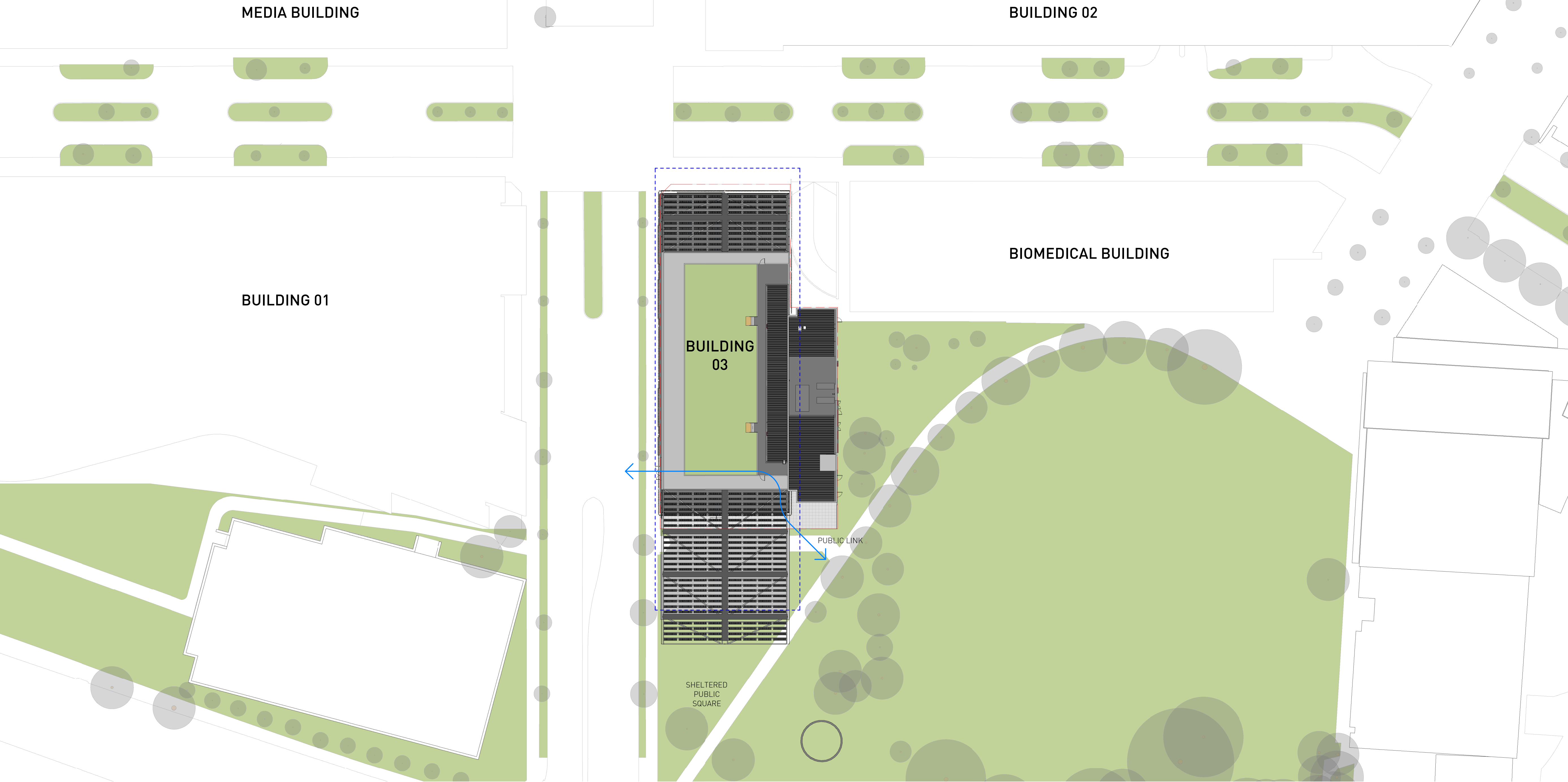
1 SITE PLAN - DA 1 : 400 S96 SUBMISSION
