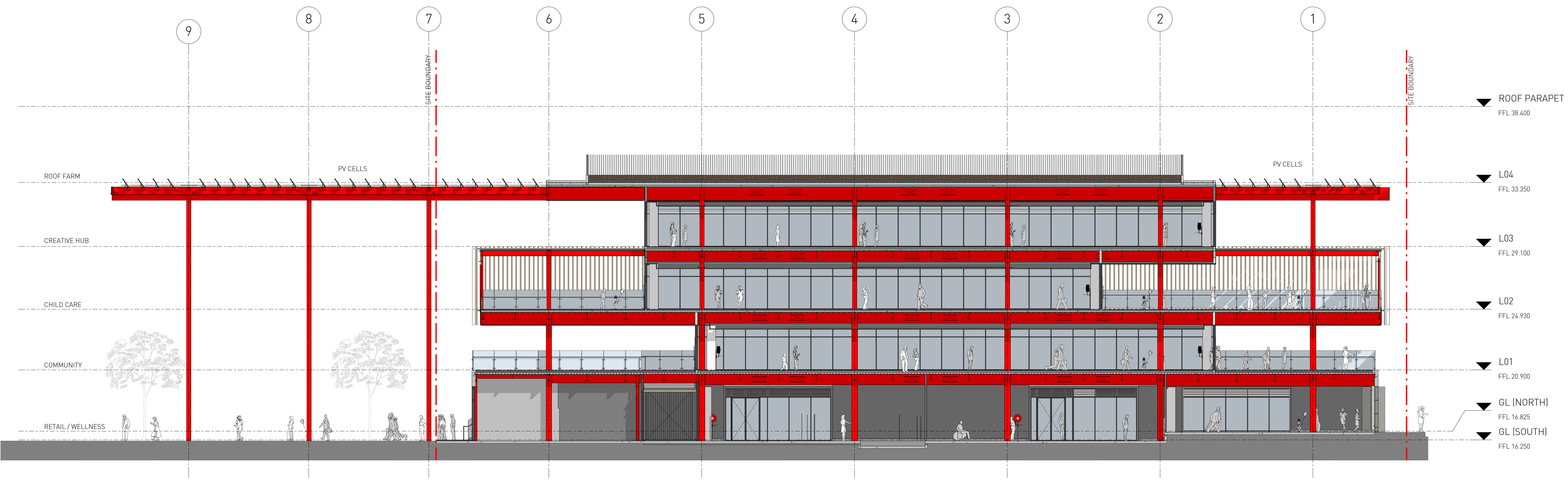
1 DA SECTION A-A (NORTH SOUTH) 1 : 125
