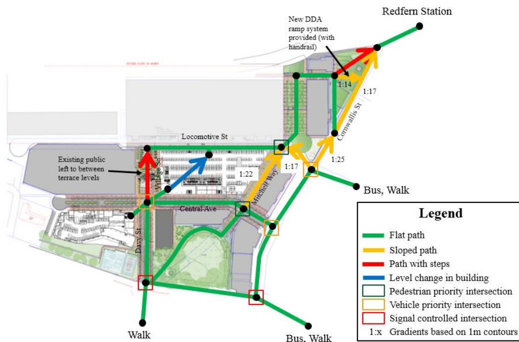
Figure 13 - Pedestrian connectivity and accessibility within site and to external streets
