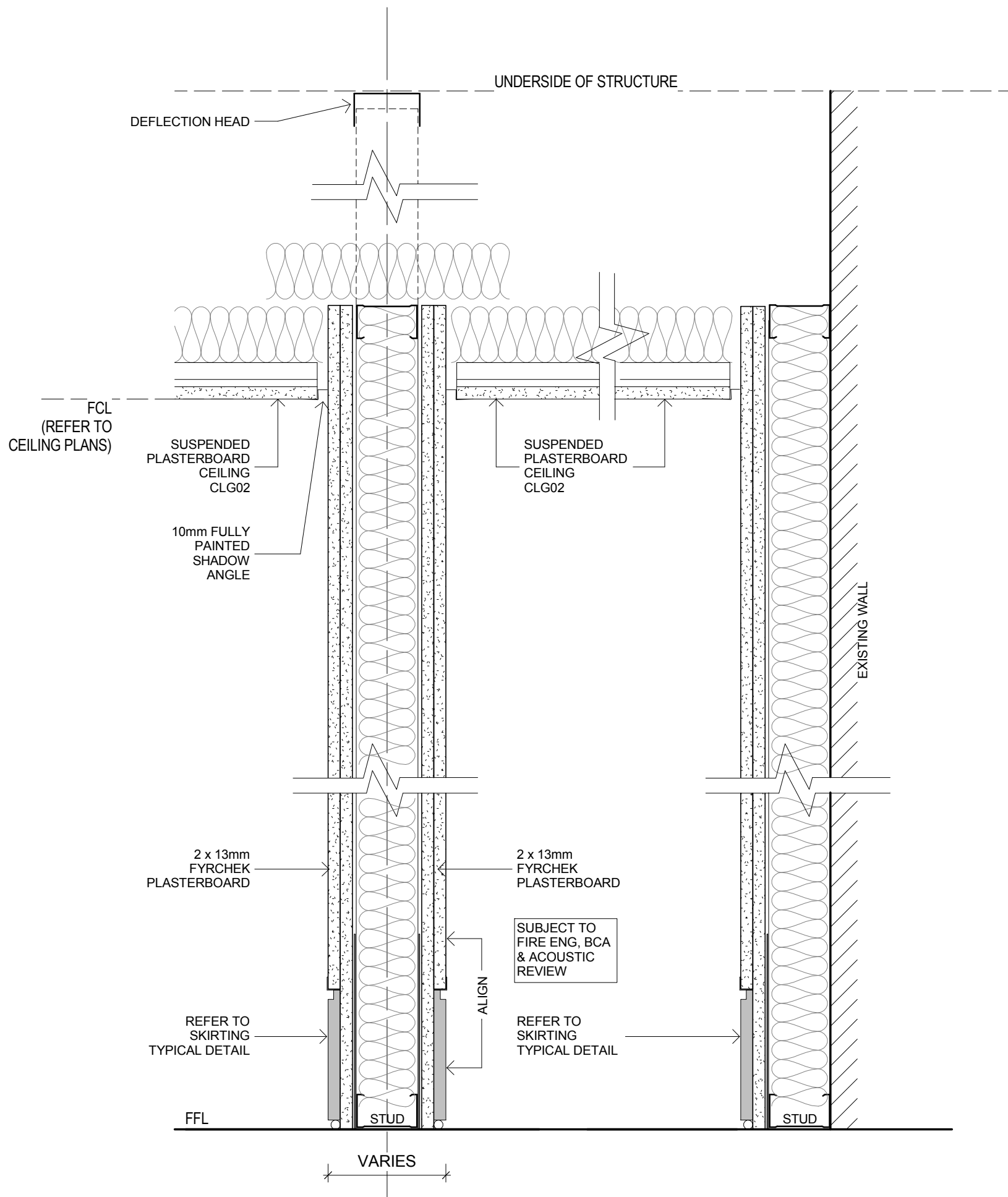
2 PT02-DETAIL SECTION 1:5
