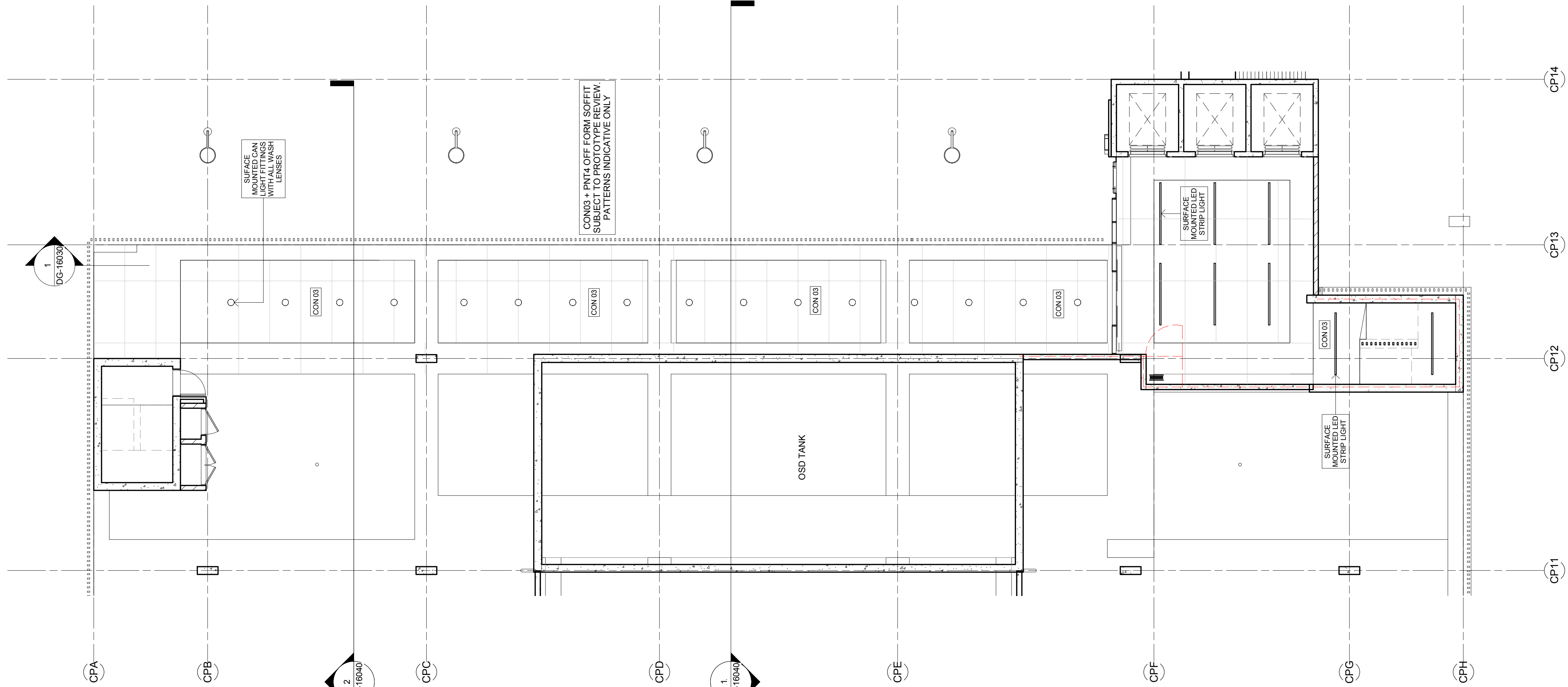
1 RCP - Lower Ground - Walkway 1:100
