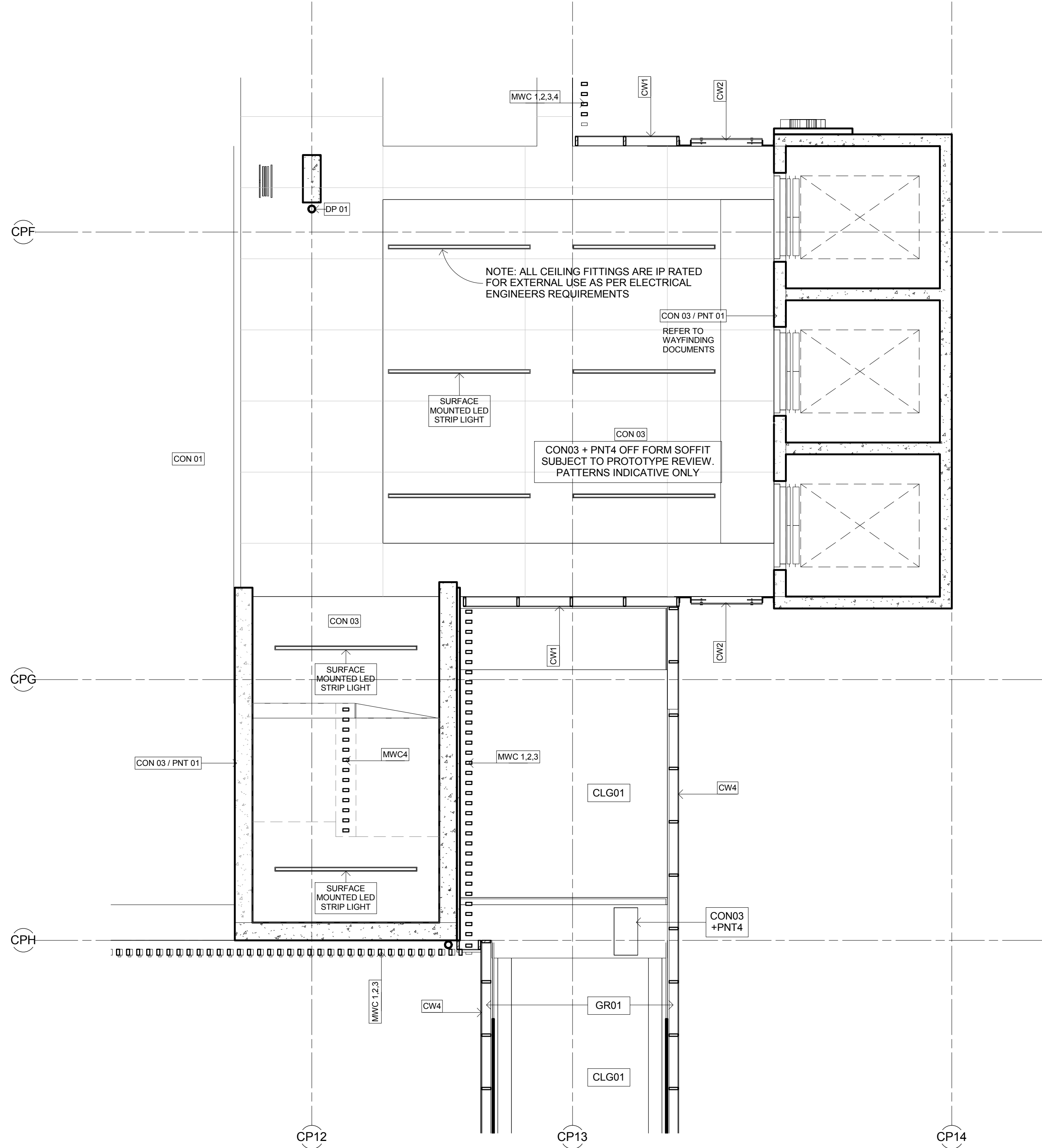
2 Lift Lobby RCP - Level 1 1 : 50
