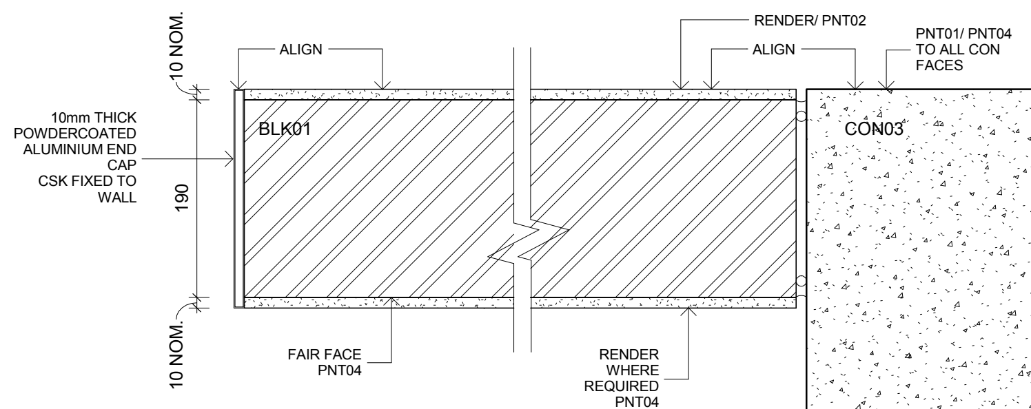
7 RENDERED BLK JUNCTION-PLAN DETAIL 1:5
