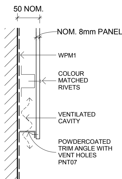
5 CLD01-SECTION DETAIL 1:5
