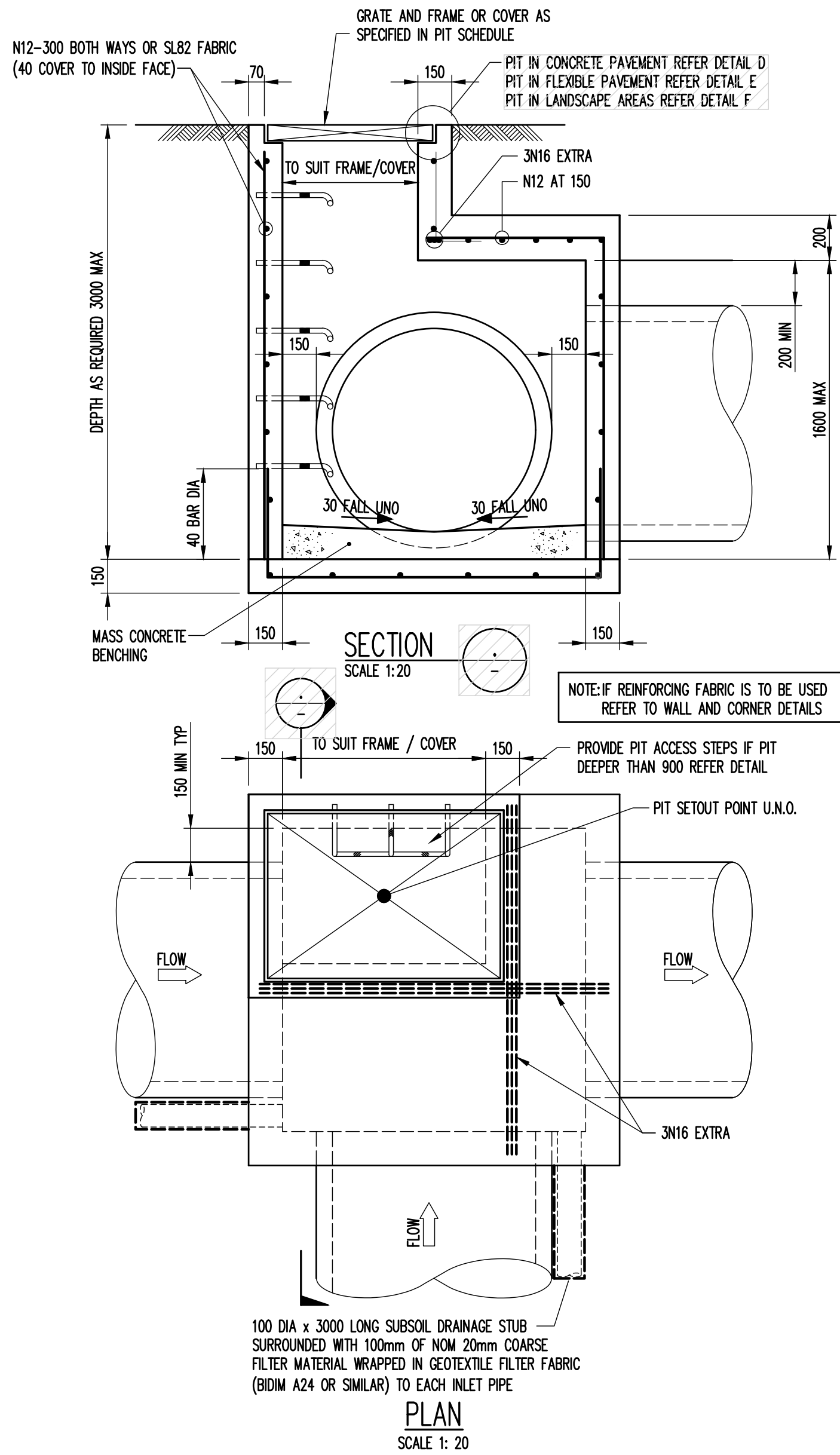
PIT TYPE A
