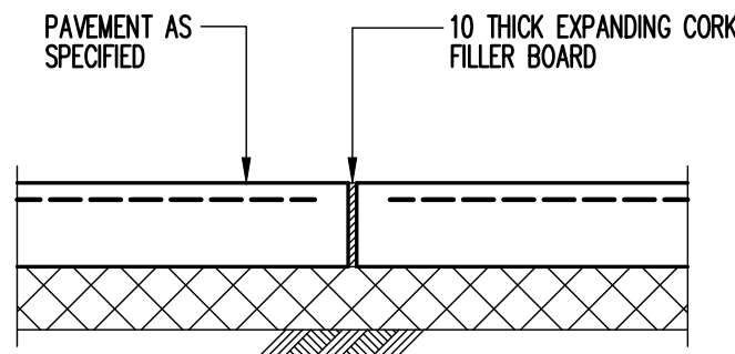
EXPANSION JOINT (EJ) SCALE 1:20
