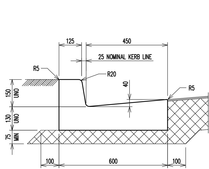
KERB AND GUTTER (K&G) SCALE 1:10
