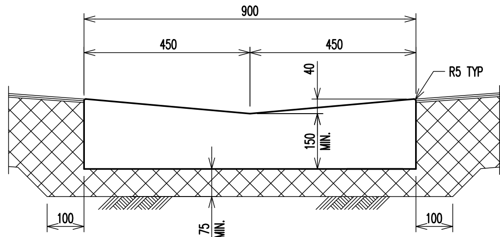
DISH DRAIN (DD) SCALE 1:10
