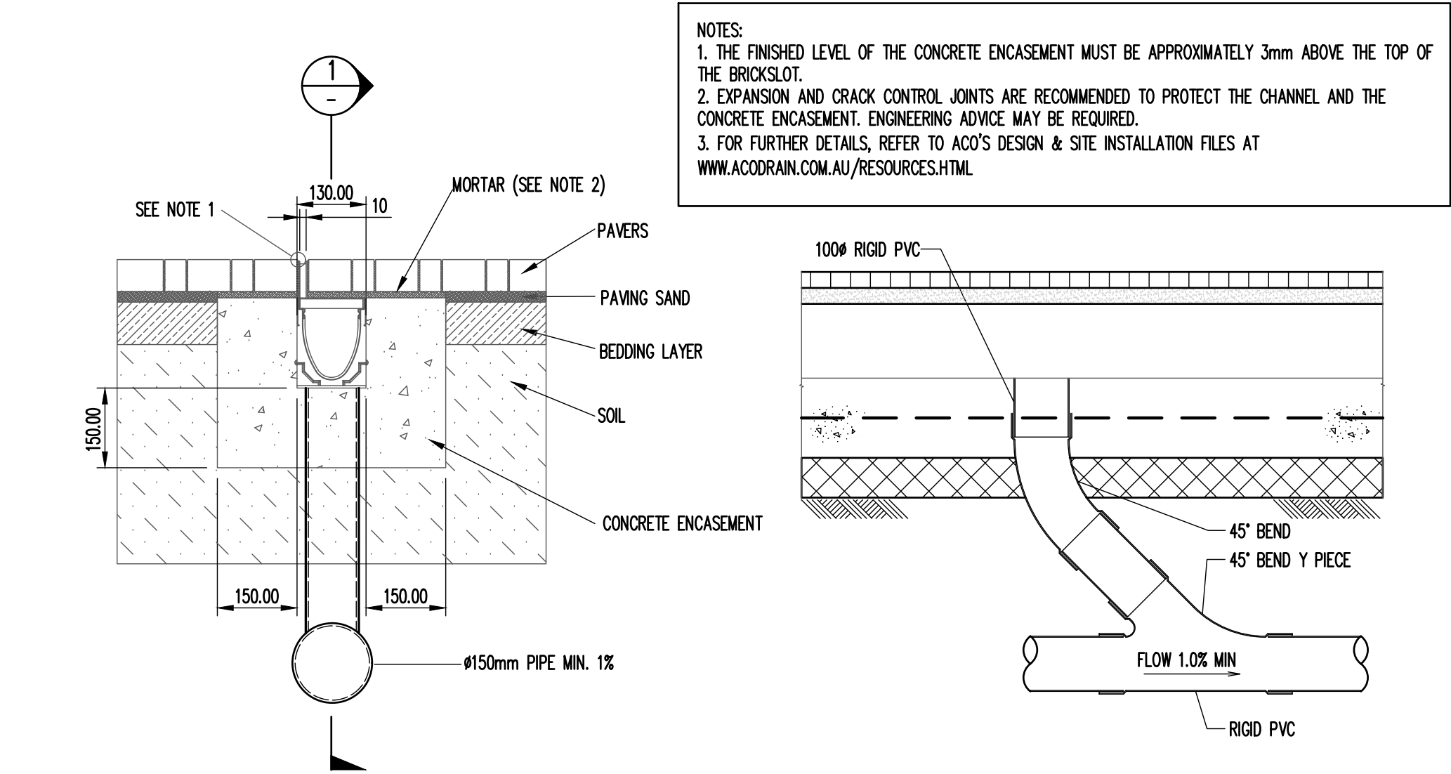
SLOT DRAIN IN PAVERS
