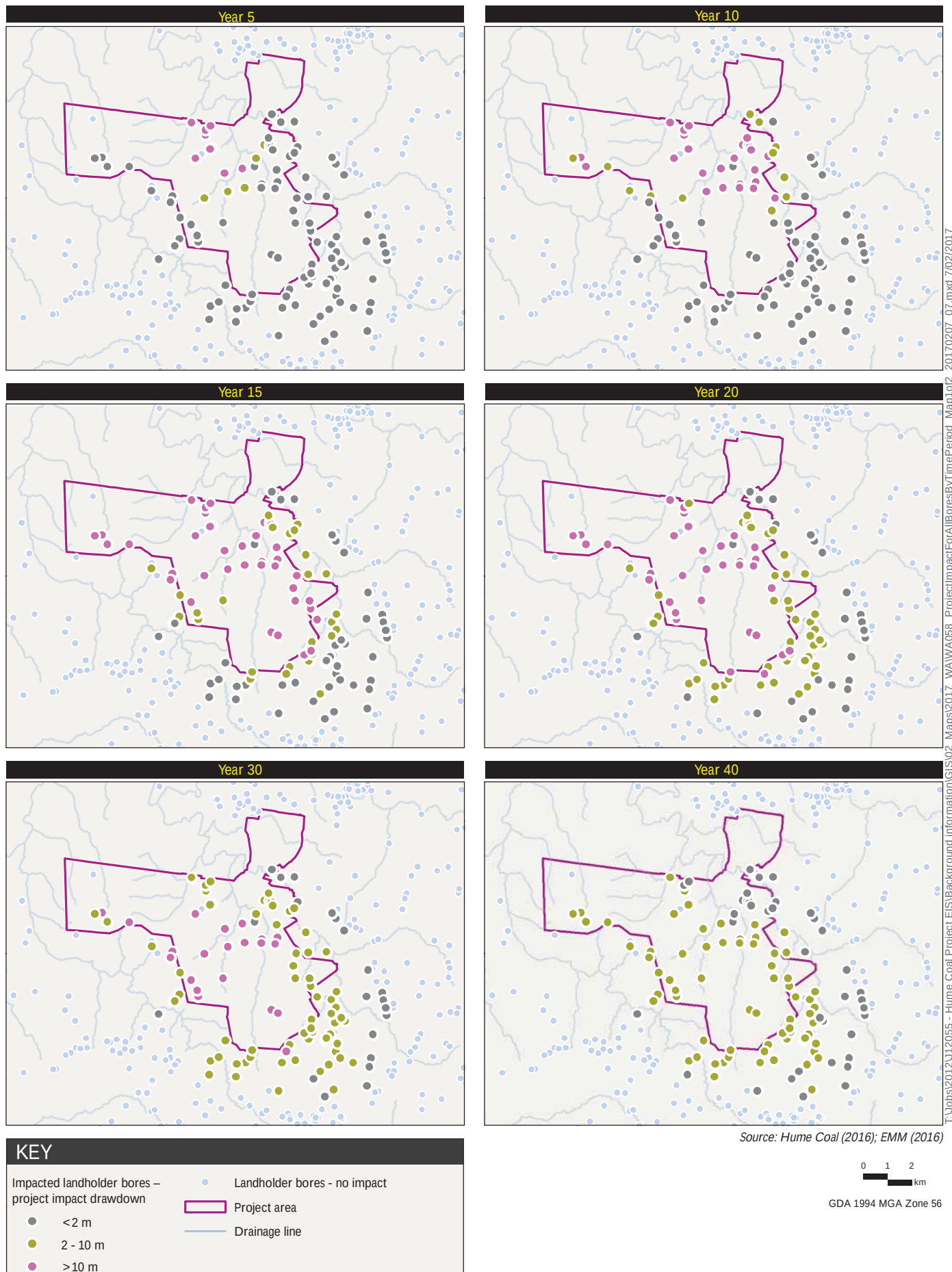
Project drawdown at landholder bores, at selected years since commencement of mining Hume Coal Project Water Assessment Figure N.1a
