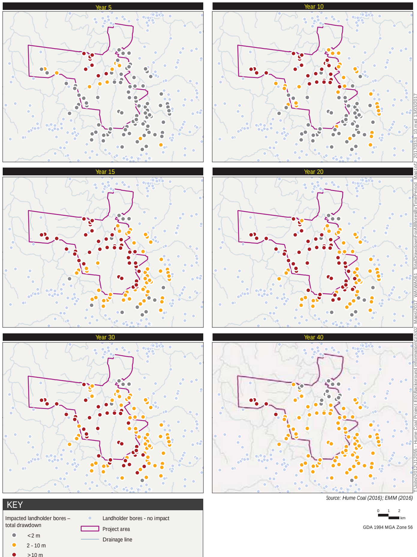
Total drawdown at landholder bores, at selected years since commencement of mining Hume Coal Project Water Assessment Figure N.2a
