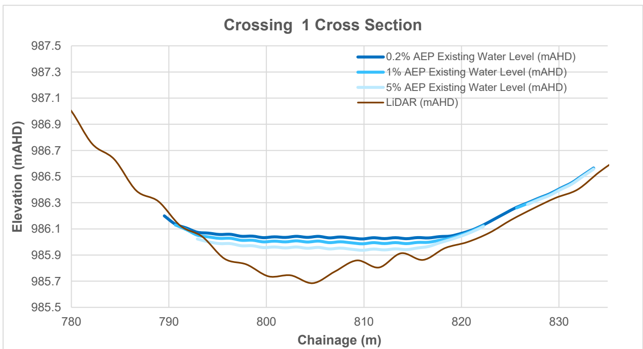
Figure 4-3 Crossing 1 Cross Section
