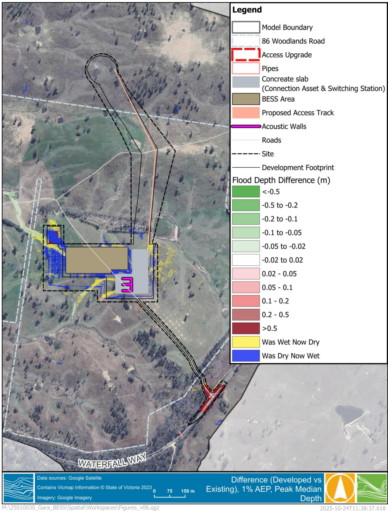
Figure 3-7 Change in 1% AEP peak depth
