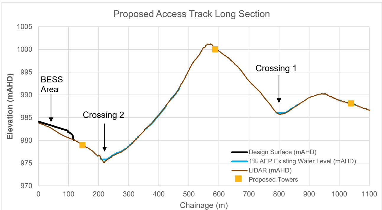
Figure 4-2 Proposed access track long section
