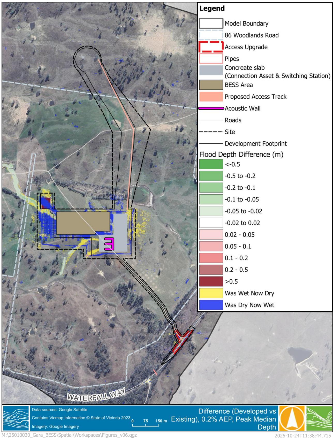
Figure C 4 Design Conditions – 0.2% AEP depth-difference
