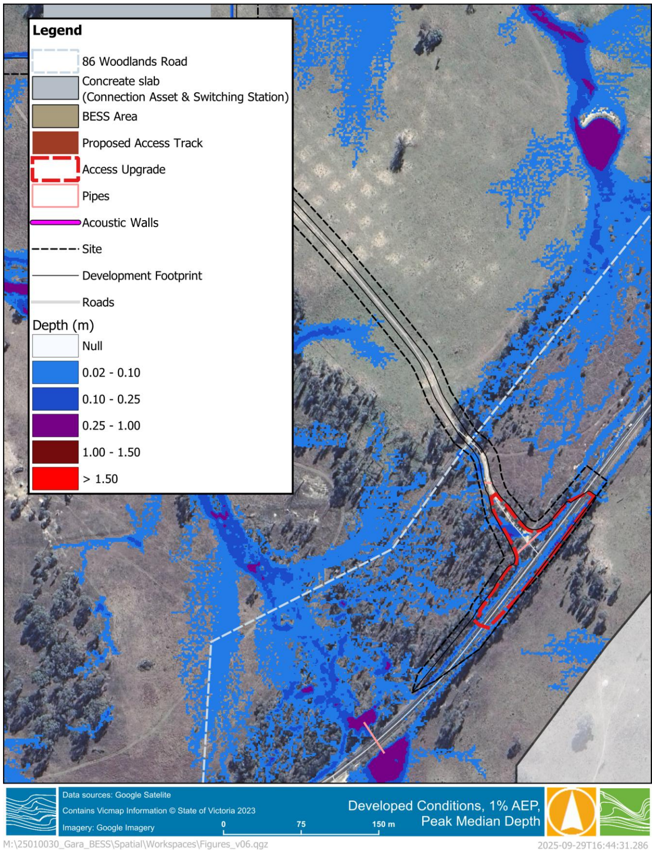
Figure 3-10 Developed Conditions 1% AEP Peak Depth at the Access Upgrade
