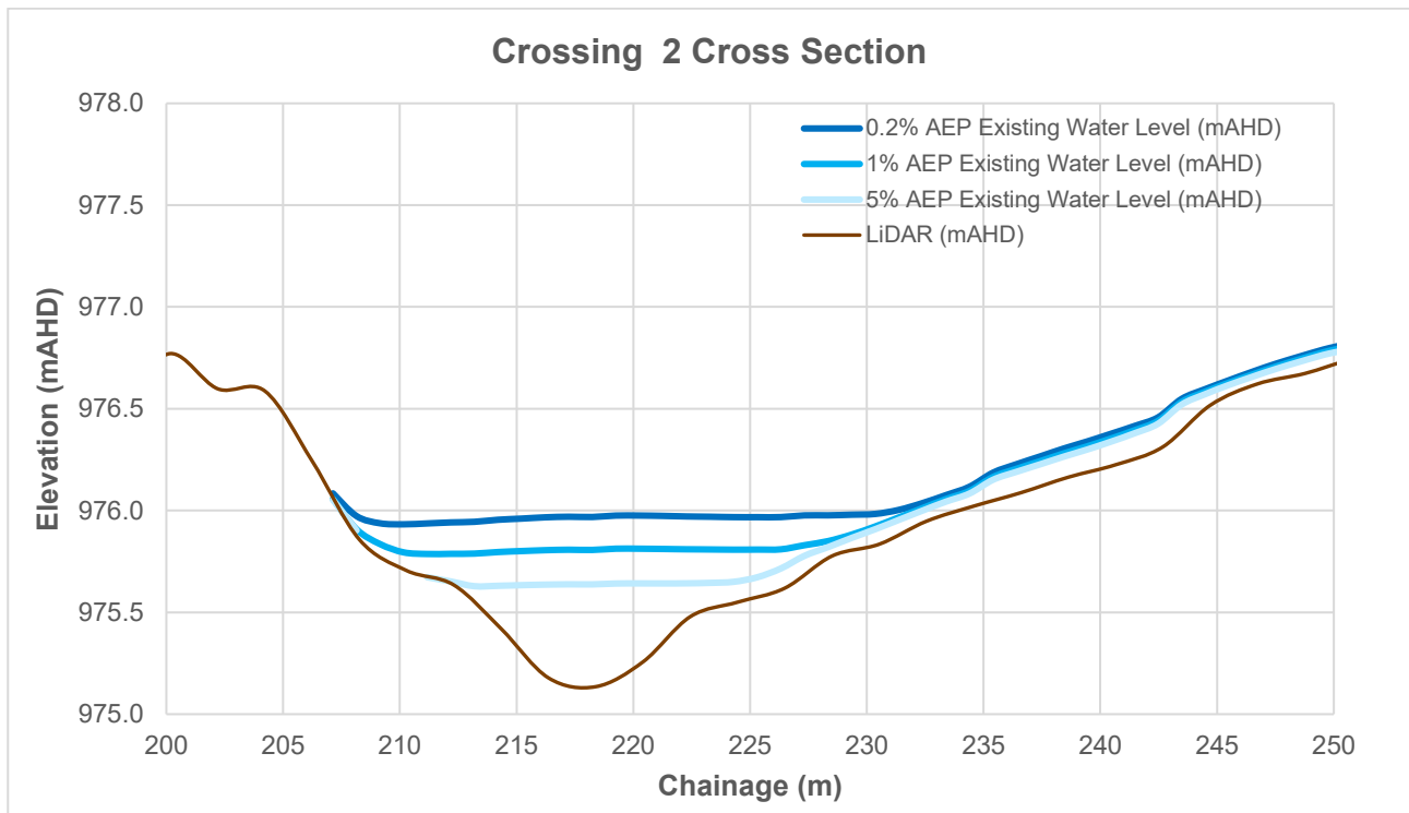
Figure 4-4 Crossing 2 Cross Section
