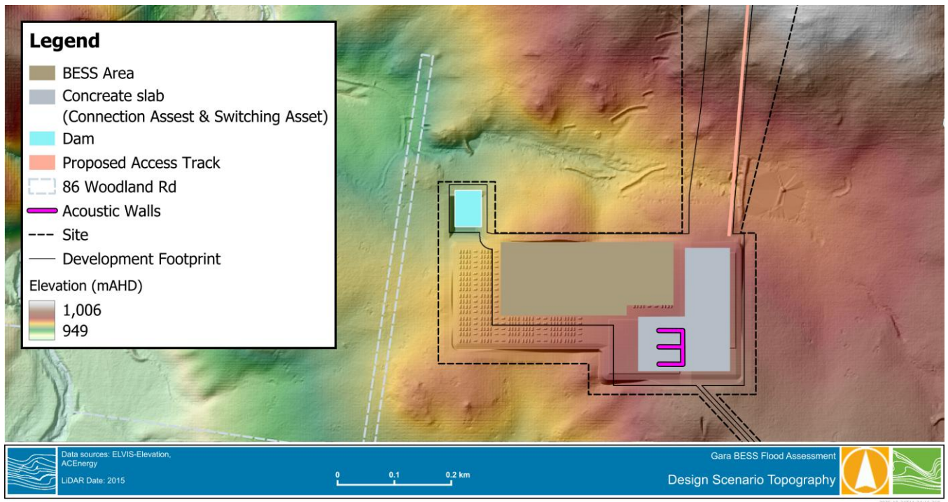
Figure 2-6 Design Scenario Topography
