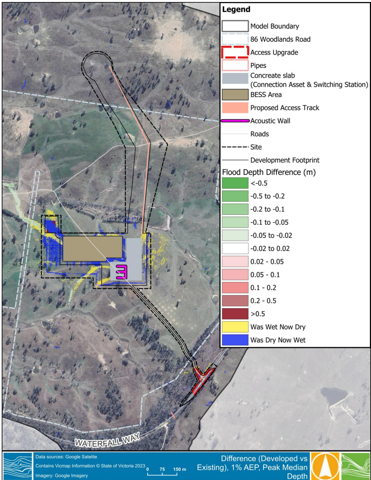
Figure C 2 Design Conditions – 1% AEP depth-difference
