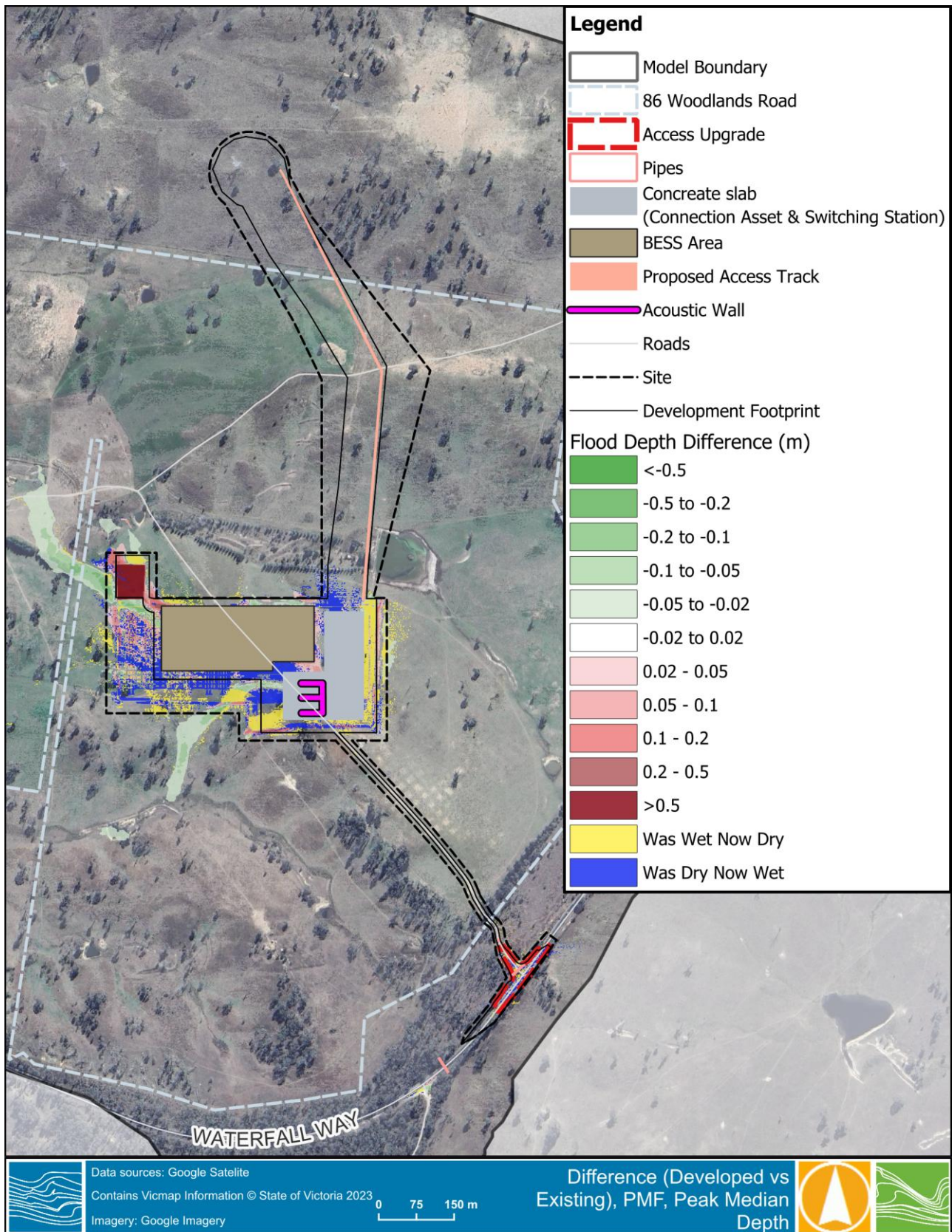
Figure C 5 Design Conditions – PMF depth-difference
