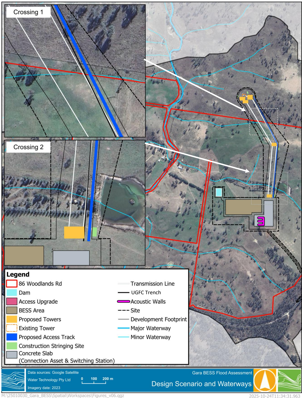
Figure 4-1 Defined waterways at the site with proposed crossings marked
