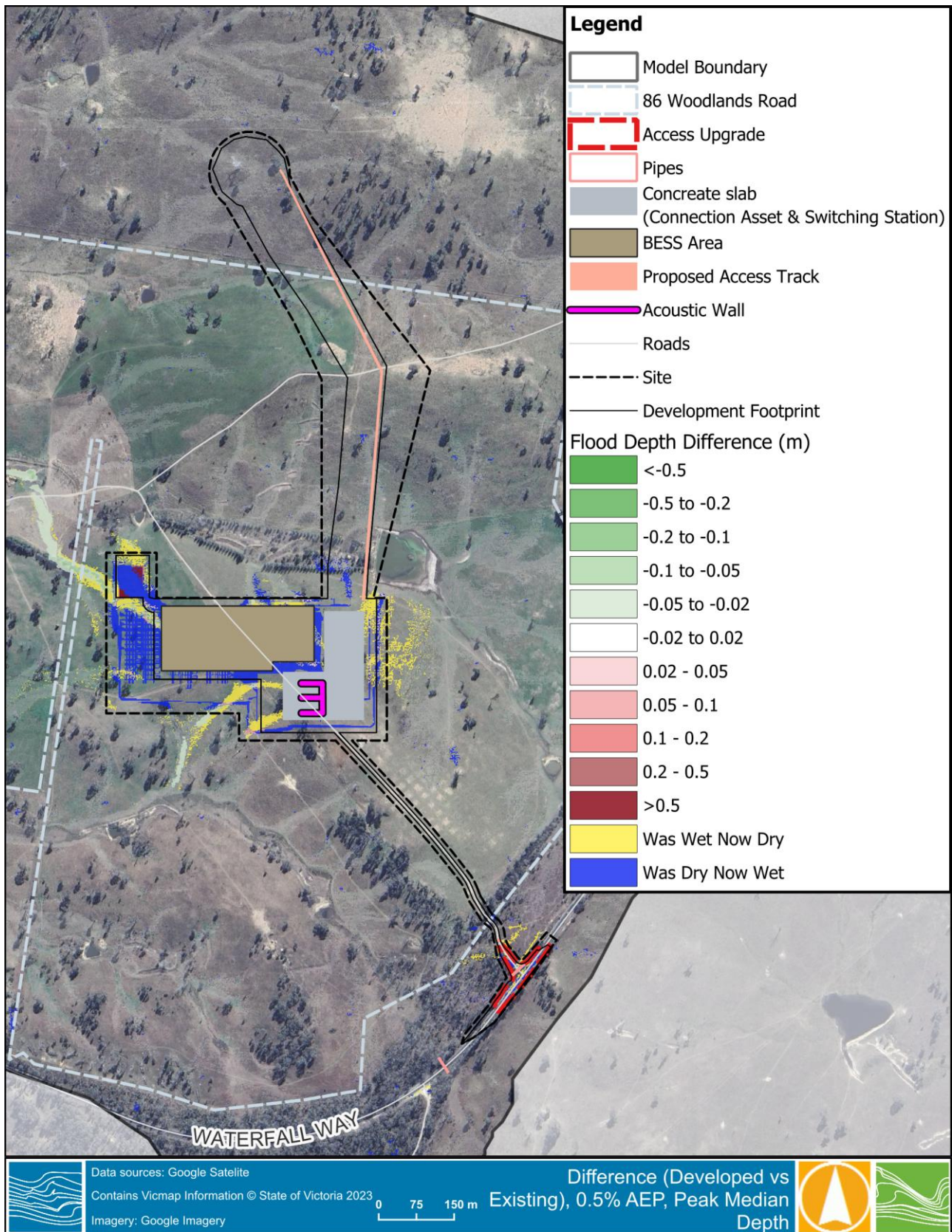
Figure C 3 Design Conditions – 0.5% AEP depth-difference
