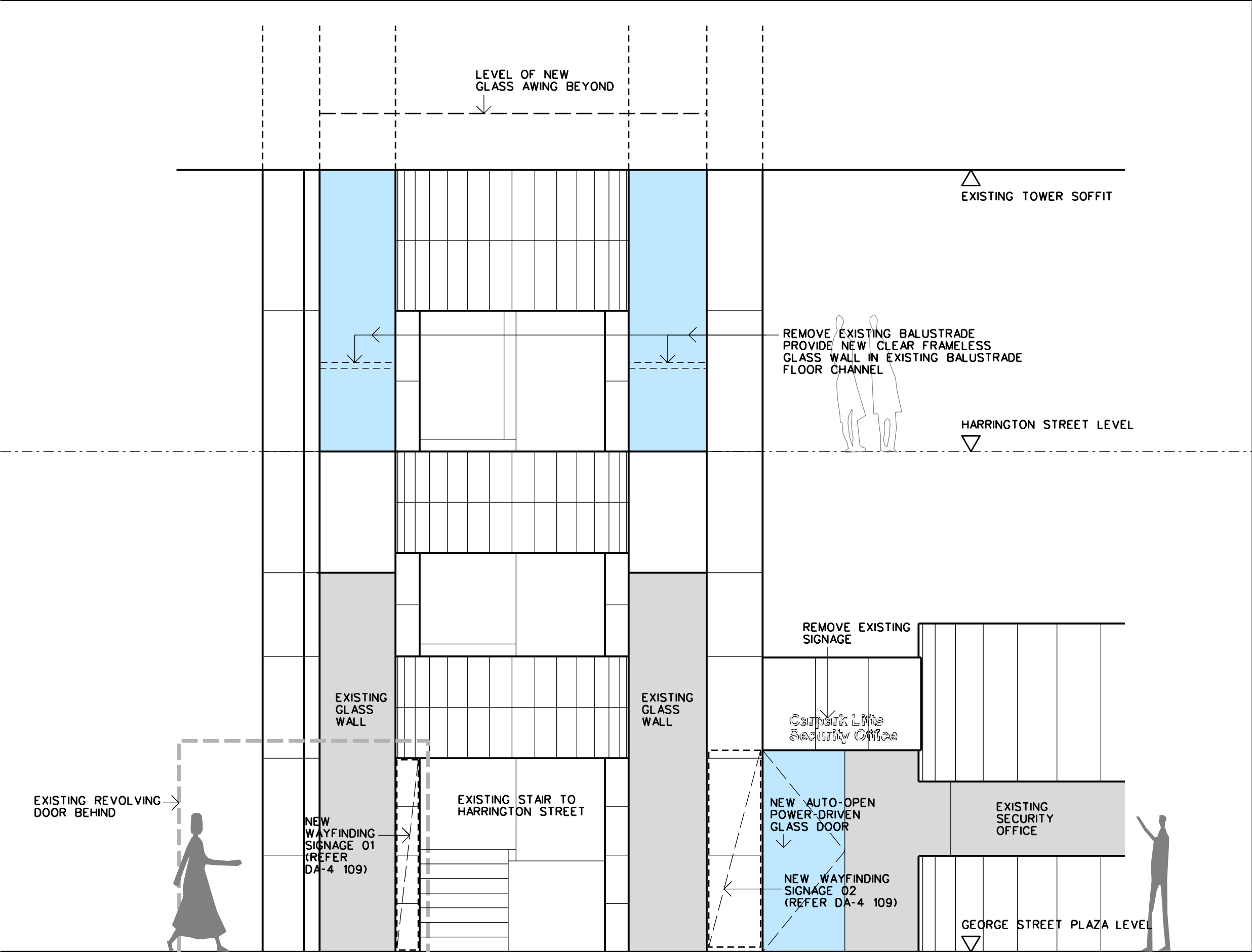
DEVELOPED ELEVATION
