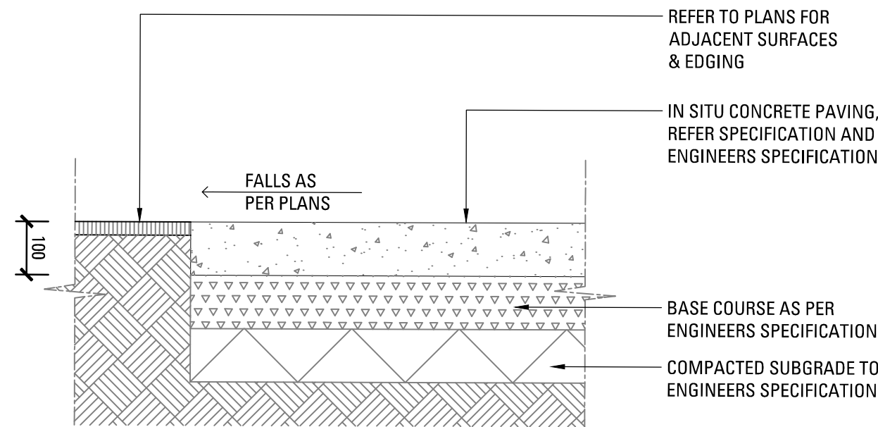
00 INSITU CONCRETE PAVING SCALE 1:10
