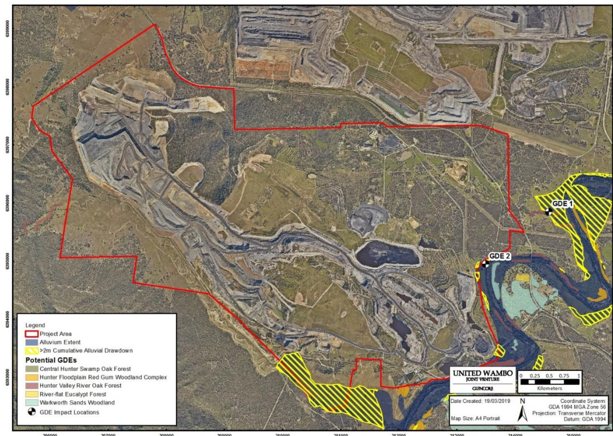
Figure 5-4: Groundwater Dependent Ecosystems
