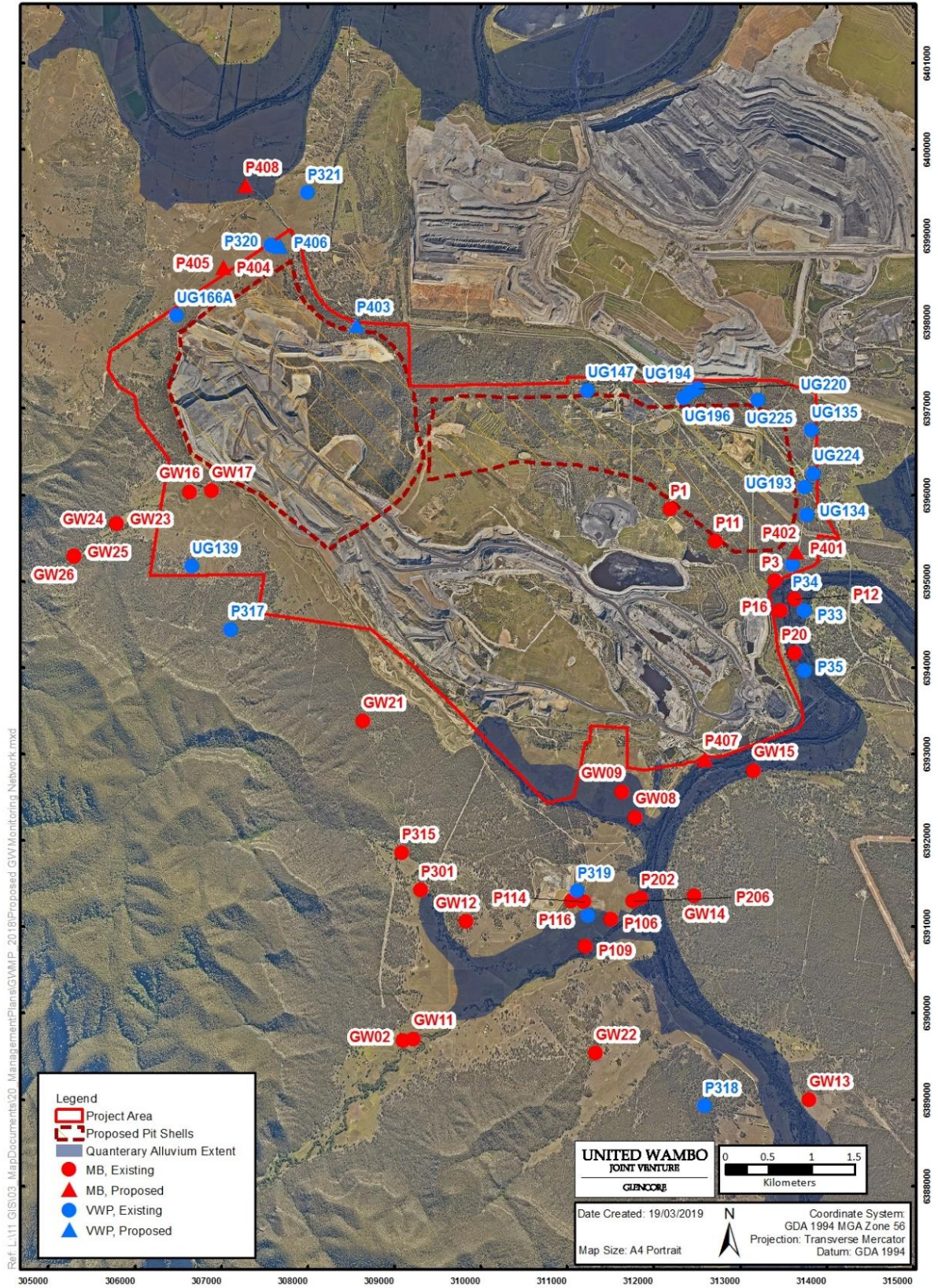
Figure 7-1: Groundwater Monitoring Network
