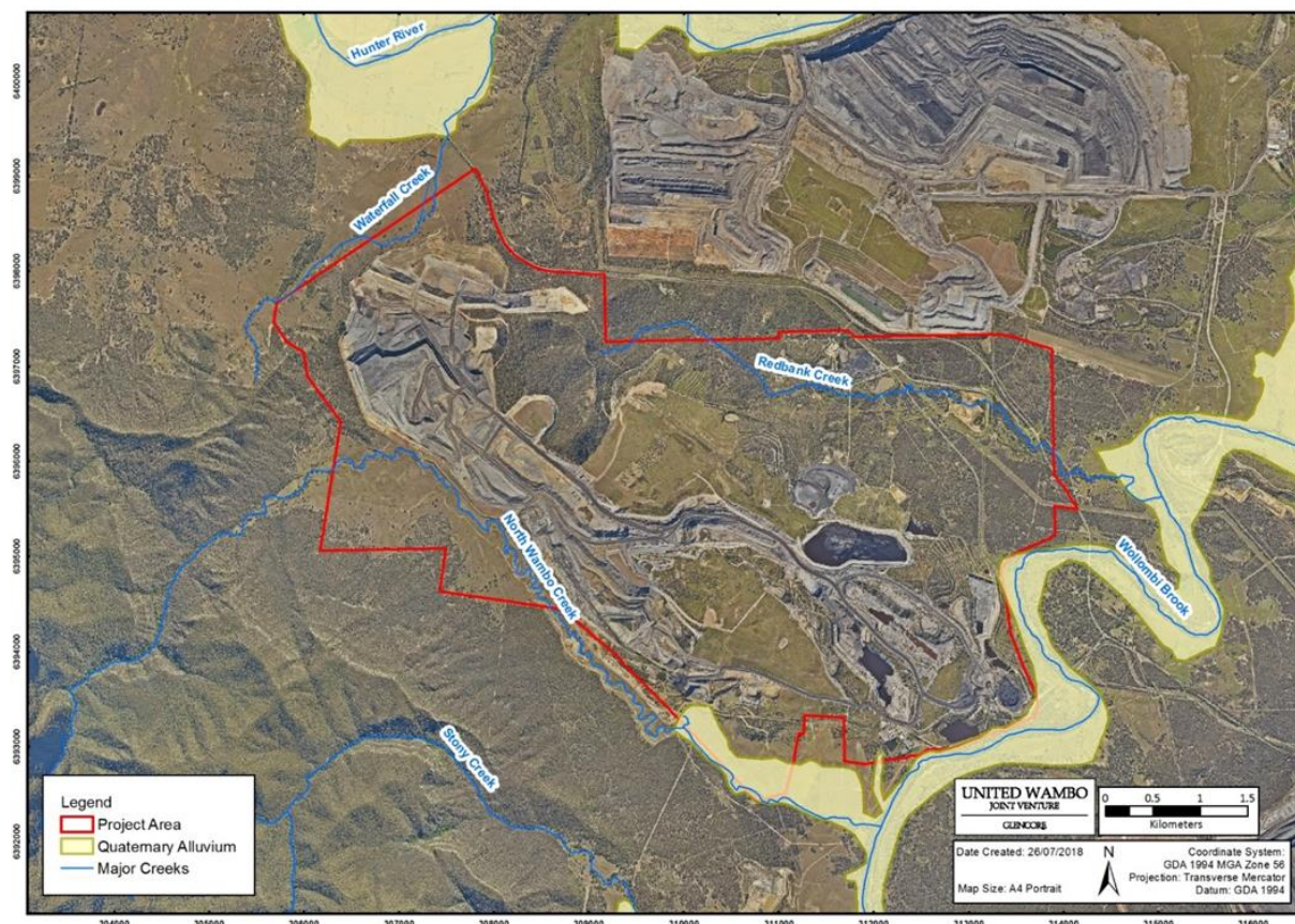
Figure 5-2: Quaternary Alluvium
