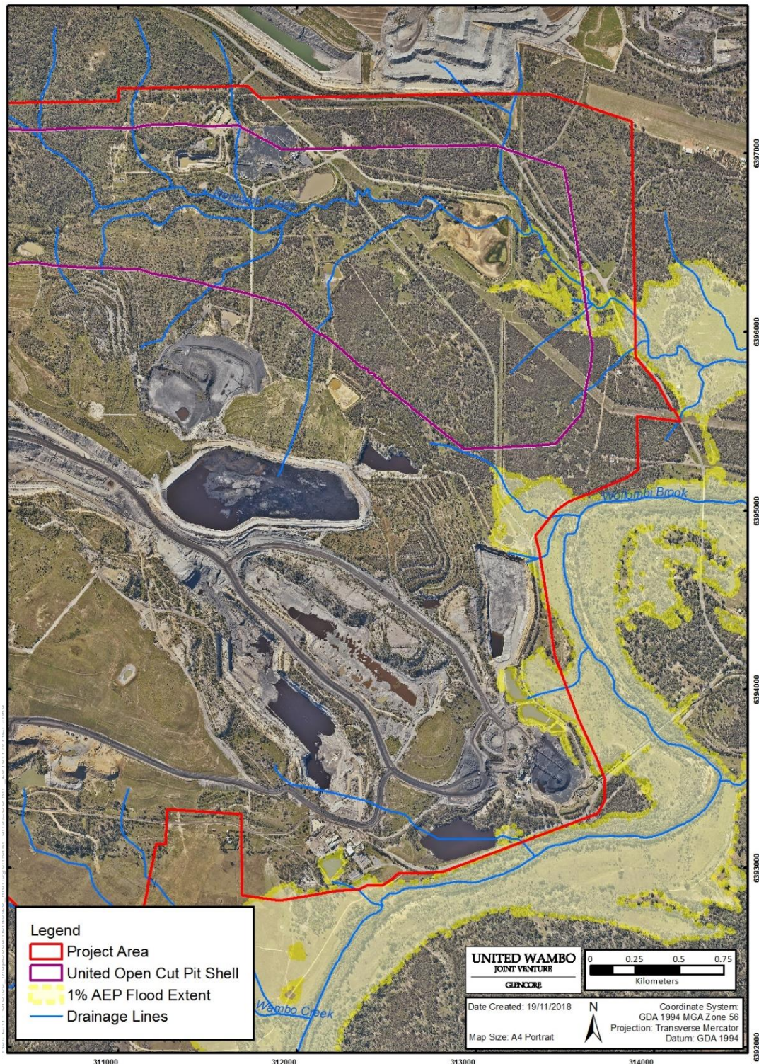
Figure 8-1: 1% AEP Flood Extent
