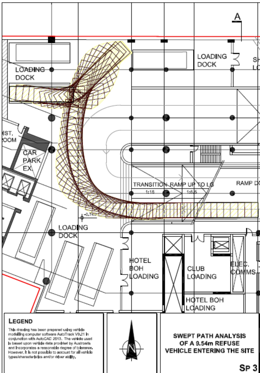
Figure 3: Swept path analysis showing Ingress for waste and recycling collection vehicle at residential and commercial loading dock
