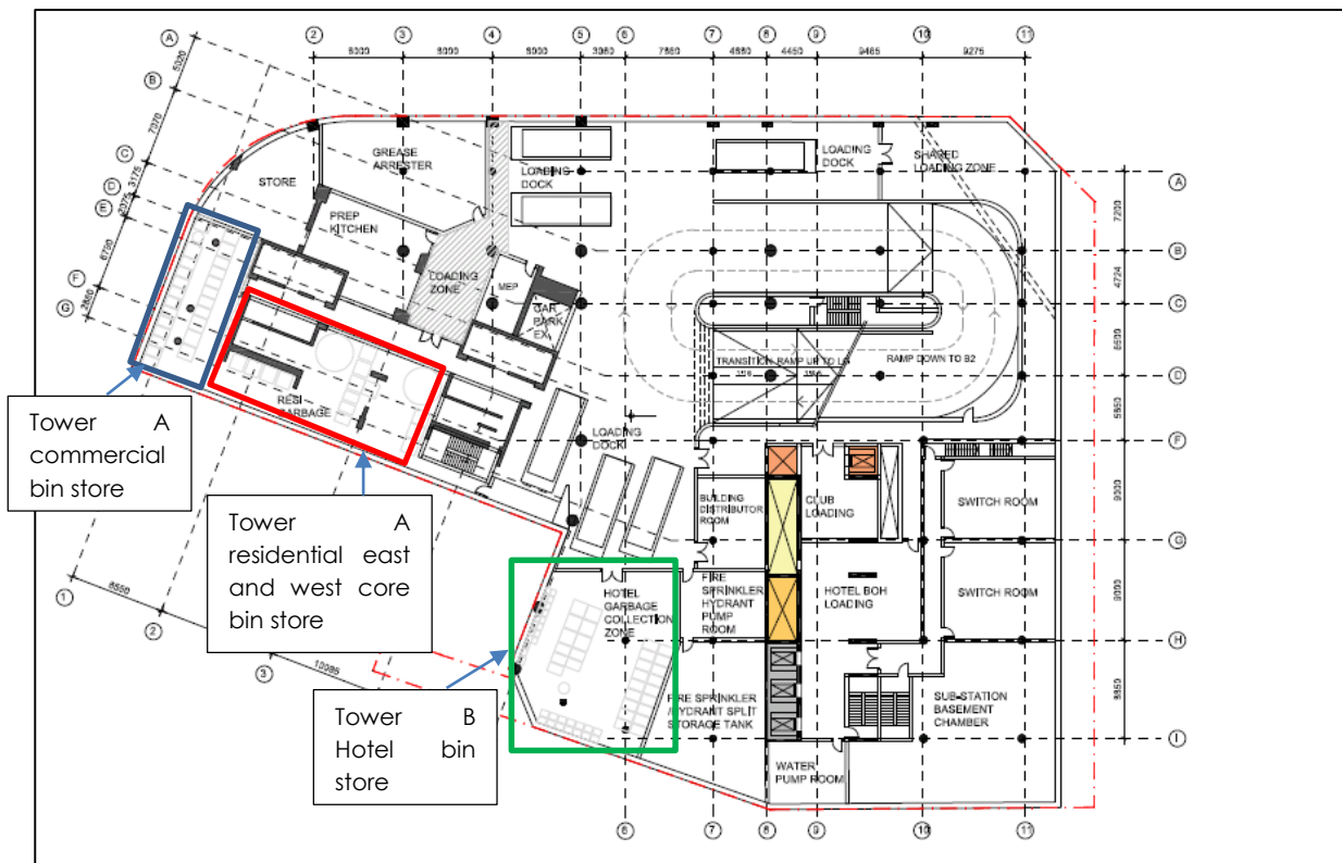
Figure 1: Basement level 1 floor plan showing the three bin stores
