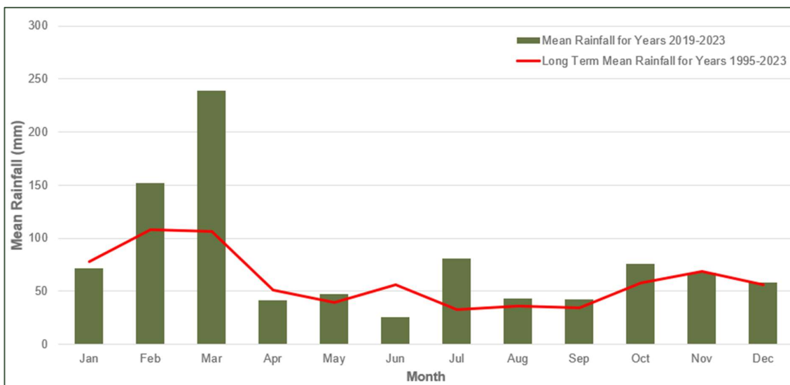
Figure 9 Long term Mean Rainfall for Badgerys Creek AWS – 1995 to 2023
