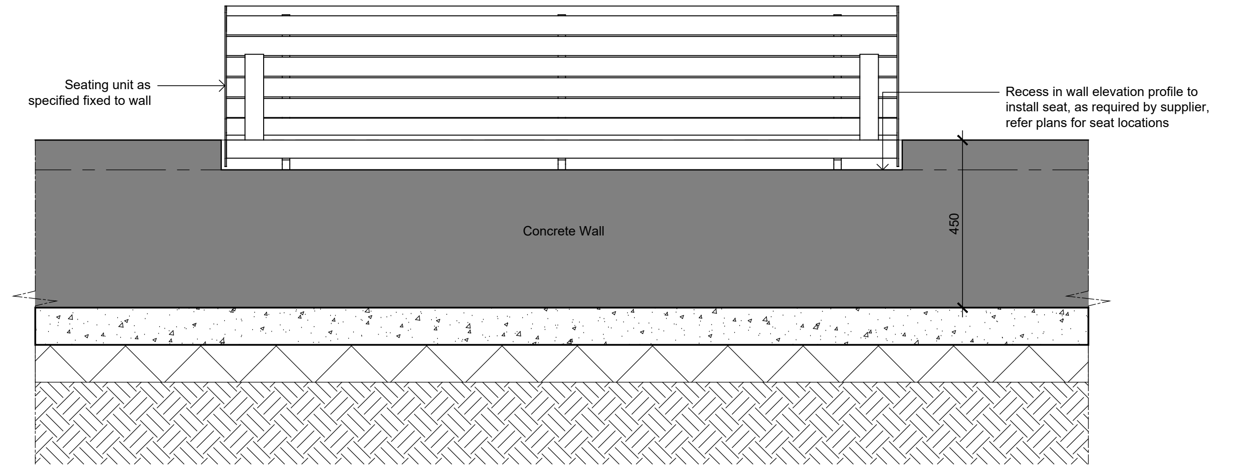
Typical Elevation - Wall Mounted Seat with Backrest and Armrest 1:10
