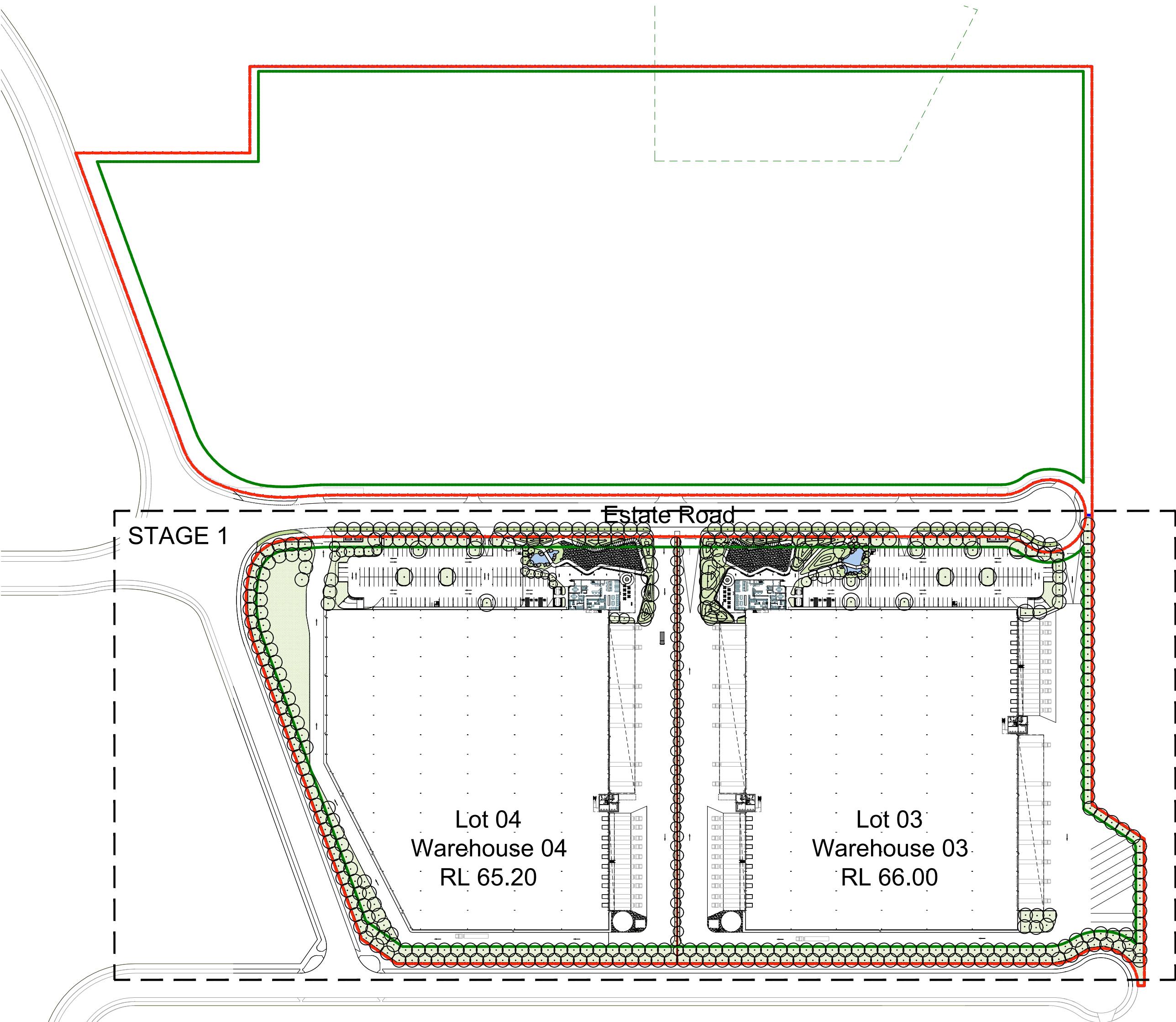
Site Plan | 1:2000
