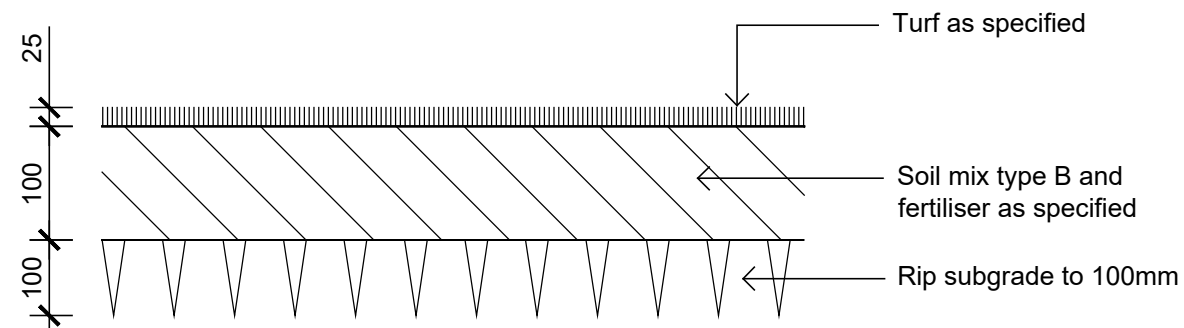
03 Detail Turf on Even Grade
