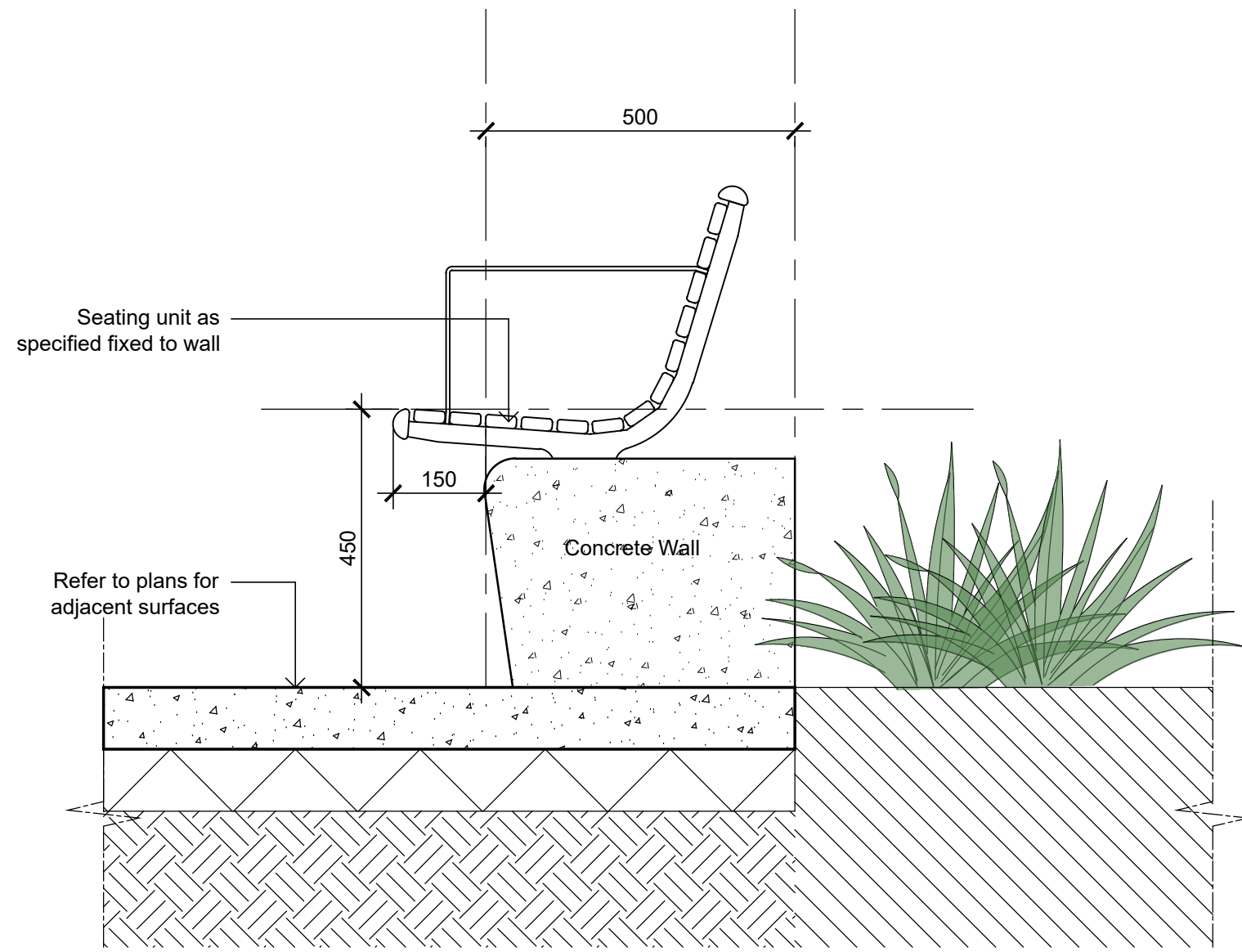
Wall Mounted Seat with Backrest and Armrest 1:10
