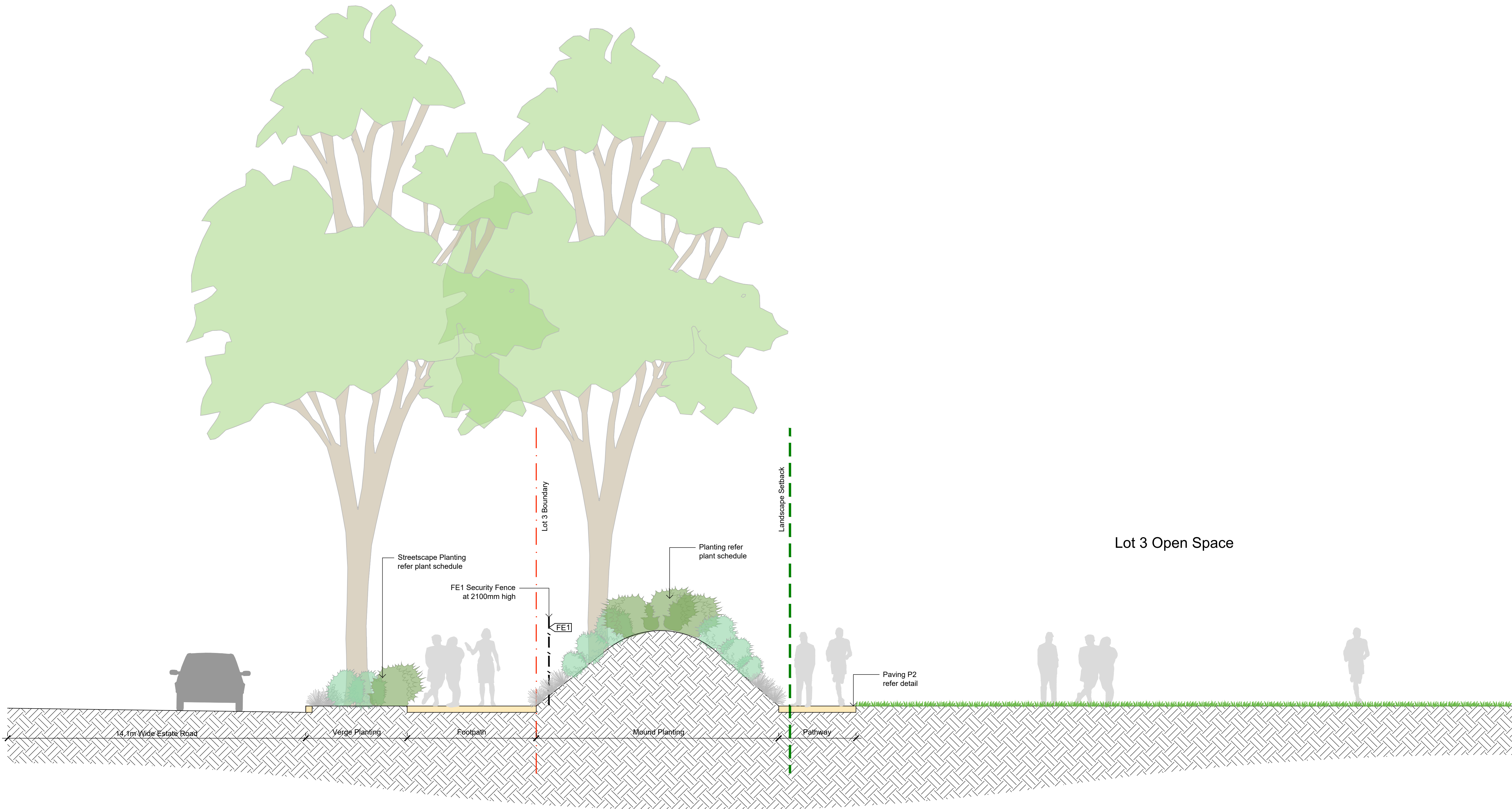
01 Section - Lot 3 Communal Open Space 1:50
