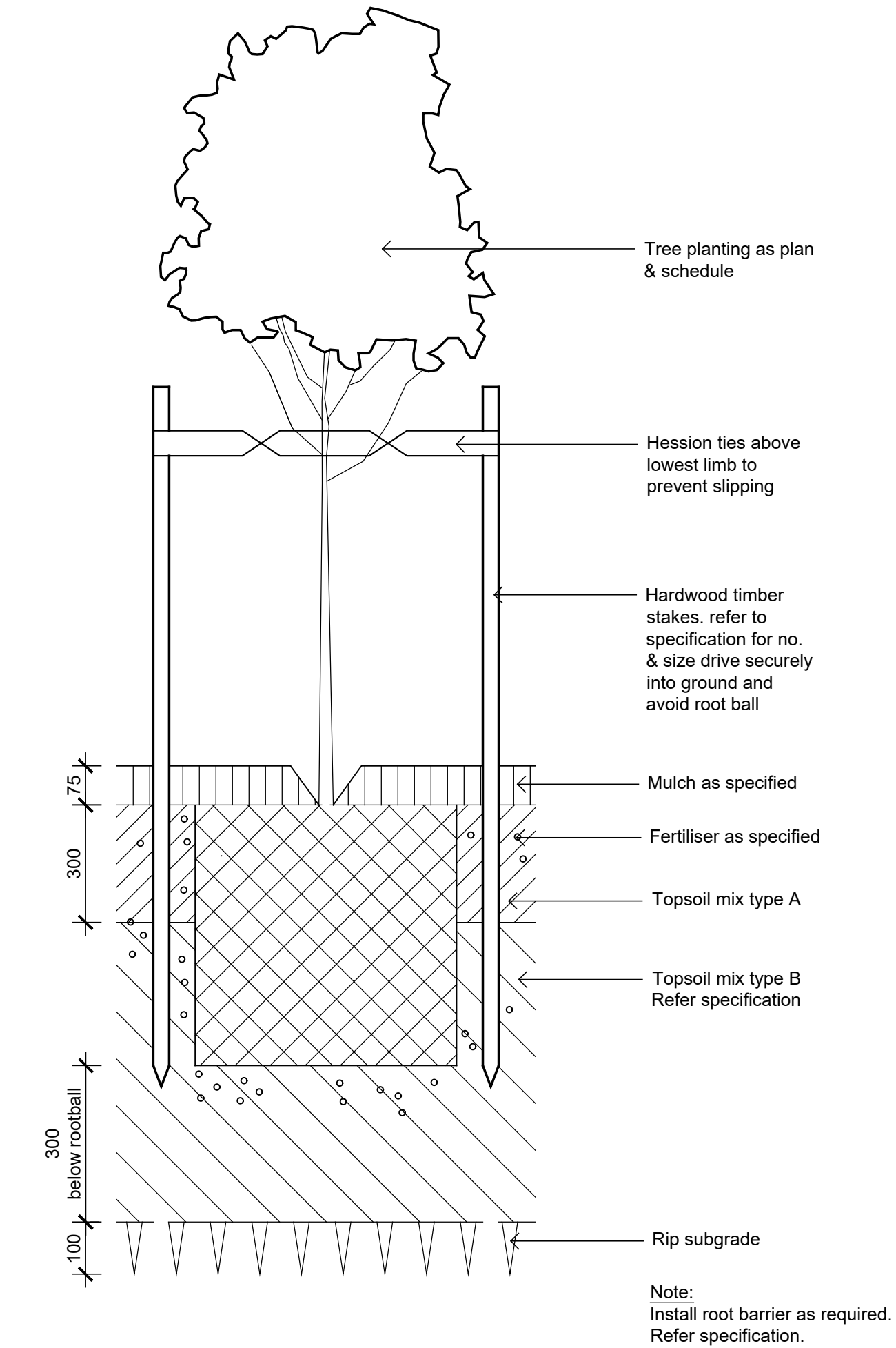
01 Detail 75-200L Tree Planting on Grade
