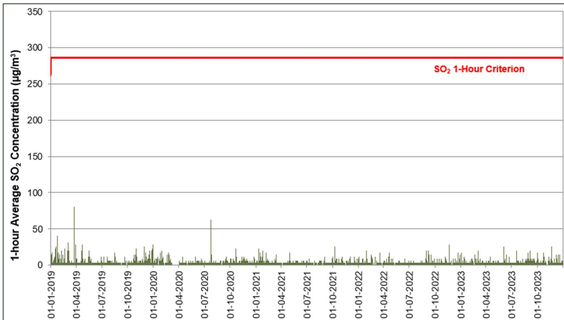
Figure 15 Measured Daily Maximum 1-Hour Average SO 2 Concentrations at Bringelly AQMS (2019-2023)
