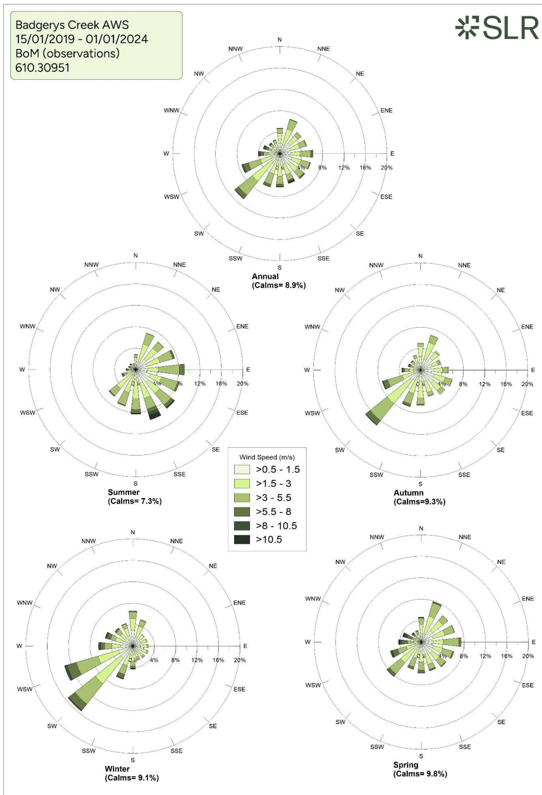
Figure 11 Annual and Seasonal Wind Roses – Badgerys Creek AWS (2019-2023)
