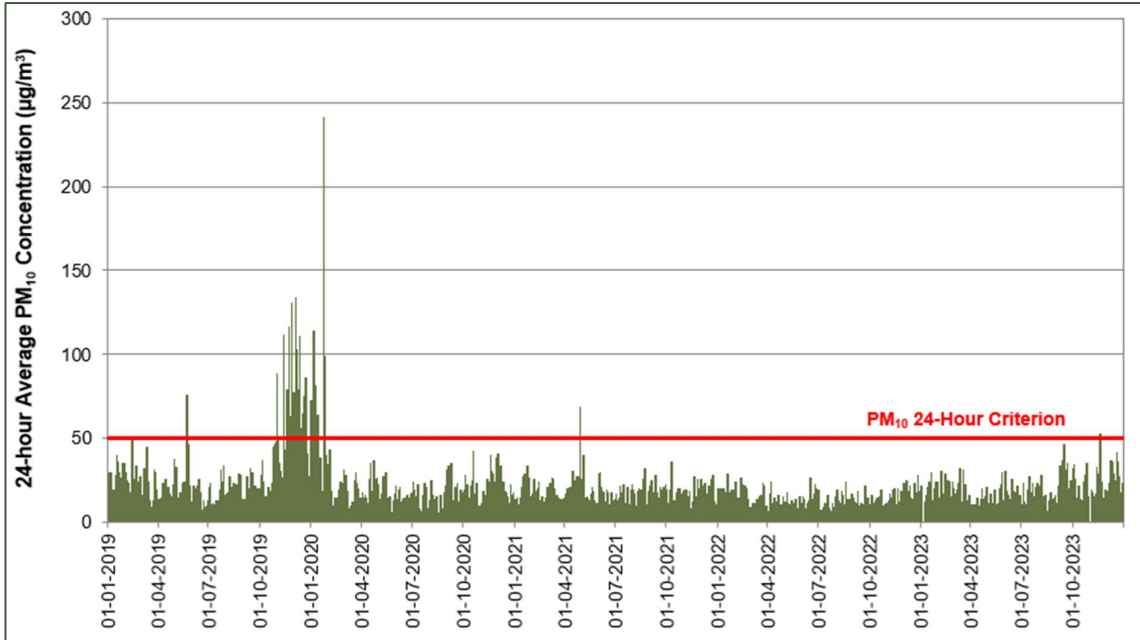
Figure 17 Measured 24-Hour Average PM 10 Concentrations at Bringelly AQMS (2019-2023)
