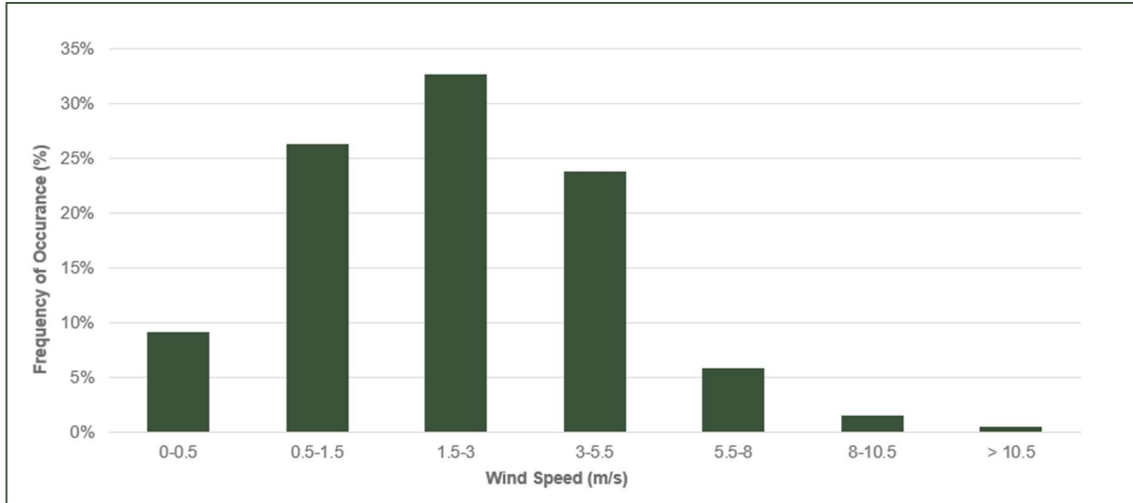
Figure 12 Wind Speed Frequency Chart for Badgerys Creek AWS – 2019-2023
