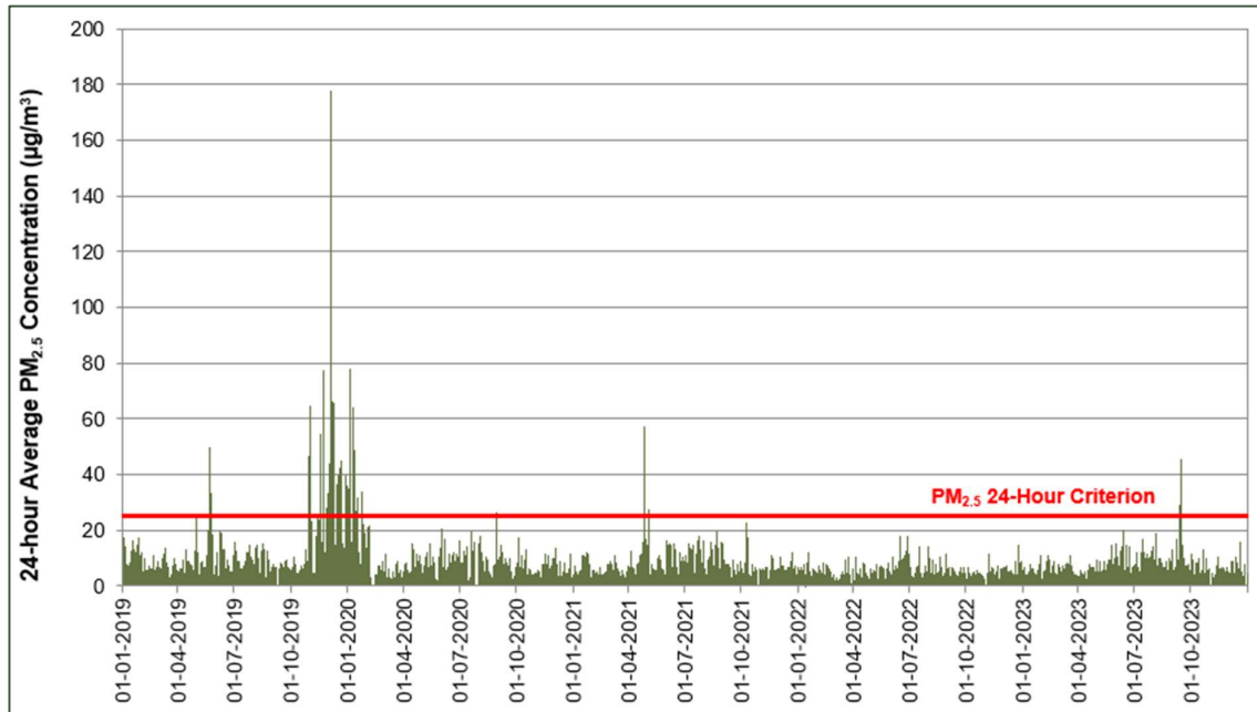
Figure 18 Measured 24-Hour Average PM 2.5 Concentrations at Bringelly AQMS (2019-2023)
