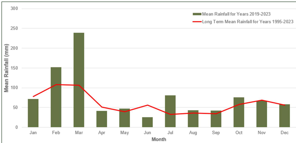
Figure 13 Long term Mean Rainfall for Badgerys Creek AWS – 1995 to 2023
