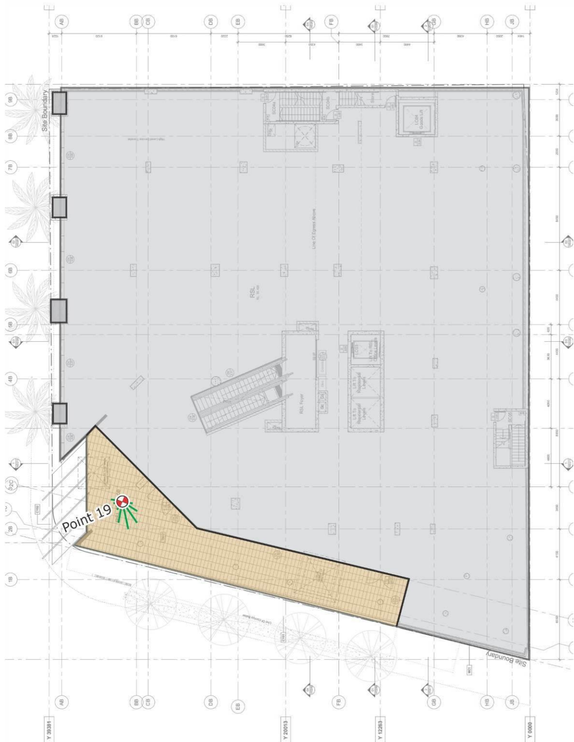
Figure 6c: Wind Direction Plots – 157 Redfern Street - Level 02 (results shown without treatments applied)
