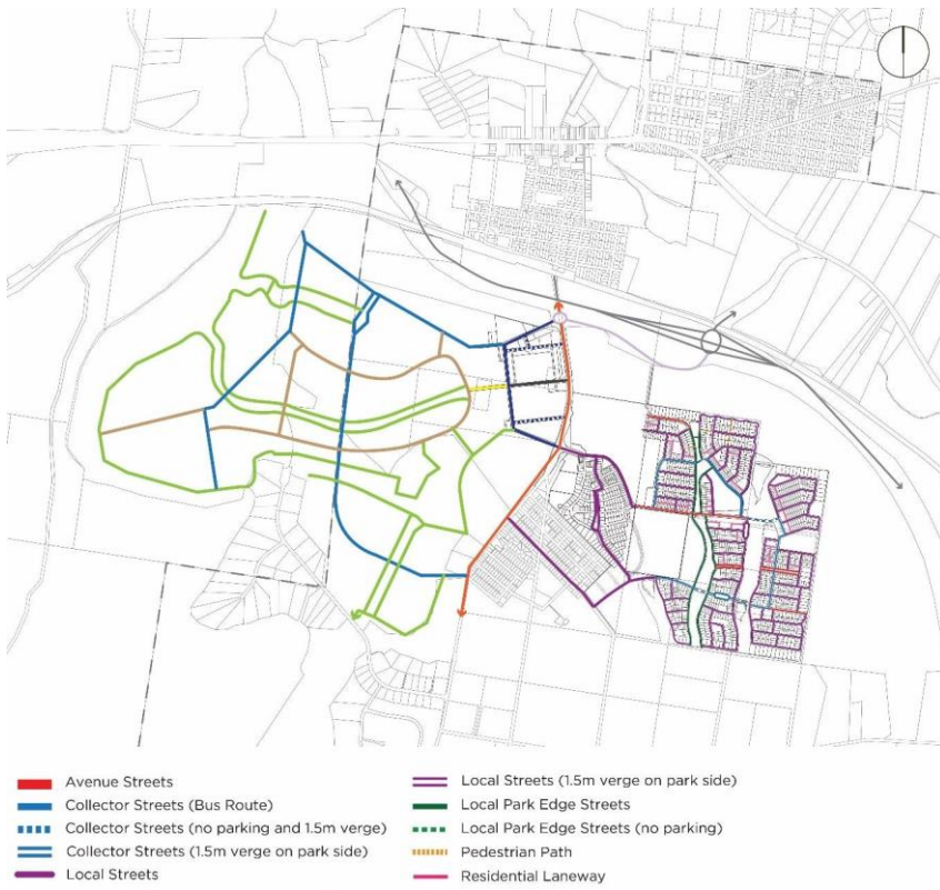
Figure 5: Overall road network and hierarchy
