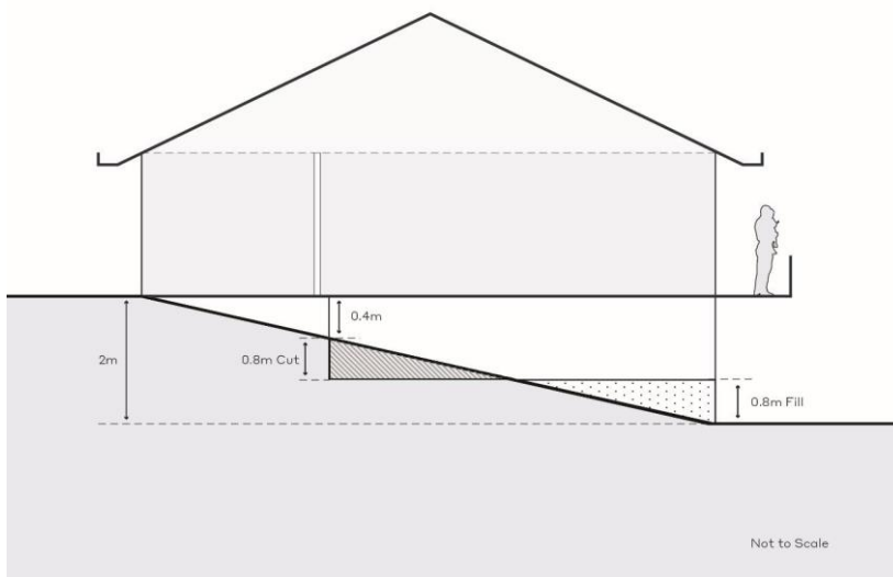
Figure 26: Sample cut and fill within residential lots
