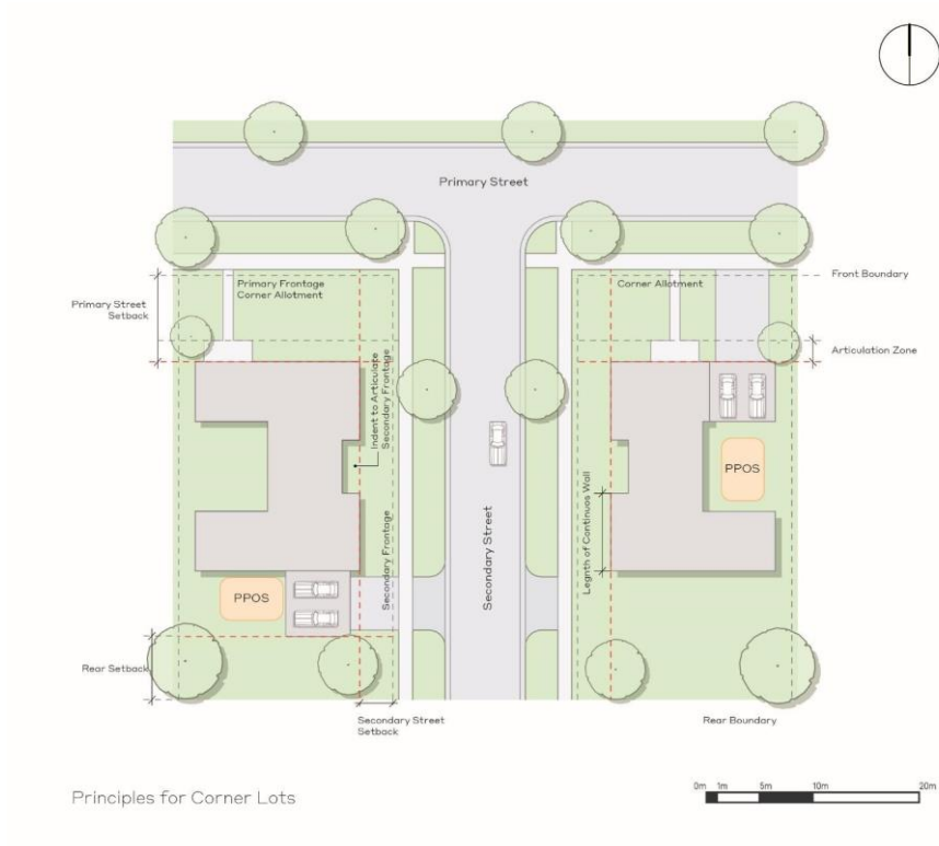
Figure 25: Principles for corner lots
