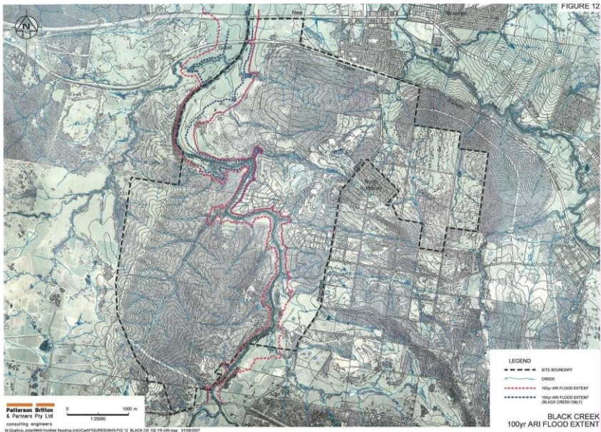
Figure 47: Black Creek 100 year ARI flood extent
