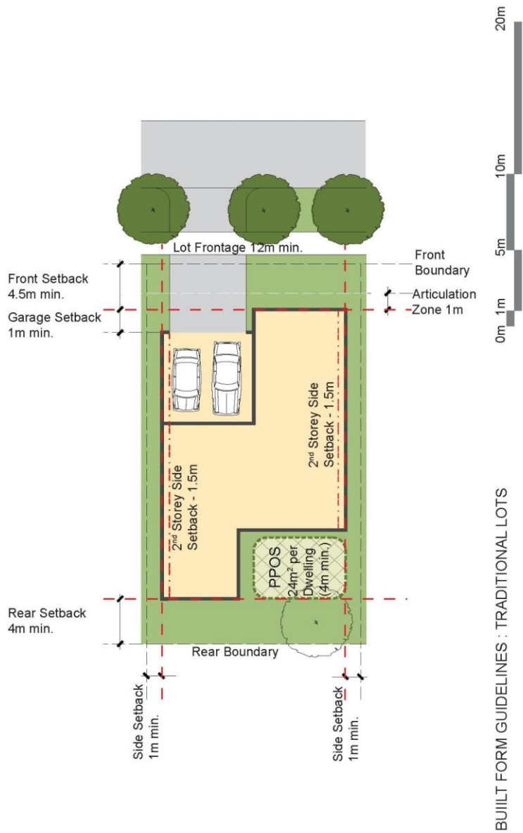
Figure 30: Indicative layout for traditional lot (detached dwelling)
