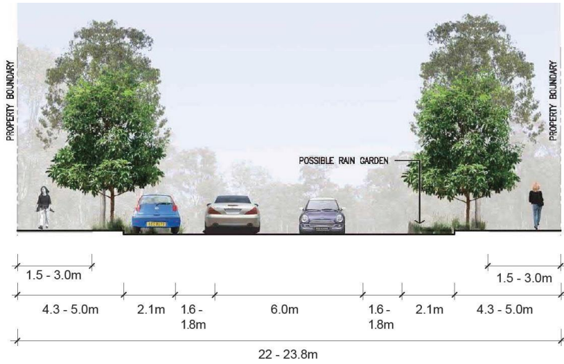
Main Street Type 2 (West)
