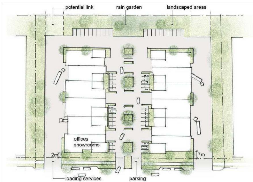
Figure 43: Typical building layout for light industrial area
