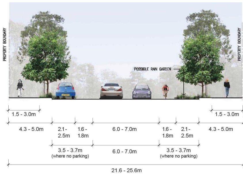
Town Centre Link Road
