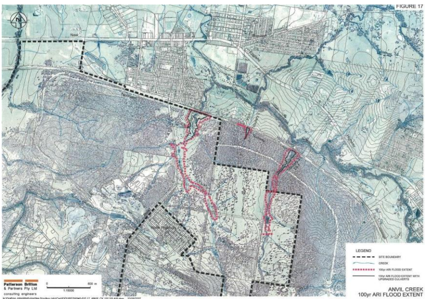
Figure 48: Anvil Creek 100 year ARI flood extent
