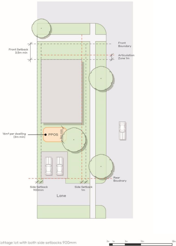
Figure 29: Indicative layout for a cottage lot dwelling (rear loaded)
