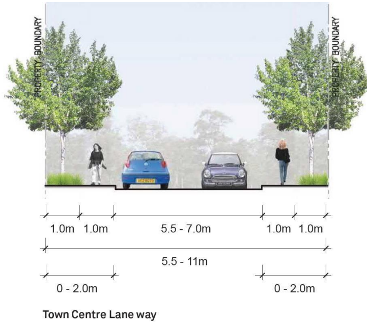
Figure 13: Town Centre Laneway
