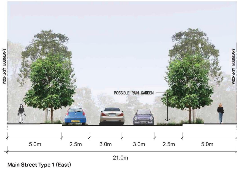
Figure 9: Main Street Type 1 (East)
