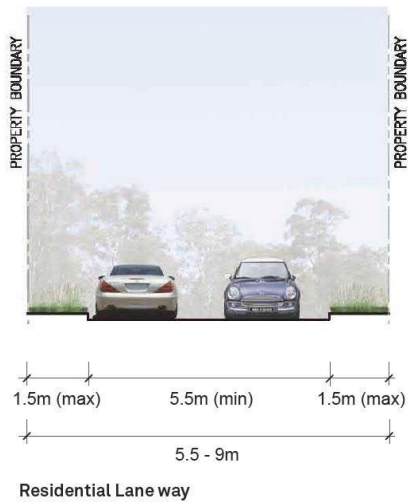
Residential Lane way
