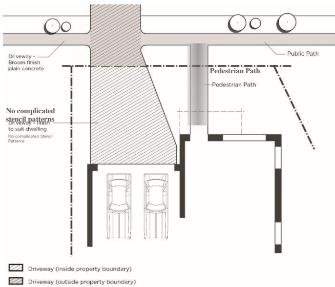
Figure 33: Driveway crossing requirements
