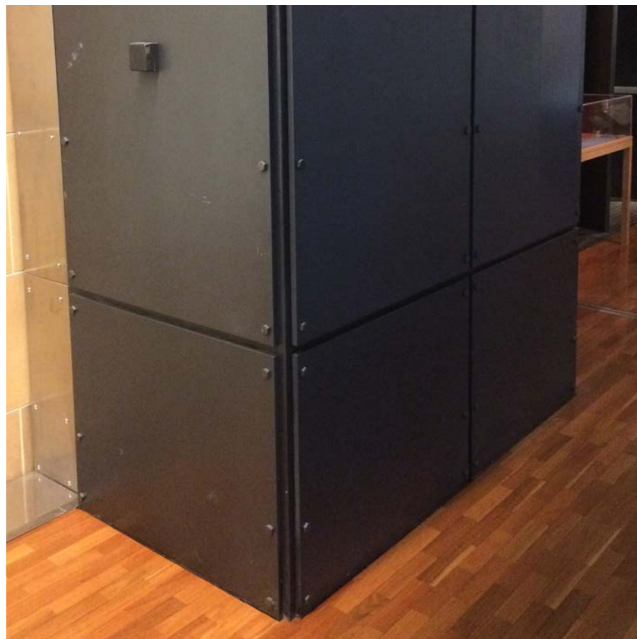
MP1 Express jointed metal bonded marine grade plywood/ cfc panels finished with MIO paint
