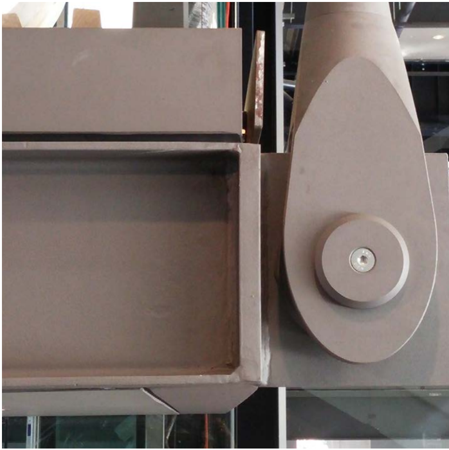
New steel structure: columns, beams Finished with warm grey MIO paint
