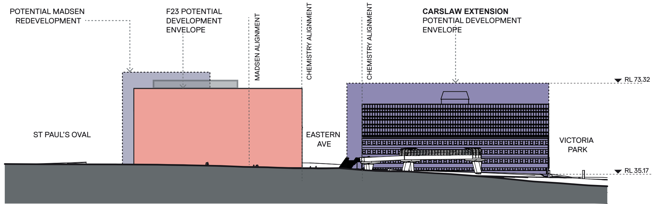
CITY ROAD ELEVATION
