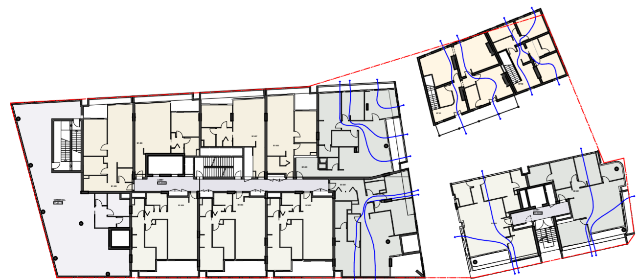
4 PLAN Level 4 1:500
