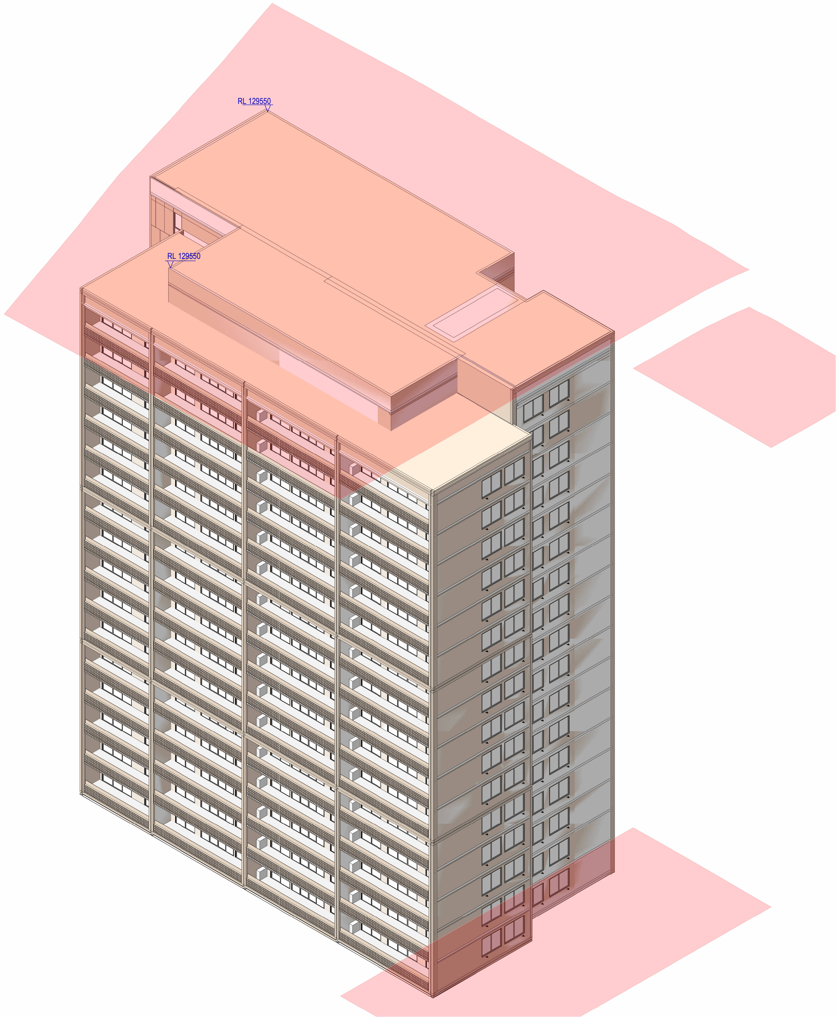
2 Height Plane Control Overlay - B2 View 02
