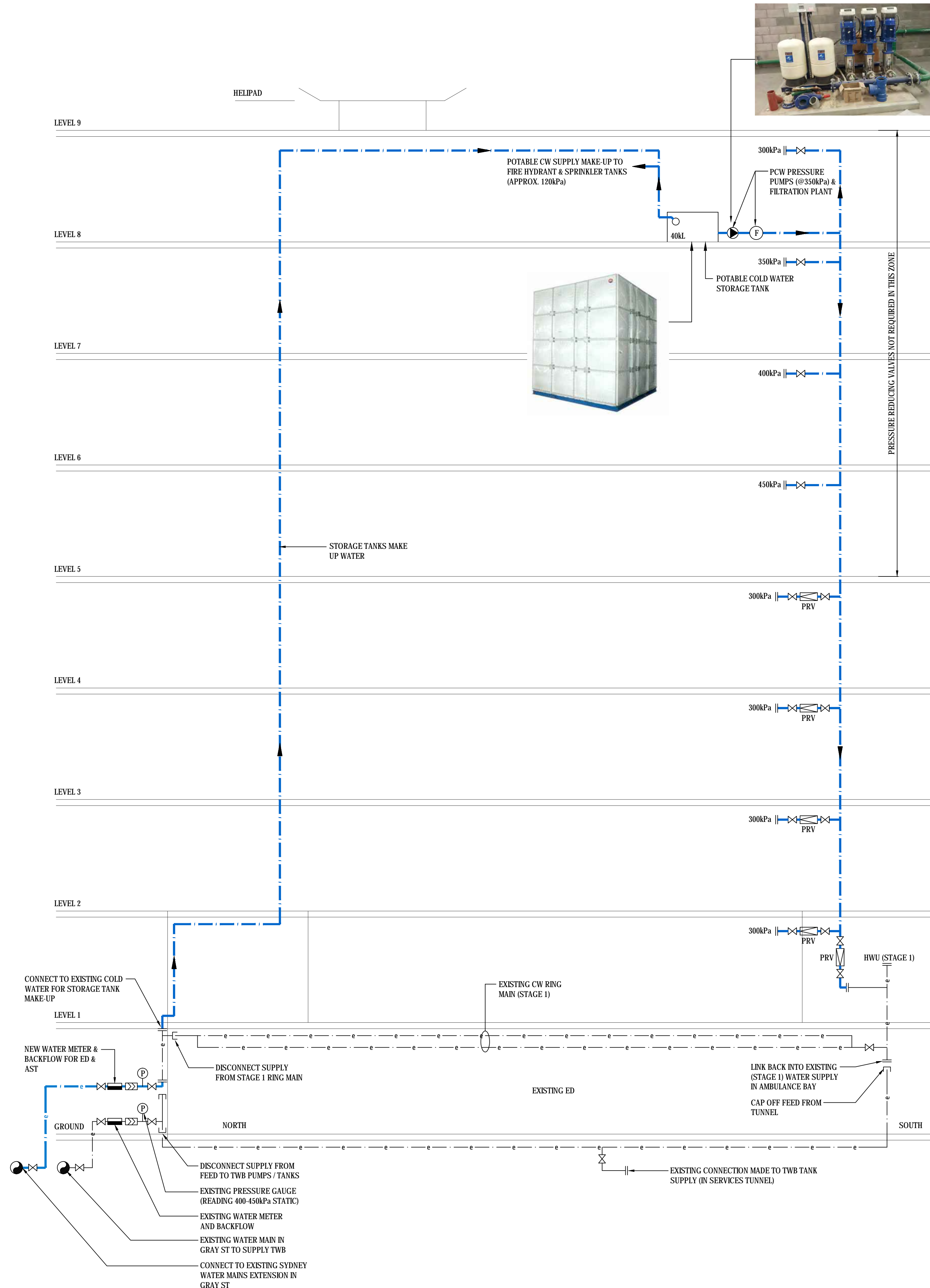
COLD WATER SCHEMATIC
