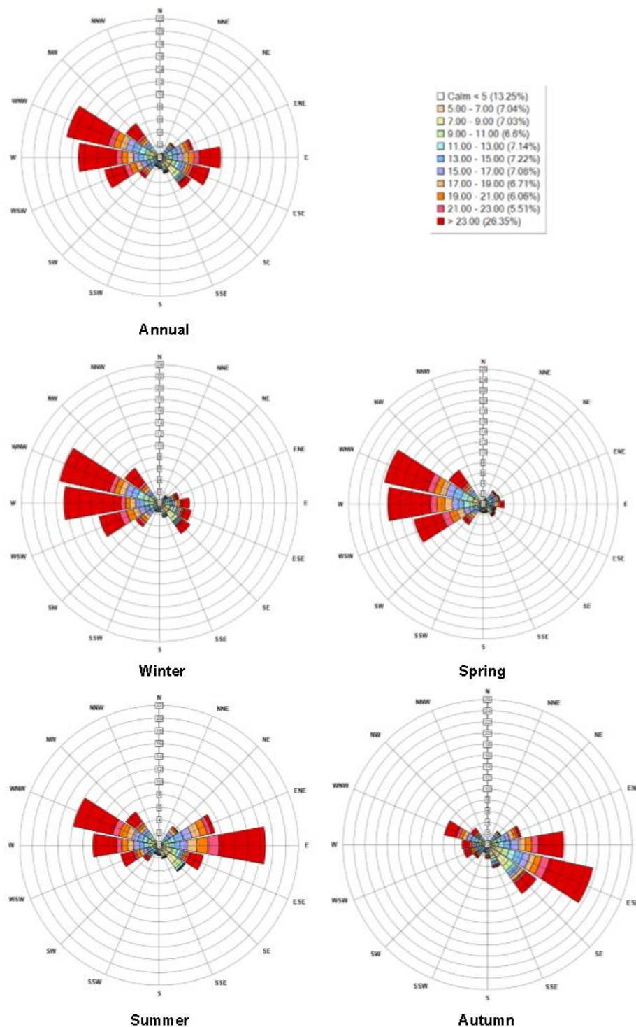
Figure 10 – Annual and Seasonal Wind roses for Borg Manufacturing (June 2016 – May 2017)
