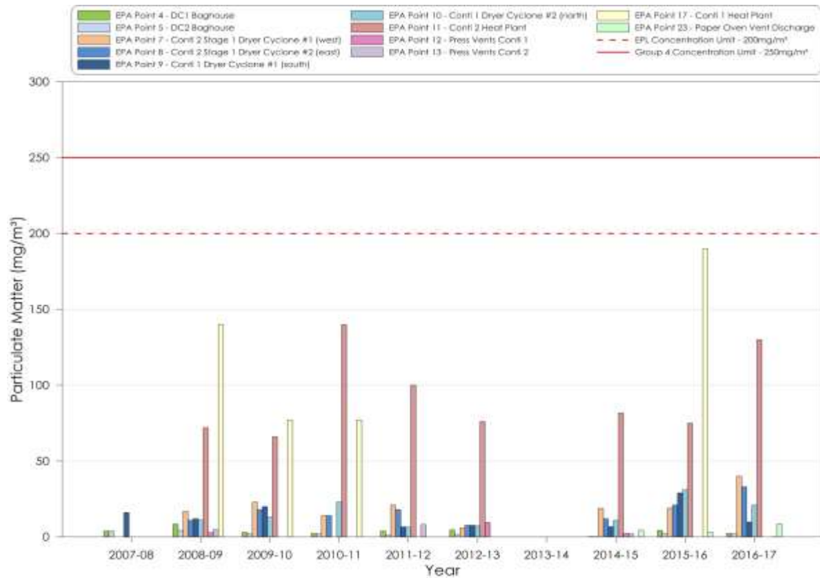
Figure 3 – Total Suspended Particulate Matter (TSP) Monitoring Results
