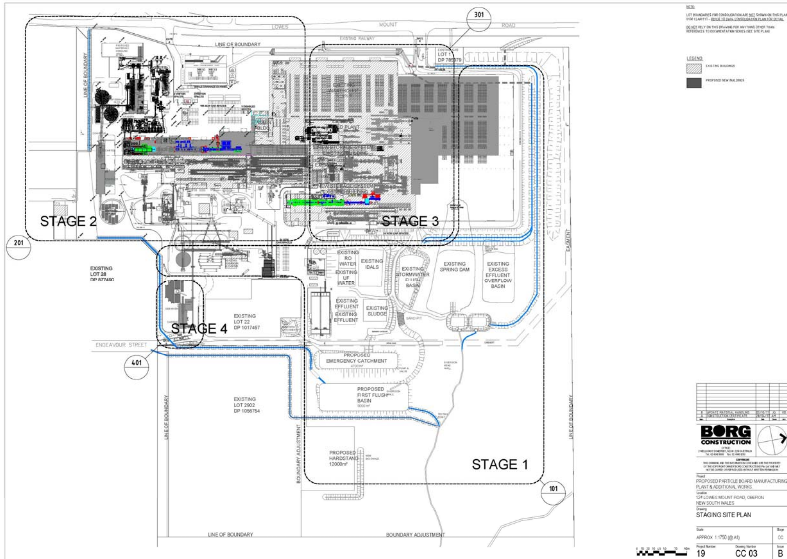
Figure 2: Staging Plan
