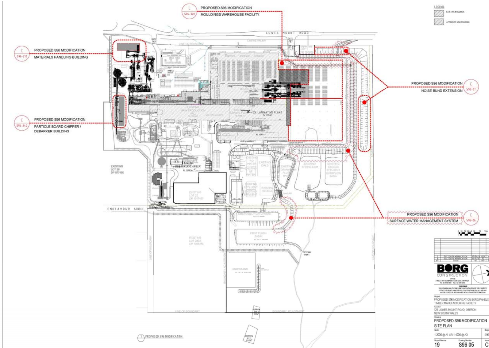
Figure 1: Site Plan
